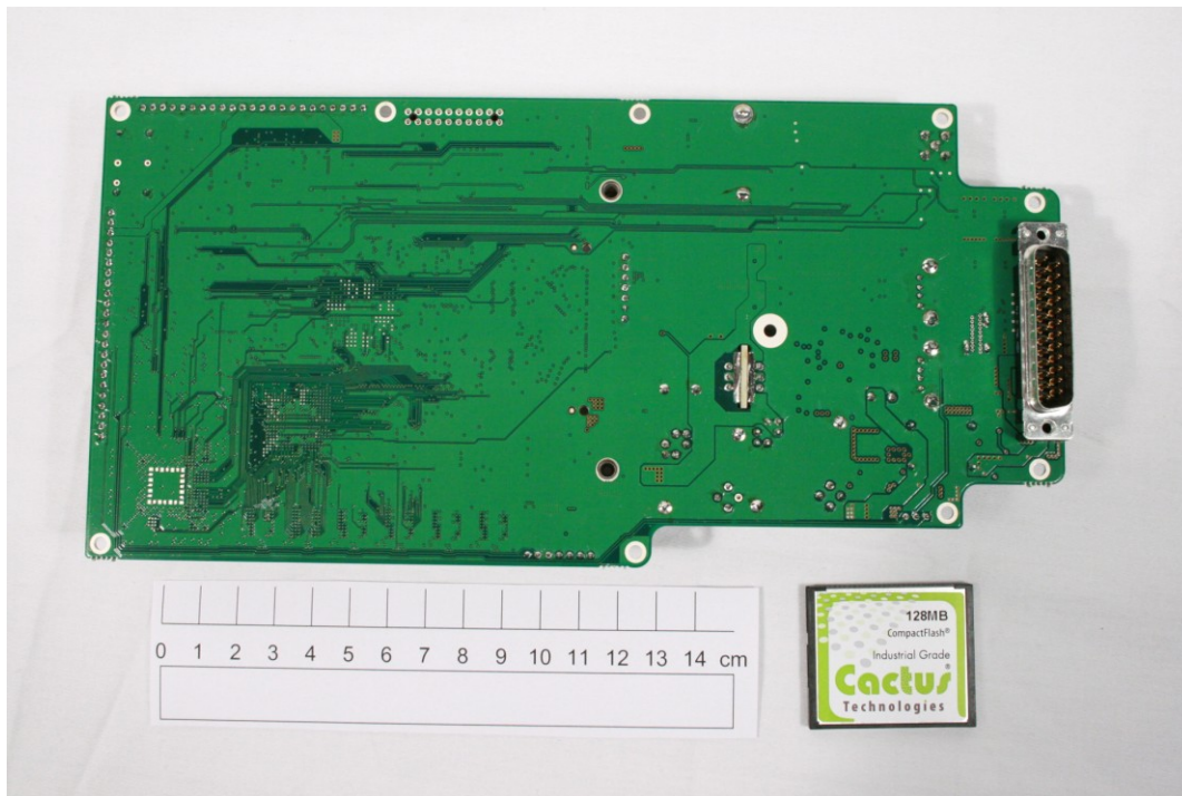
MAIN BOARD FOR BS421
