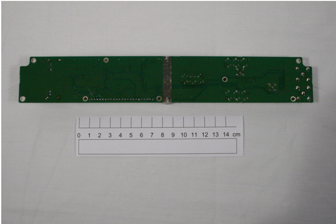
RX BOARD
