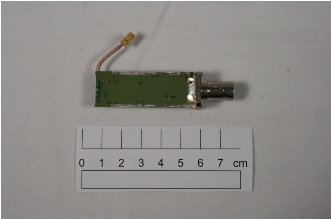
PA for TR41x 150W 850-870 MHz
