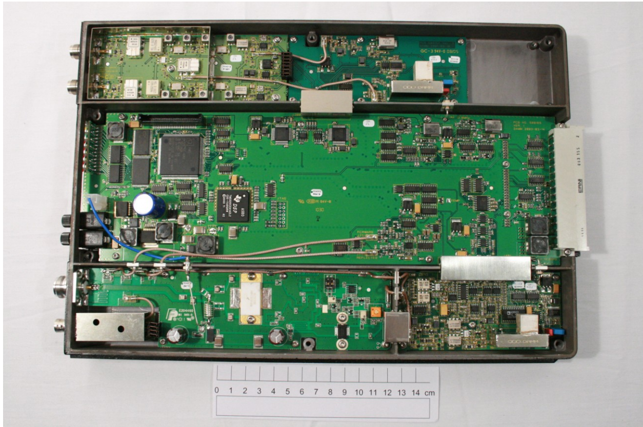
TR412H Transceiver 805-825_850-870 MHz
