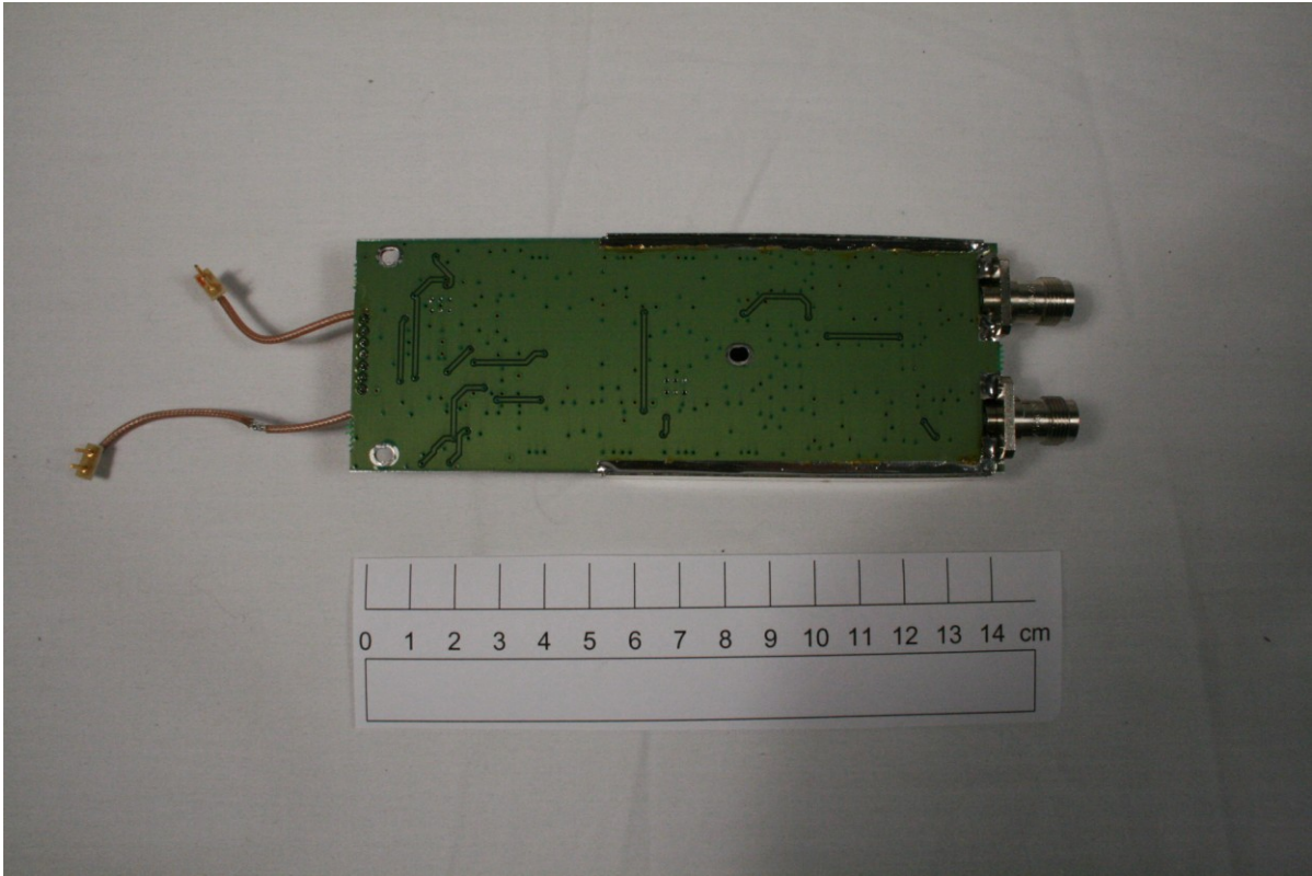
RX Synthesizer for TR41x 760-780 MHz
