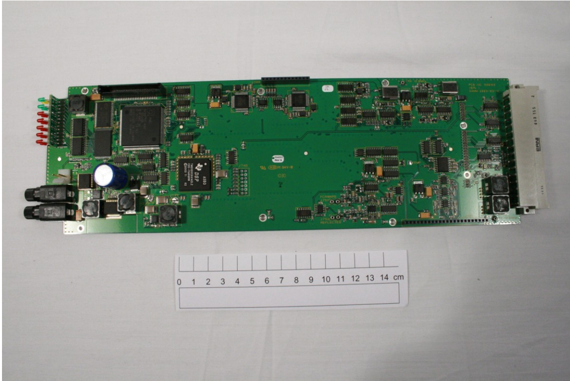
Main Board for TR412
