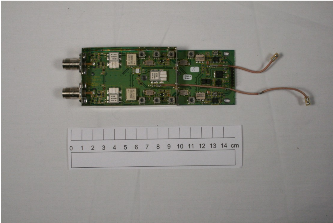
RX Front End for TR41x 805-825 MHz
