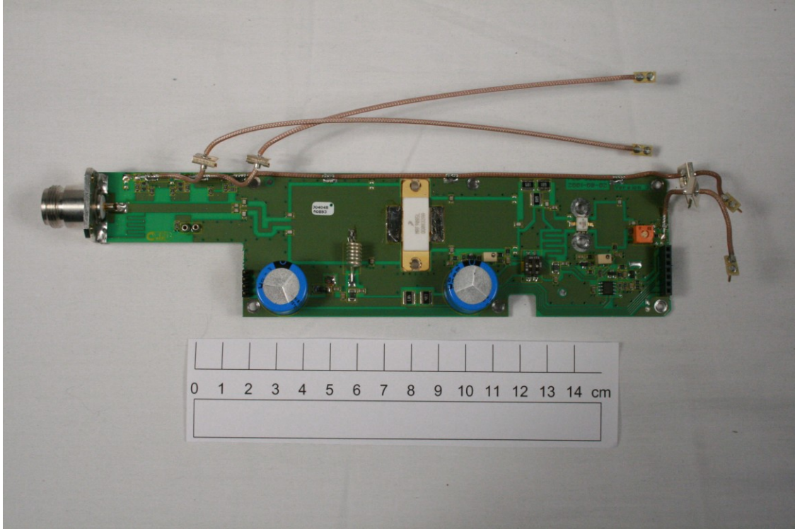
PA for TR41x 60W 850-870 MHz
