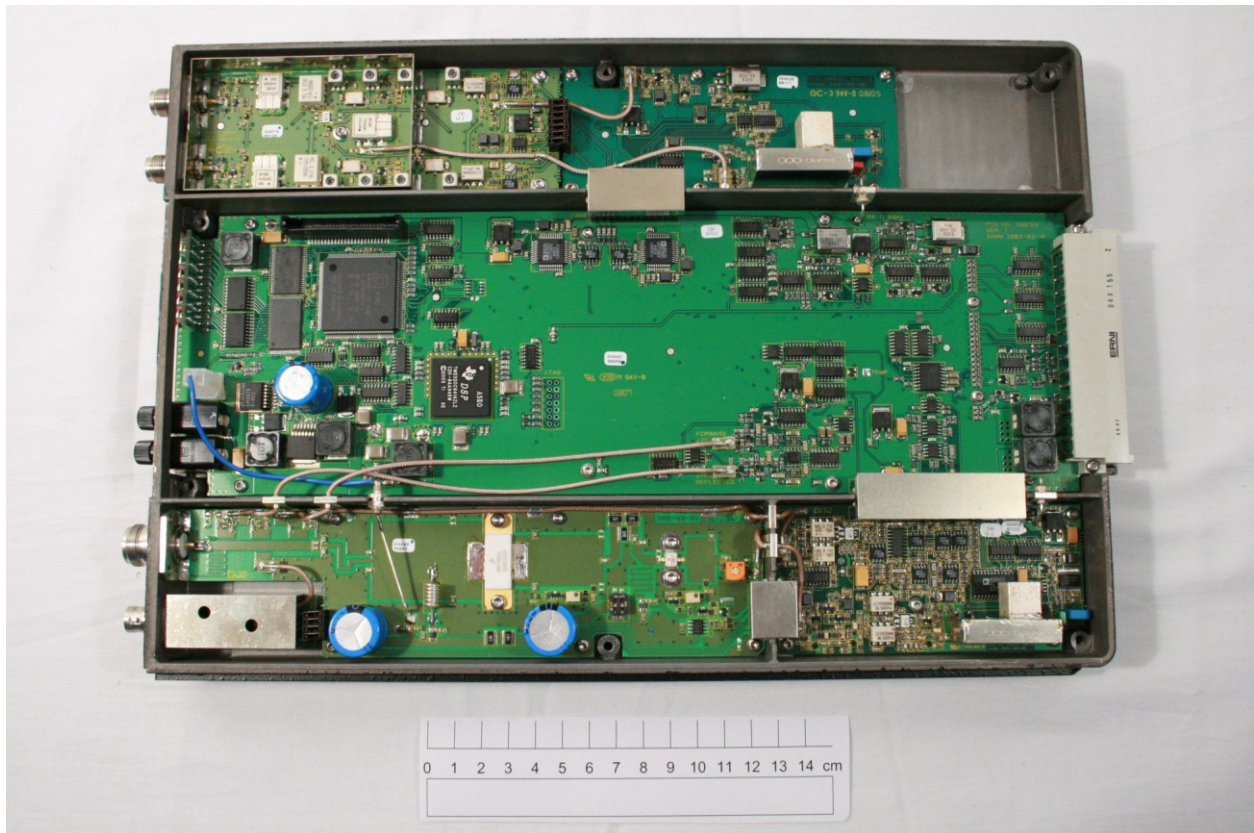
TR412 Transceiver 805-825_850-870 MHz
