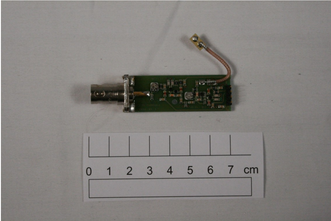
RFTL SWITCH FOR TR41x 850-960 MHz
