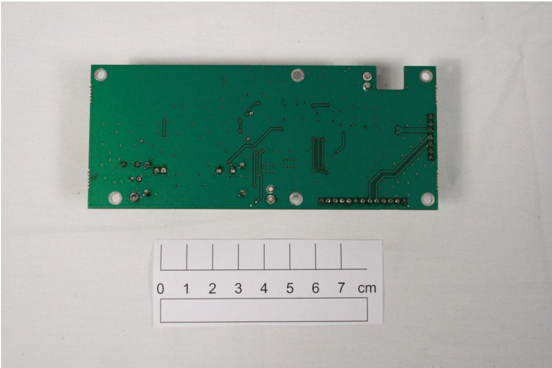
RX SYNTHESIZER
