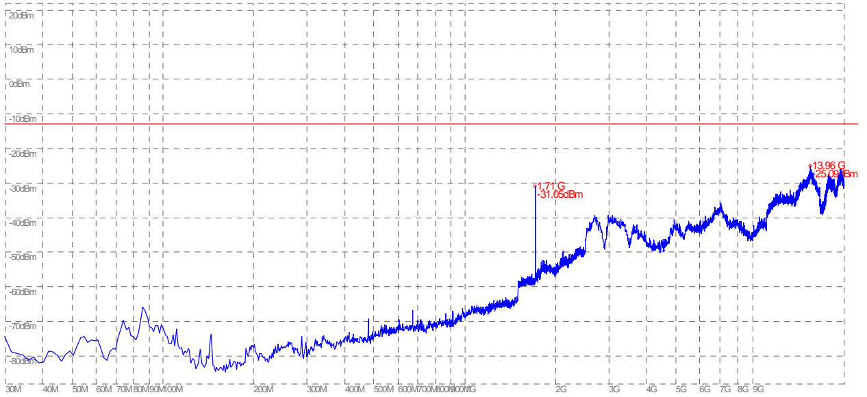
(Plot E.2: WCDMA 1700MHz Channel = 1312, Test Antenna Vertical)
