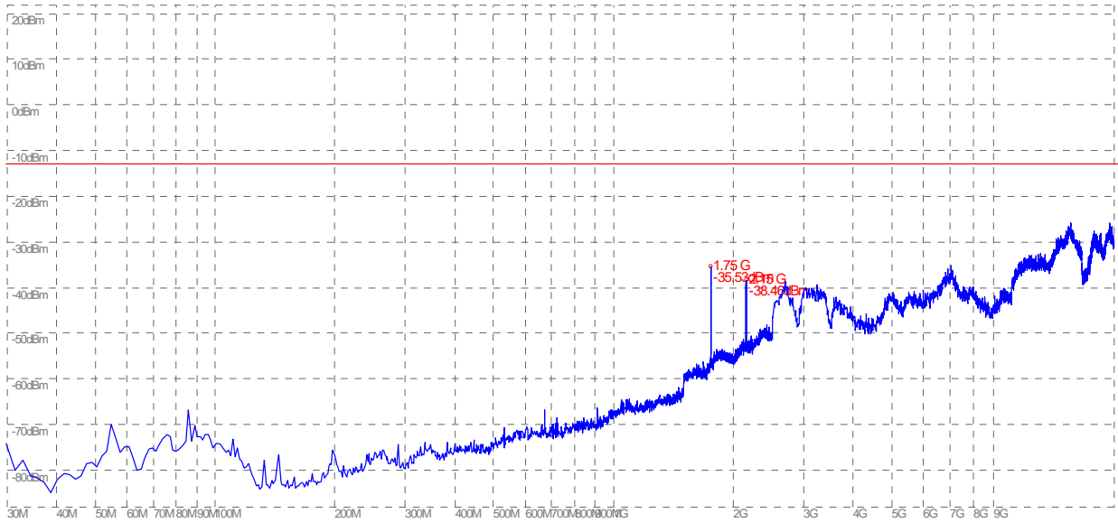
(Plot E.5: WCDMA 1700MHz Channel = 1513, Test Antenna Horizontal)
