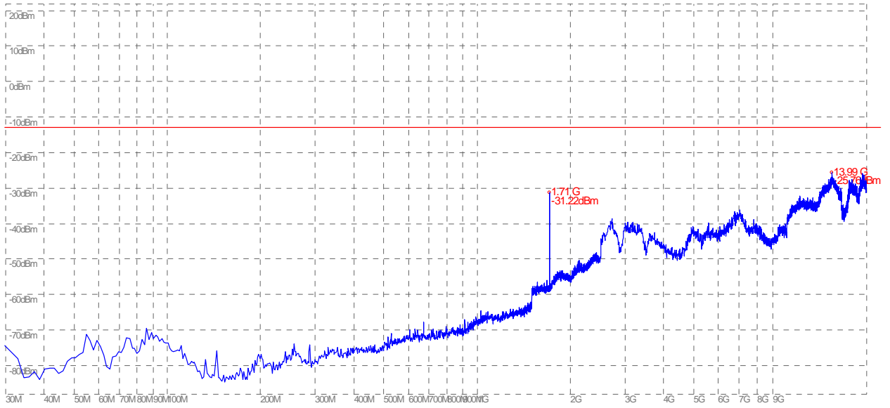
(Plot E.1: WCDMA 1700MHz Channel = 1312, Test Antenna Horizontal)
