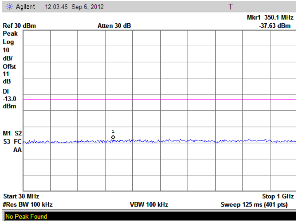
(Plot E1: WCDMA1700MHz Channel = 1312, 30MHz to 1GHz)
