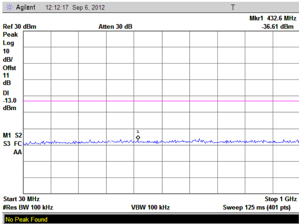
(Plot E2: WCDMA1700MHz Channel = 1412, 30MHz to 1GHz)
