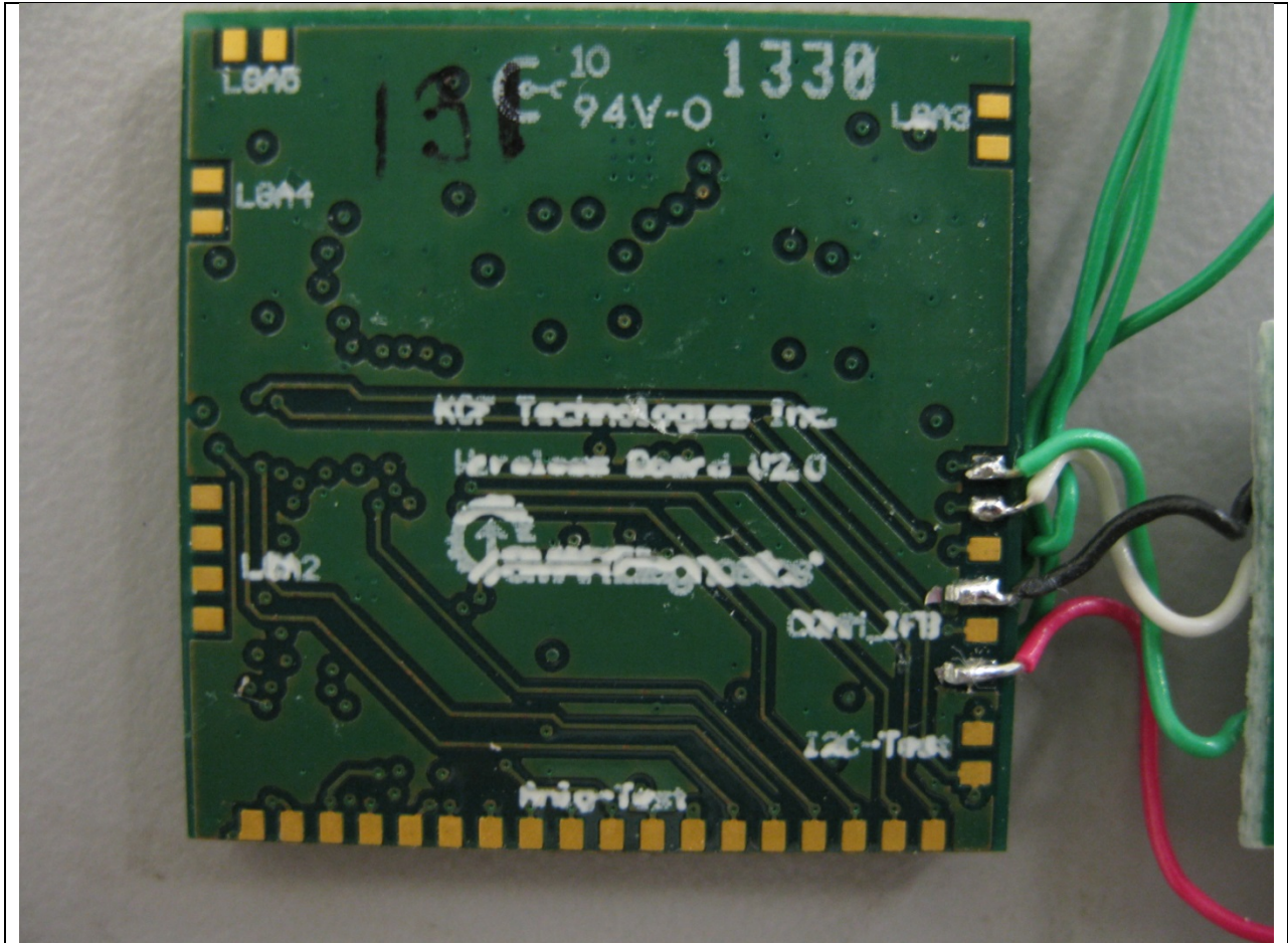
Model SD2, Bottom View (Main Board)
