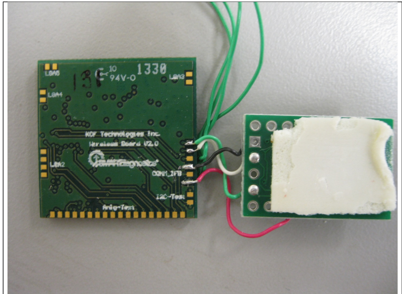
Model SD2, Bottom View (Main Board and Daughter Board)
