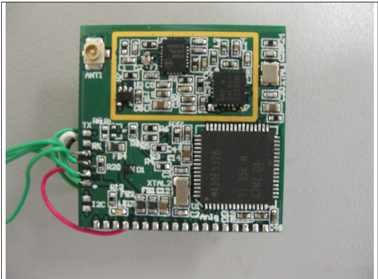
Model SD2, Top View with Shield Removed
