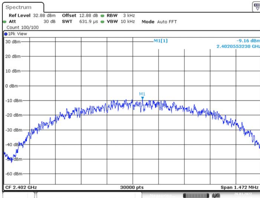
Power Spectral Density, BLE 1M Low Channel
