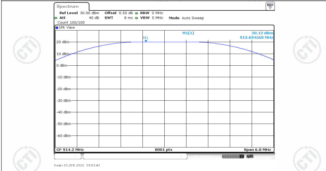
BW1523.4K_Ant1_914.2
