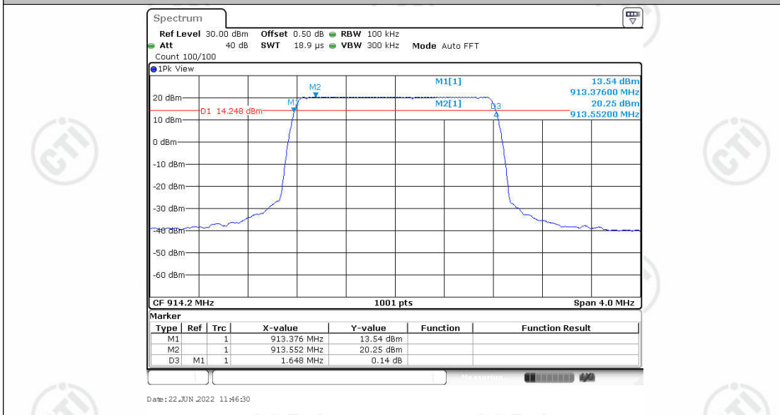
BW1523.4K_Ant1_914.2
