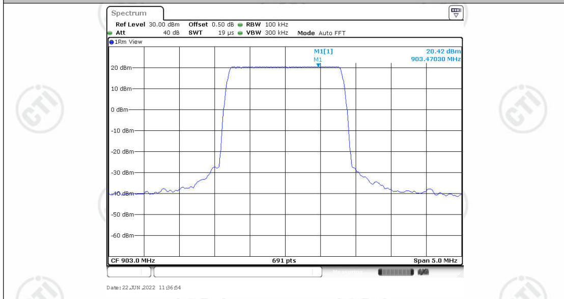
BW1523.4K_Ant1_903_0-Reference
