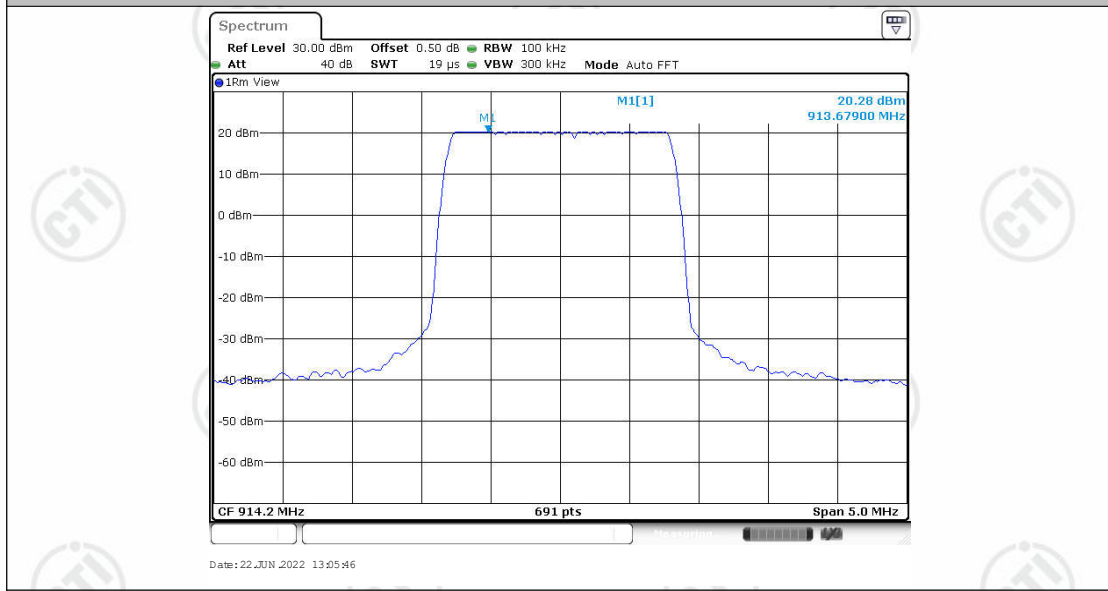
BW1523.4K_Ant1_914.2_0~Reference
