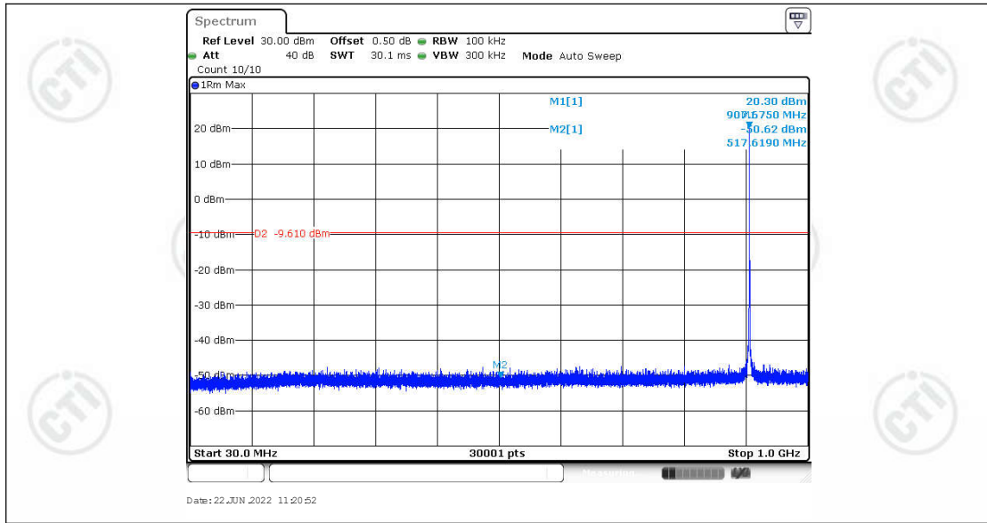
BW500K_Ant1_907.8_30~1000
