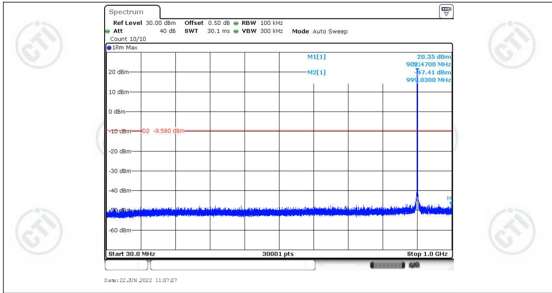
BW1523.4K_Ant1_903_30~1000
