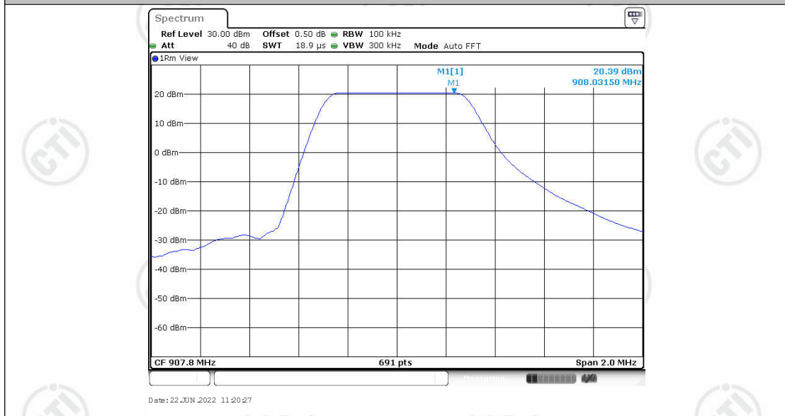
BW500K_Ant1_907.8_0~Reference
