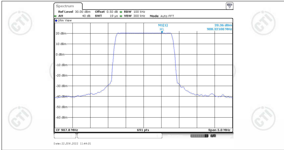
BW1523.4K_Ant1_907.8_0~Reference
