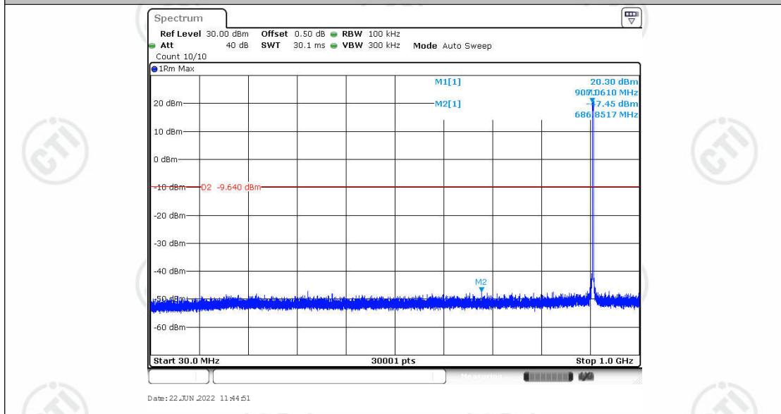
BW1523.4K_Ant1_907.8_30~1000
