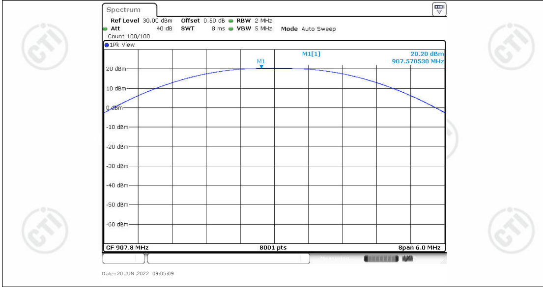
BW500K_Ant1_907.8
