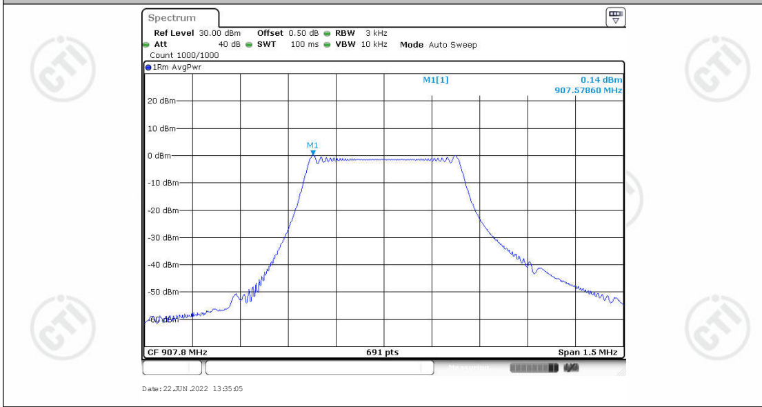
BW500K_Ant1_907.8
