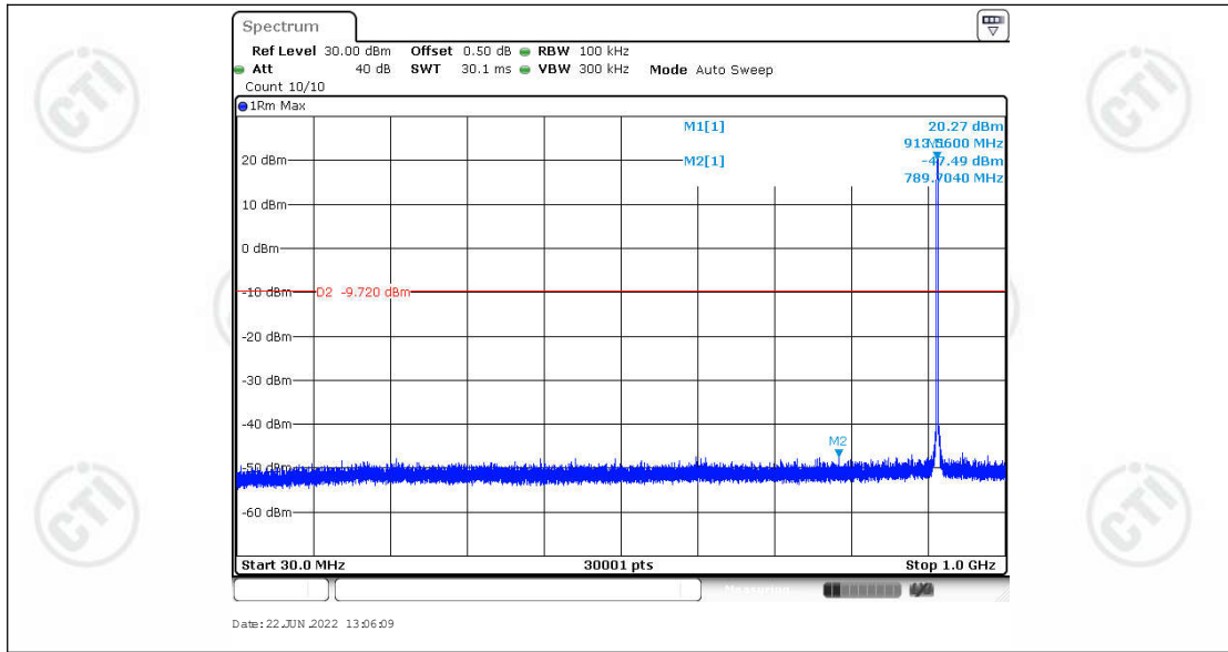
BW1523.4K_Ant1_914.2_30~1000
