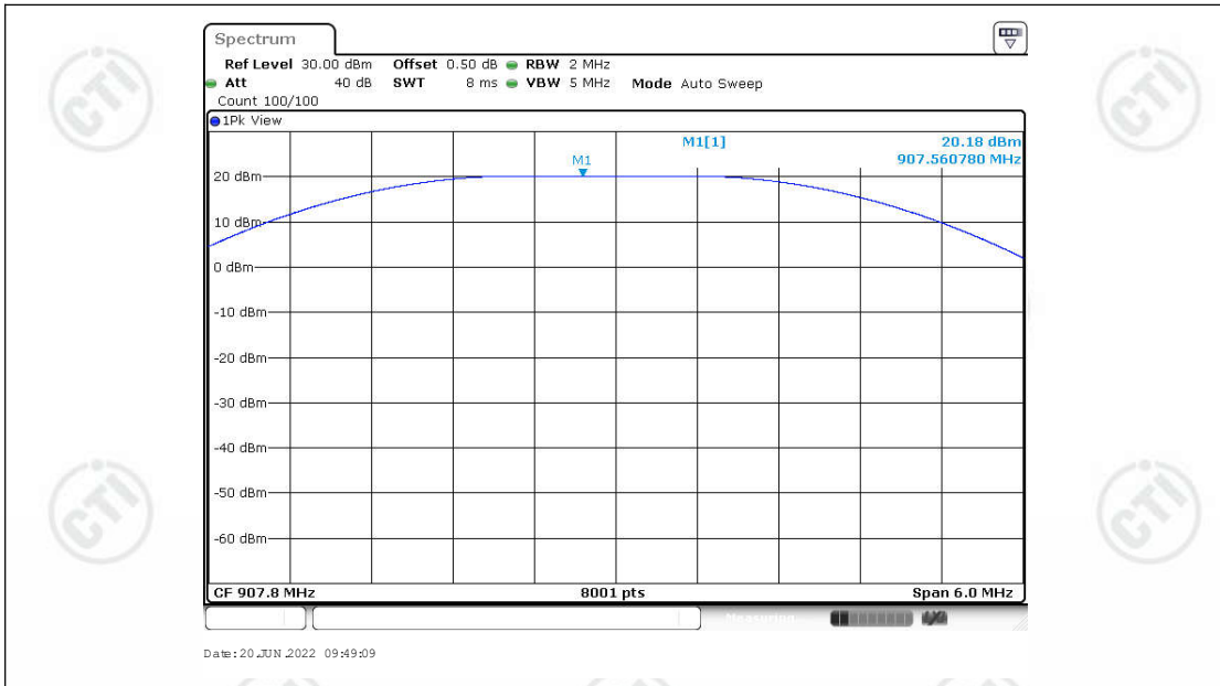
BW1523.4K_Ant1_907.8
