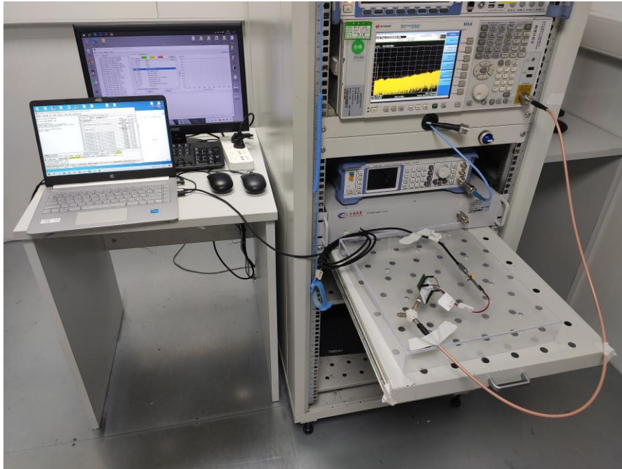
Conducted Test-LoRa-DTS
