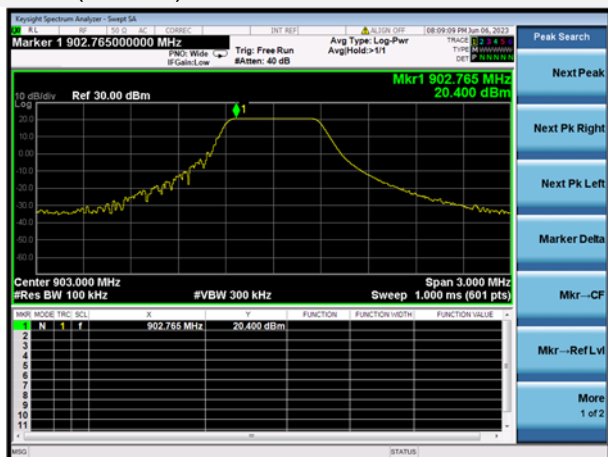
LoRa (500kHz) LOW CHANNEL, CARRIER LEVEL
