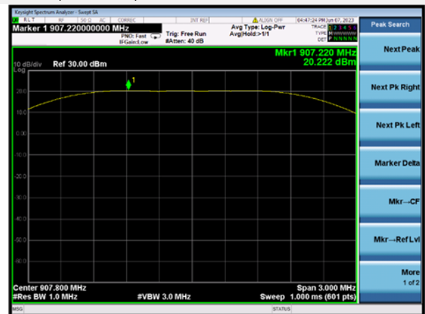
LoRa (1523kHz) MIDDLE CHANNEL
