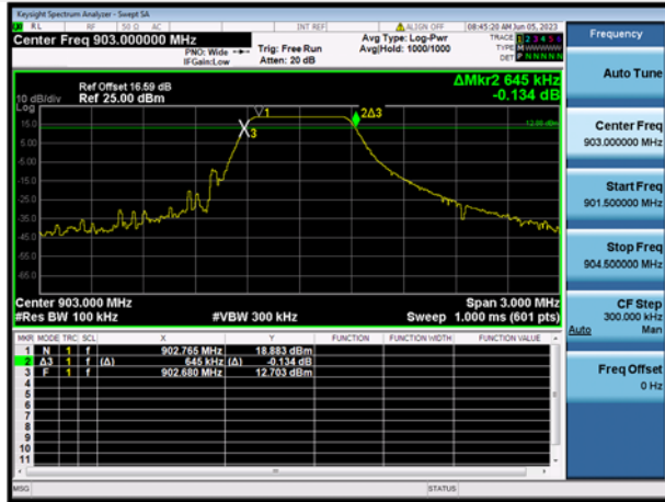
LoRa (500kHz) LOW CHANNEL
