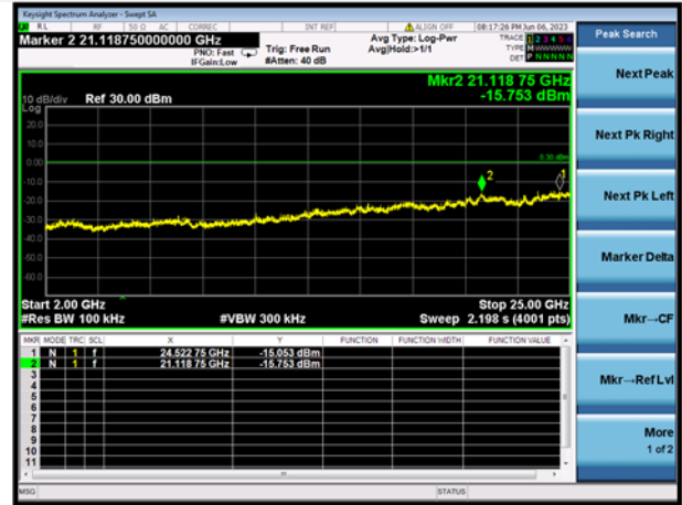
LoRa (500kHz) MIDDLE CHANNEL, SPURIOUS 2 GHz ~ 25 GHz
