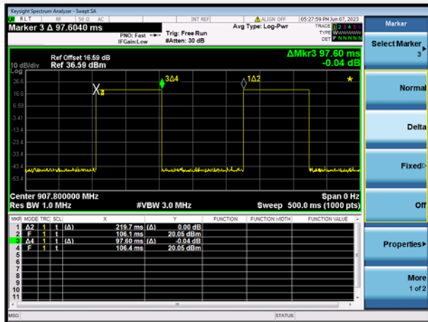
LoRa (1523kHz)
