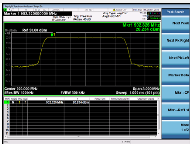
LoRa (1523kHz) LOW CHANNEL, CARRIER LEVEL
