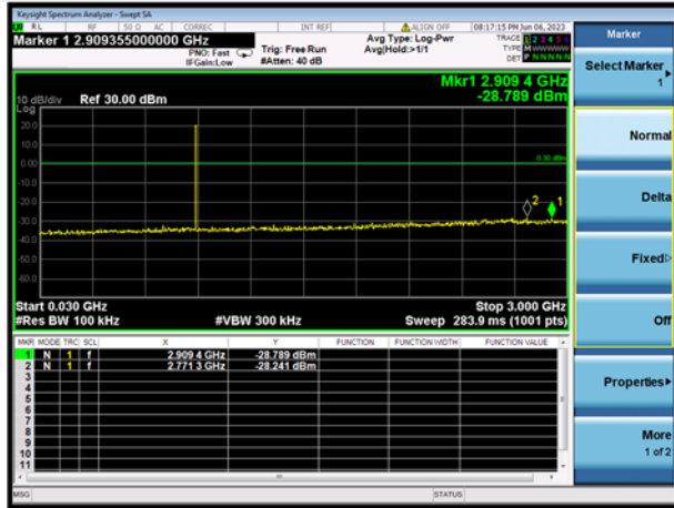
LoRa (500kHz) MIDDLE CHANNEL, SPURIOUS 30 MHz ~ 3 GHz
