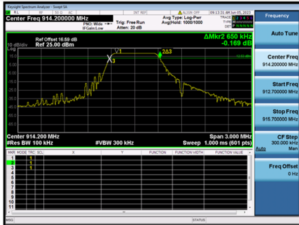
LoRa (500kHz) HIGH CHANNEL
