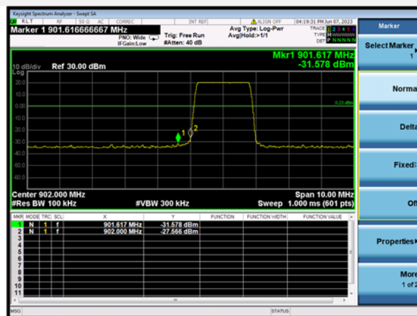
LoRa (1523kHz) LOW CHANNEL, BAND EDGE
