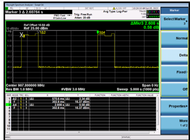
LoRa (1523kHz)
