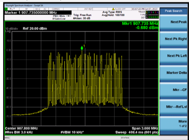
LoRa (1523kHz) MIDDLE CHANNEL
