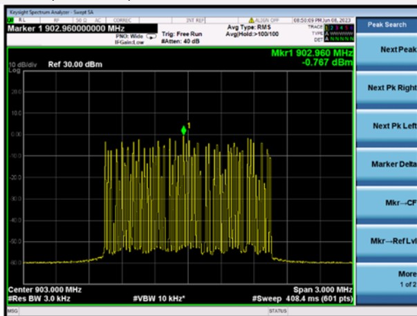
LoRa (1523kHz) LOW CHANNEL
