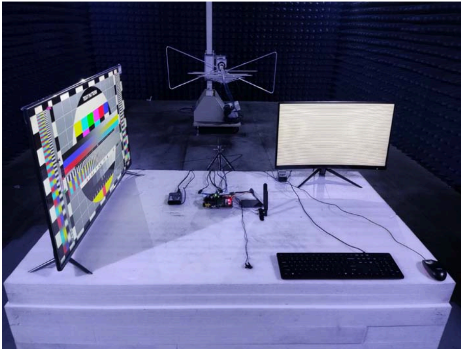
Photo of Radiated Emission Measurement (Below 1G) Adapter 1: HA-1600-12
