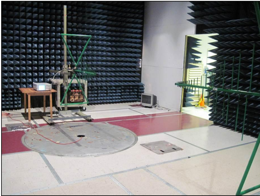
Photograph 4. ERP, Test Setup
