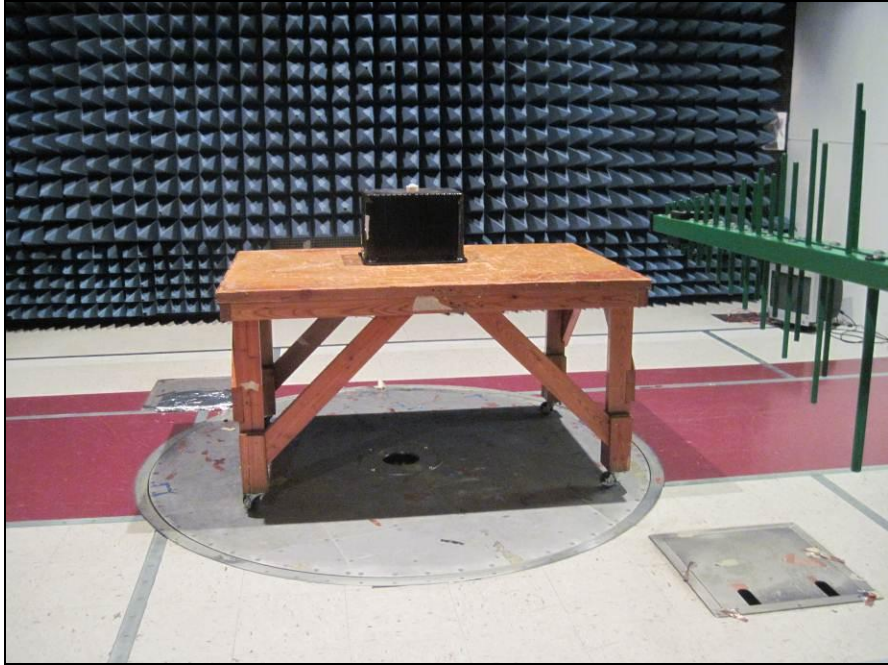
Photograph 5. Radiated Bilog
