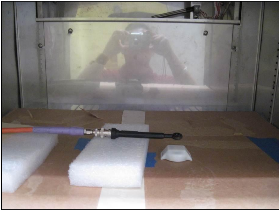
Photograph 10. Frequency Stability, Test Chamber
