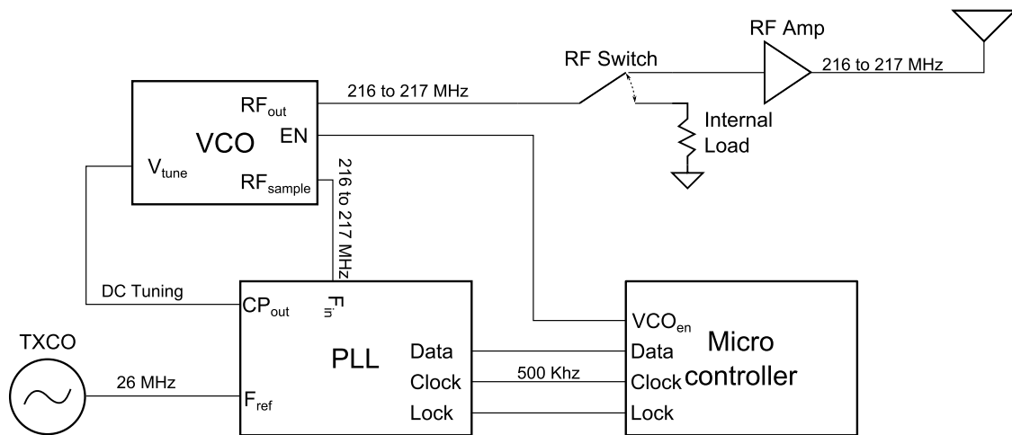
Figure 1 - Block Diagram of PLD-010
