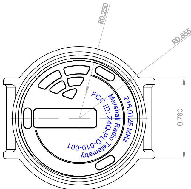
Figure 1 - Engineering Drawing of Label Location Inside Device
