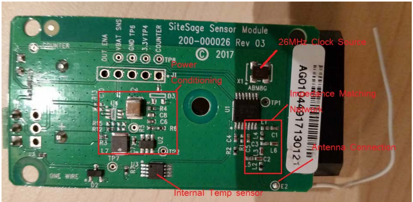
Fig . 13 Assmled sensor, with batteries
