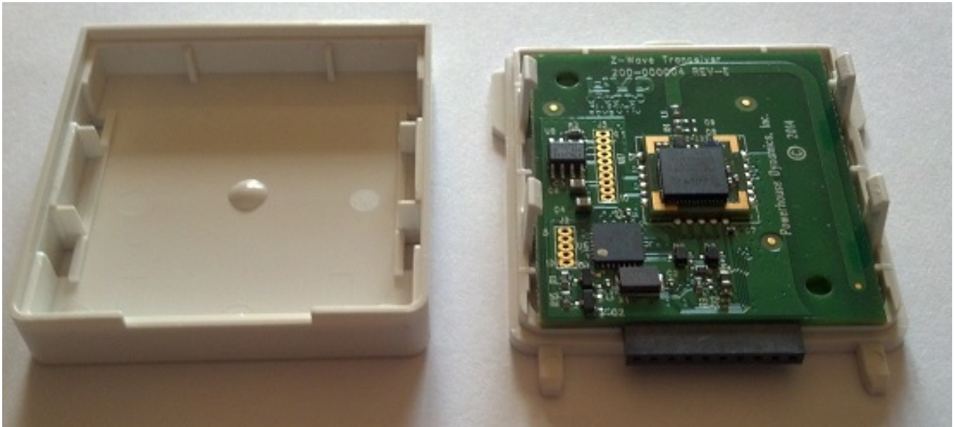
Z-Wave Module Assembly – ZM4102 chip assembly situated in the middle of the PCB, antenna running from top of PCB down right hand side. Host connection at the bottom.
