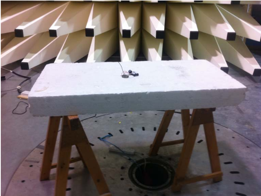
Figure 1: Test Configuration
