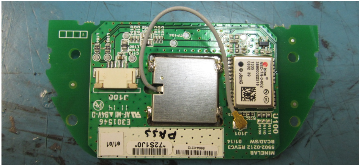
Figure 1. GPS Module
