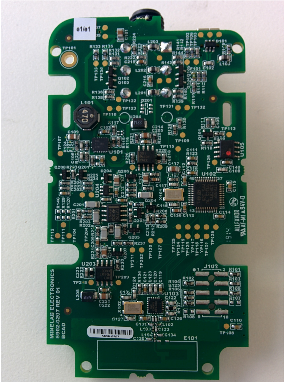
Figure 2. WM12 module, showing PCB antenna (bottom)
