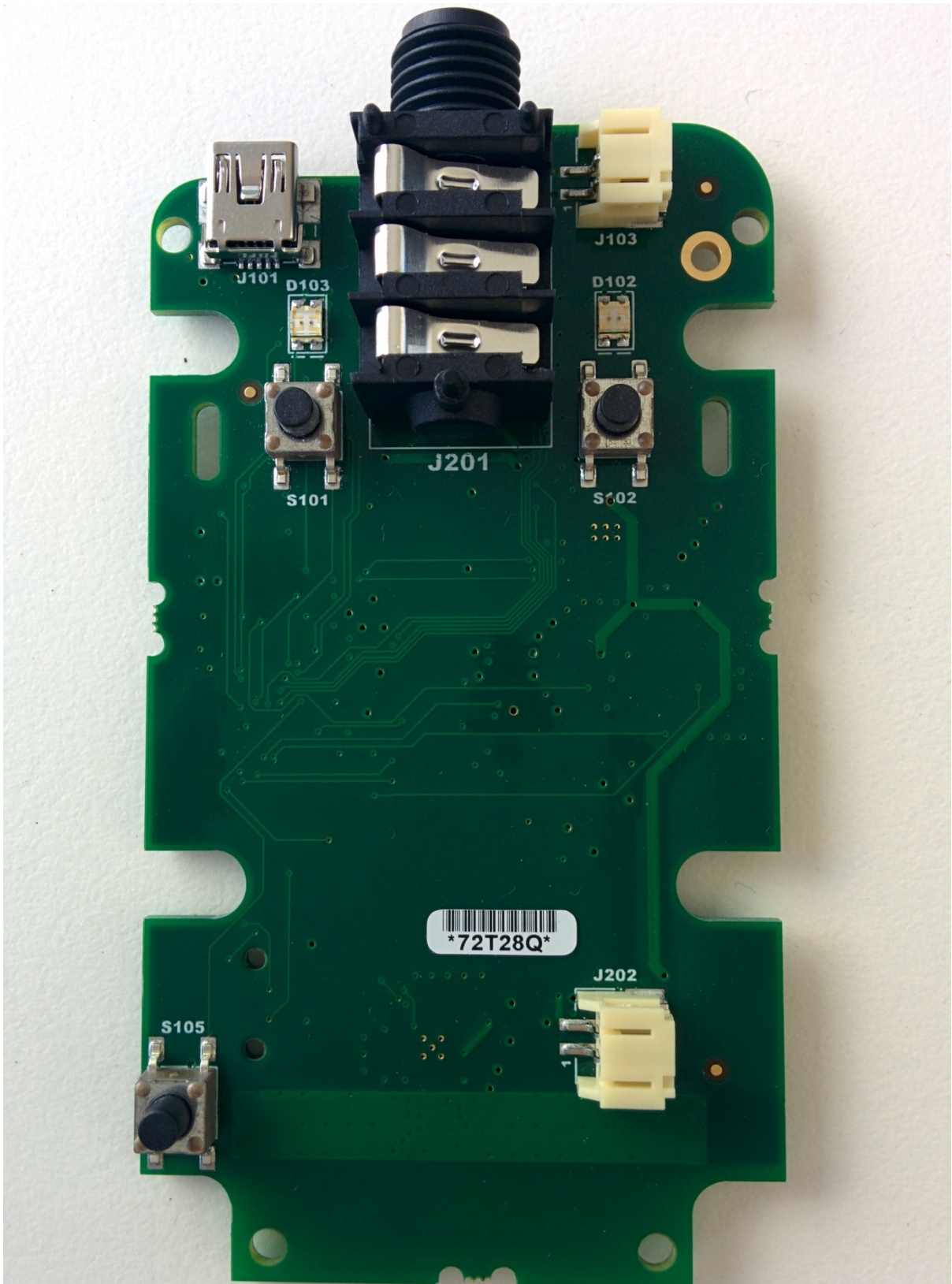
Figure 3. WM12 module, top-side
