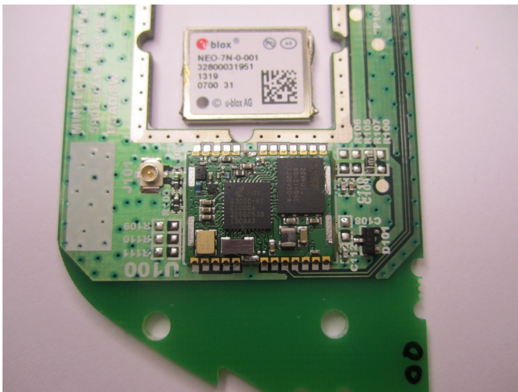
Figure 1a. GPS Receiver with can removed
