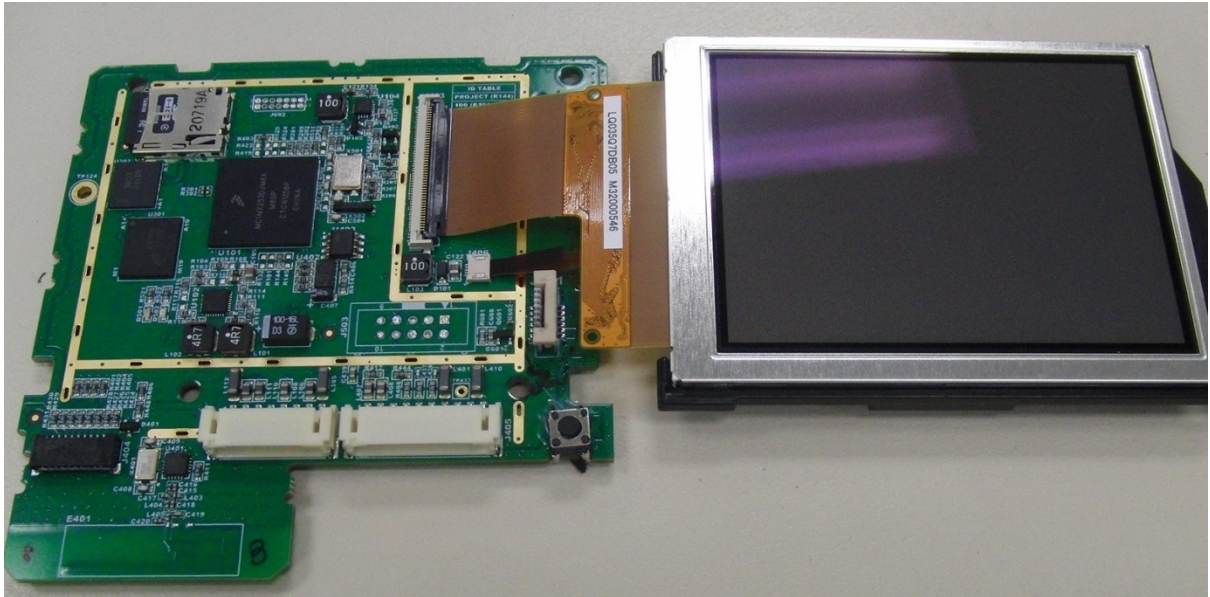
Figure 3. User Interface Pod with screen moved aside and shield removed
