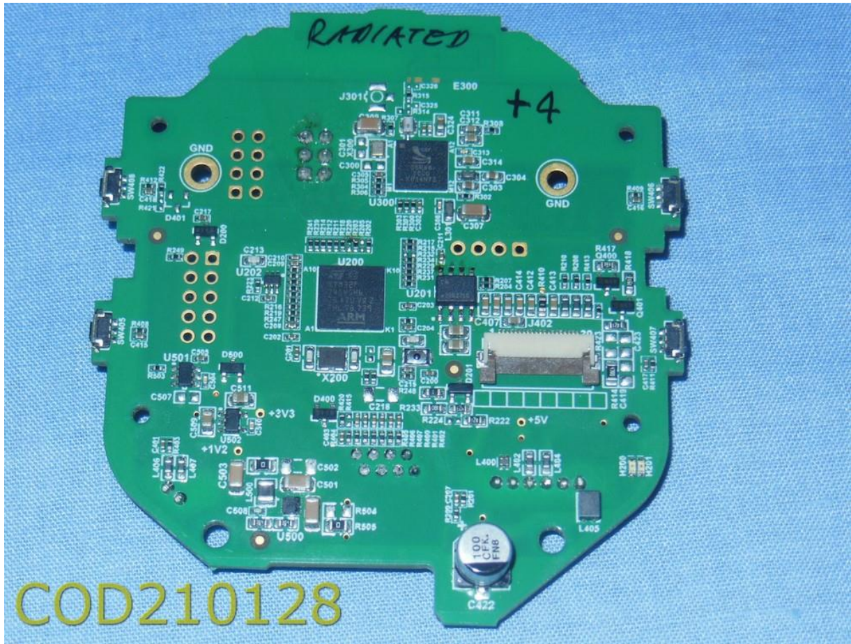
View Radiated PCB Side 2
