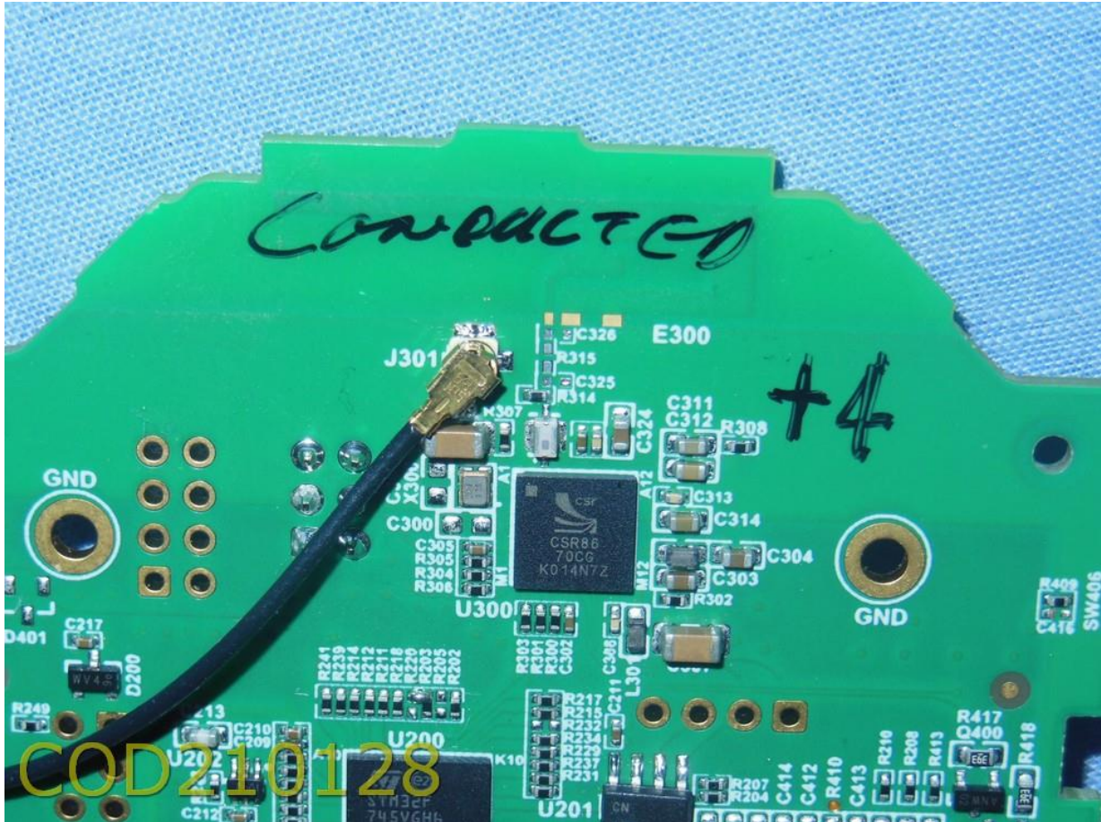
View RF Conducted PCB Side 2, Showing Addition Of Antenna Port Connection
