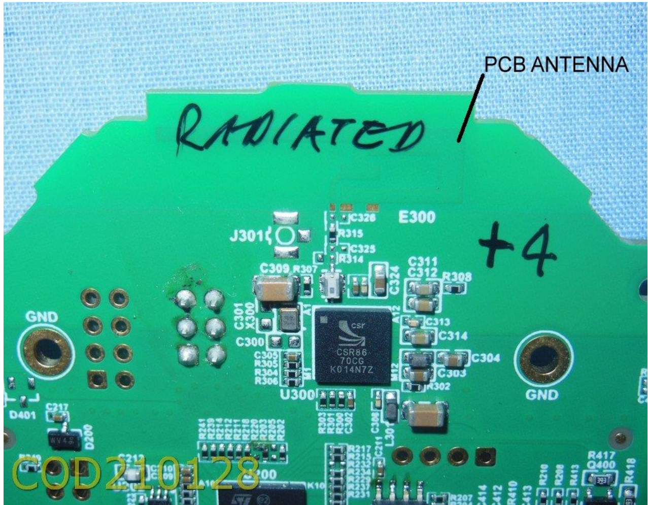
View Radiated PCB Side 2, Showing PCB Trace Antenna Location
