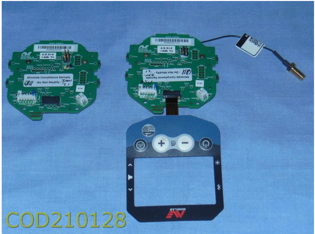
View Both RF Conducted and Radiated PCB with Common User Interface
