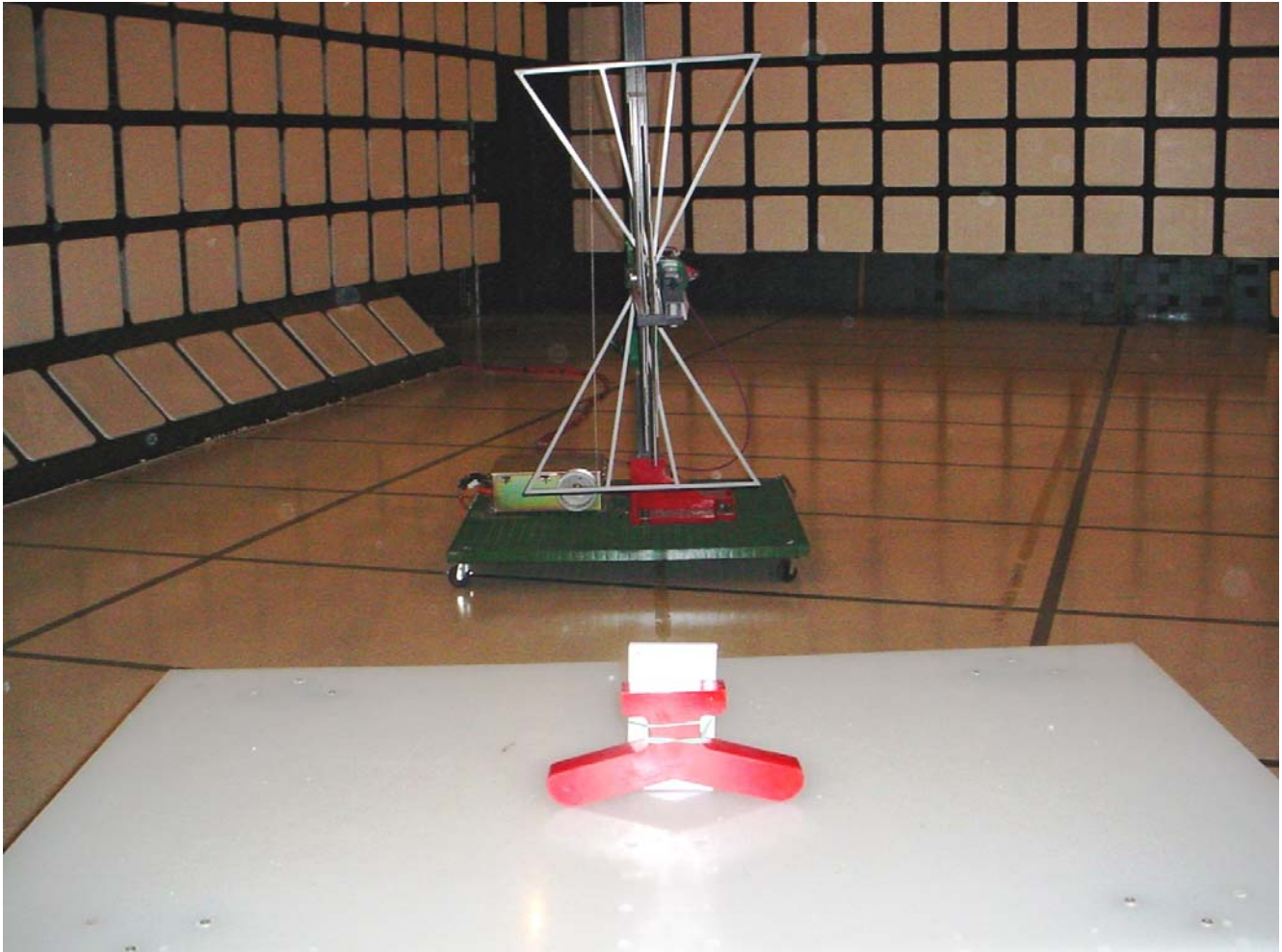
Tx Radiated Emissions at 3 m, Orthogonal Position 2
