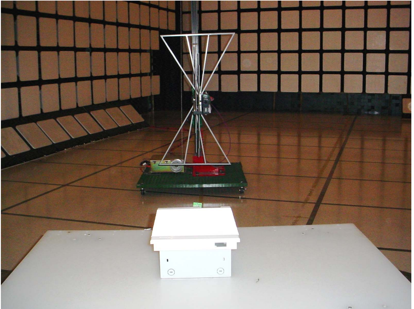
Tx Radiated Emissions at 3 m, Orthogonal Position 3
