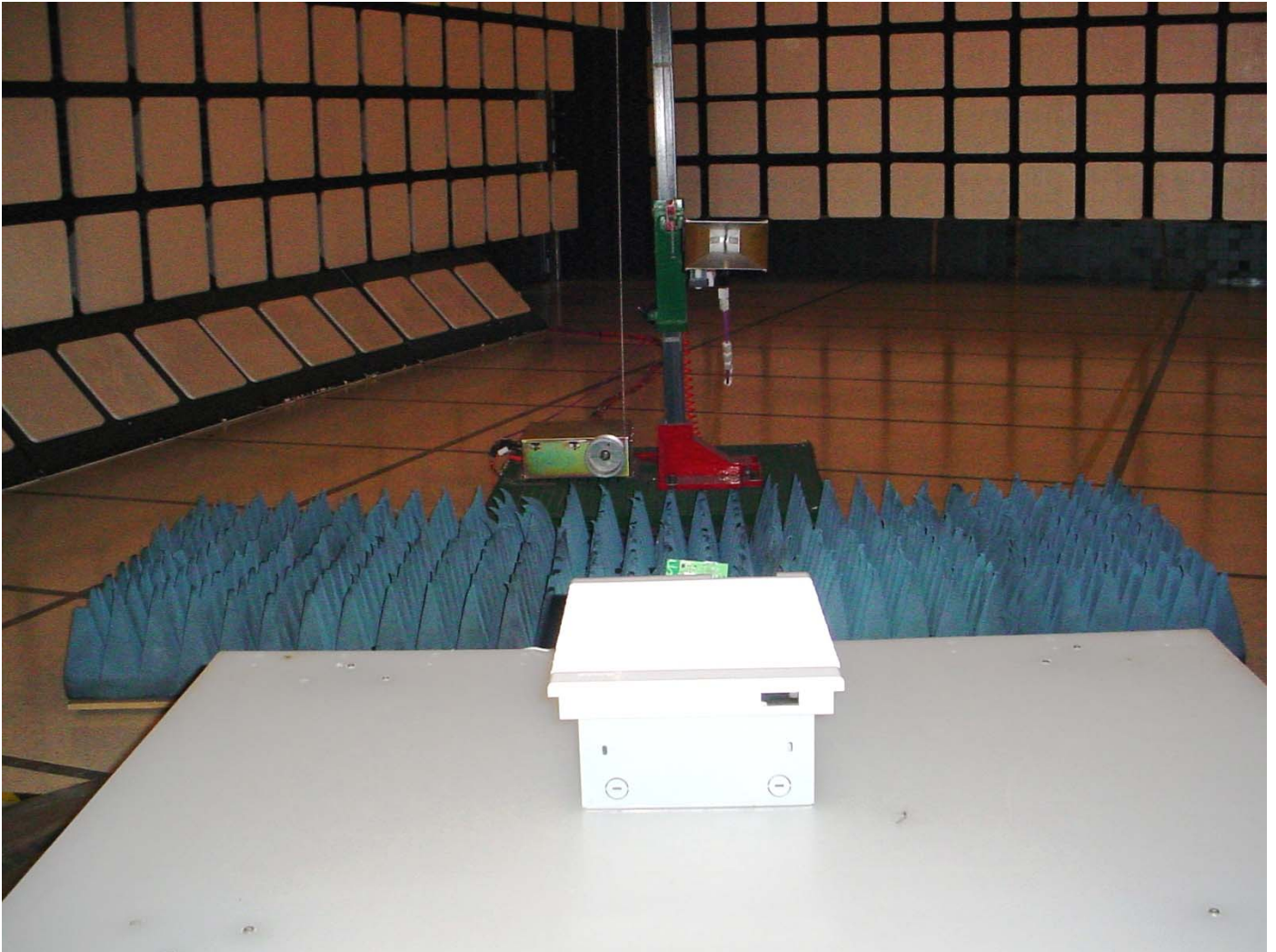
Tx Radiated Emissions at 3 m, Orthogonal Position 2
