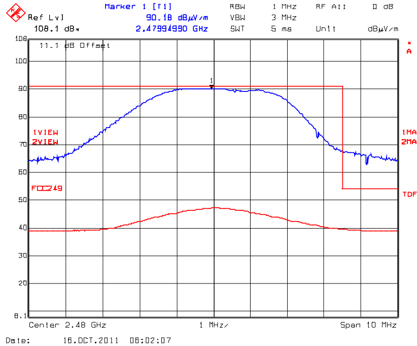
Plot 5.7.4.5. Band-Edge RF Radiated Emissions @ 3 m, Continuous Mode High End of Frequency Band, 2480 MHz, Rx Antenna Orientation: Horizontal
