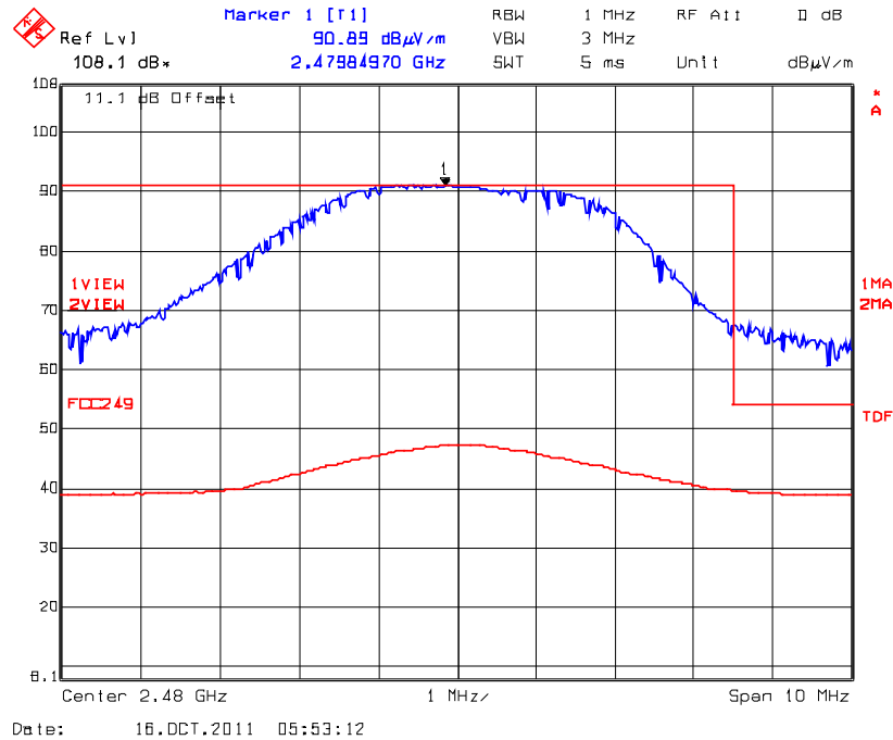
Plot 5.7.4.6. Band-Edge RF Radiated Emissions @ 3 m, Continuous Mode High End of Frequency Band, 2480 MHz, Rx Antenna Orientation: Vertical
