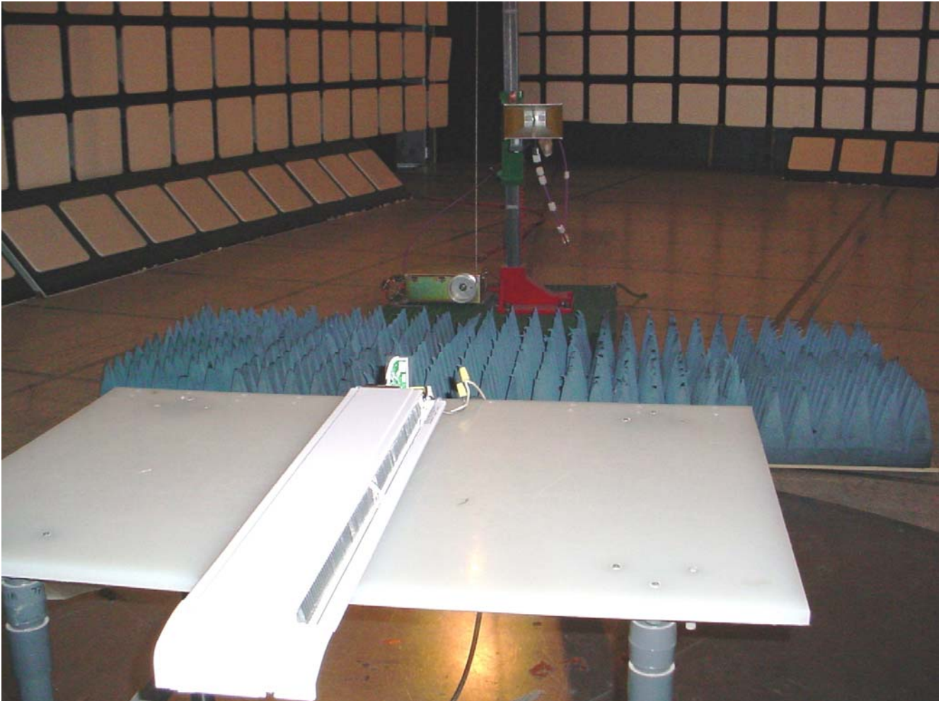
Tx Radiated Emissions at 3 m, Orthogonal Position 3
