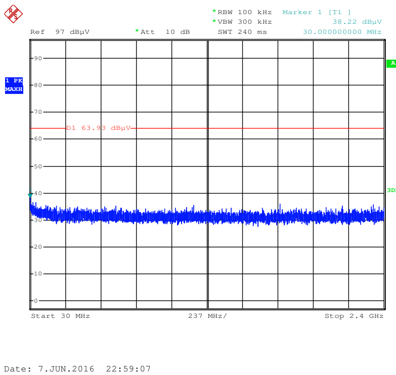
Plot on Configuration IEEE 802.11n MCS0 HT20 / CH 11 / 30MHz~2400MHz (down 30dBc)
