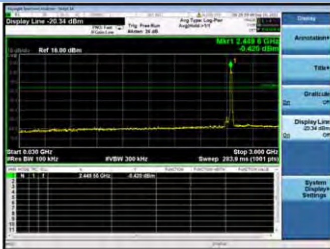
802.11n-20 CHANNEL 10, SPURIOUS 30 MHz ~ 3 GHz
