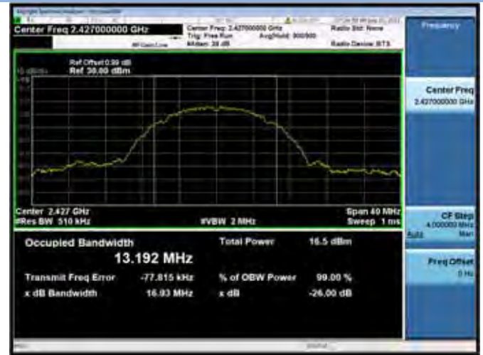
802.11b CHANNEL 4
