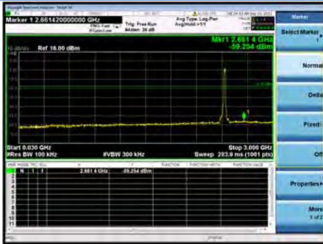
802.11n-20 CHANNEL 6, SPURIOUS 30 MHz ~ 3 GHz
