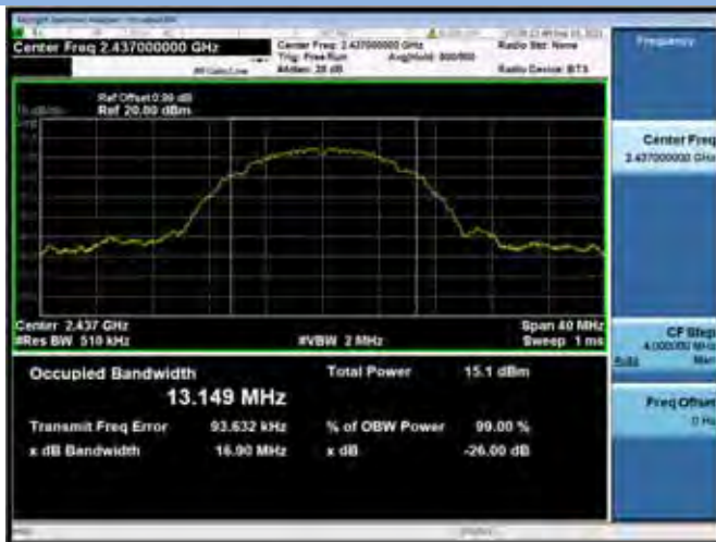
802.11b CHANNEL 6
