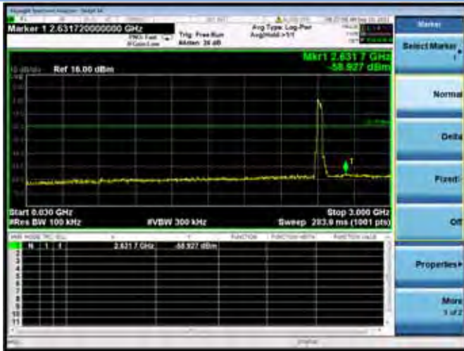
802.11n-40 CHANNEL 3, SPURIOUS 30 MHz ~ 3 GHz
