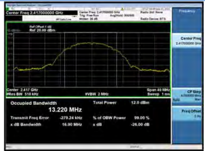
802.11b CHANNEL 2
