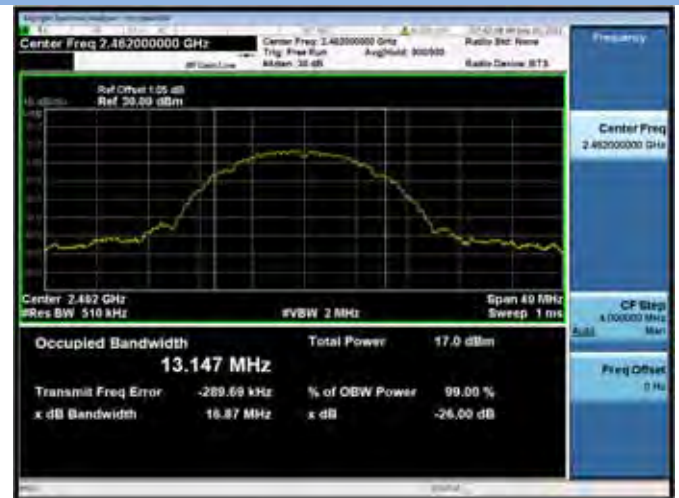
802.11b CHANNEL 11
