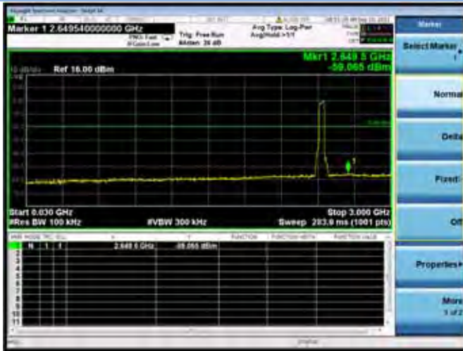
802.11n-40 CHANNEL 6, SPURIOUS 30 MHz ~ 3 GHz
