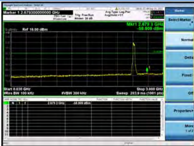
802.11n-40 CHANNEL 4, SPURIOUS 30 MHz ~ 3 GHz
