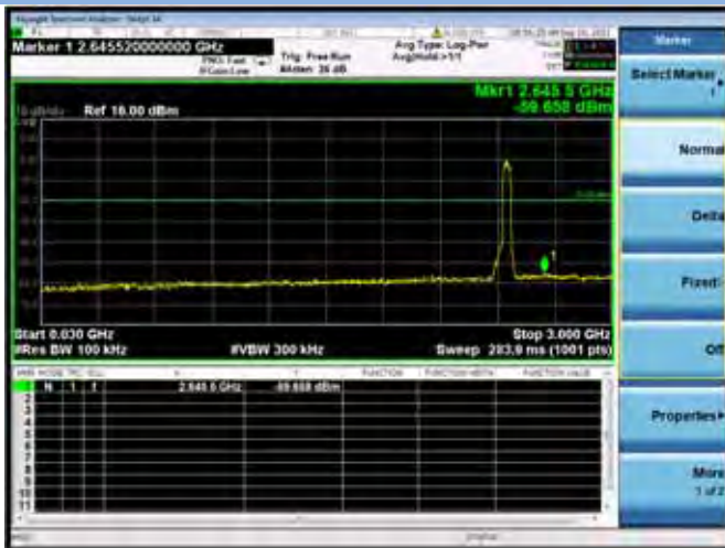
802.11n-40 CHANNEL 9, SPURIOUS 30 MHz ~ 3 GHz
