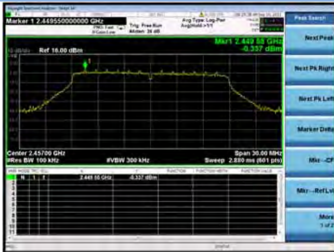
802.11n-20 CHANNEL 10 CARRIER LEVEL
