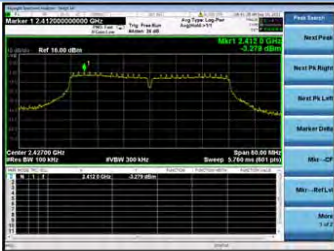
802.11n-40 CHANNEL 4 CARRIER LEVEL
