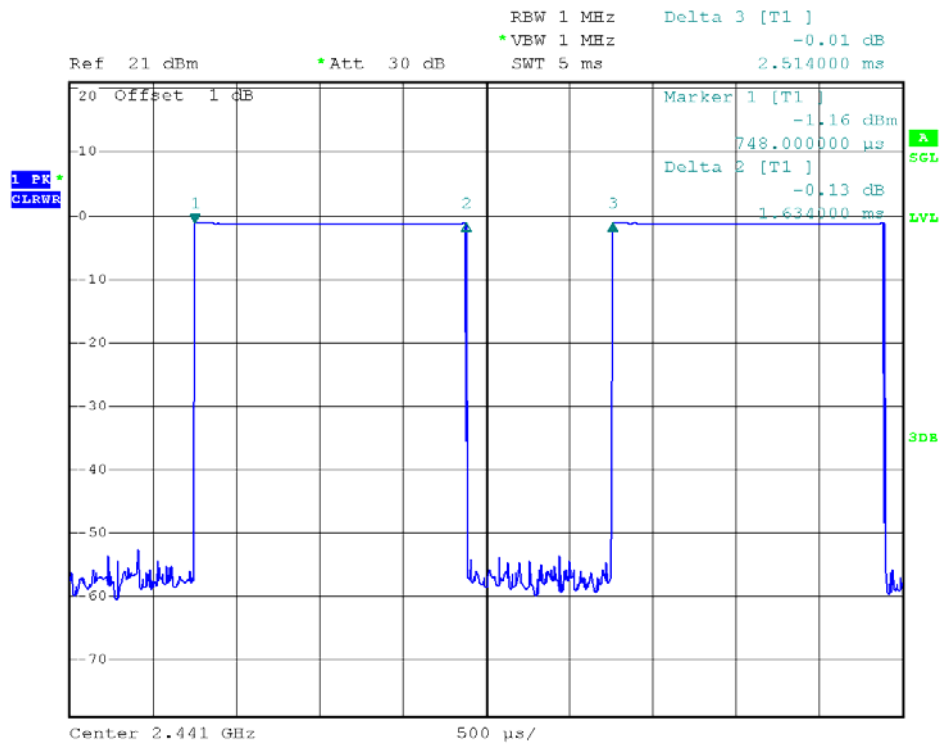
39 Channel @ DH3
