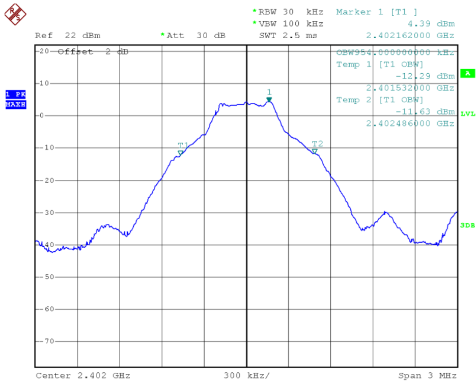
0 Channel @ GFSK
