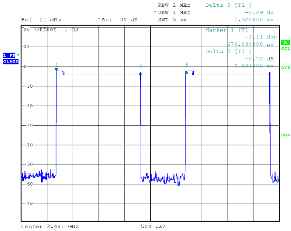
39 Channel @ 2DH3
