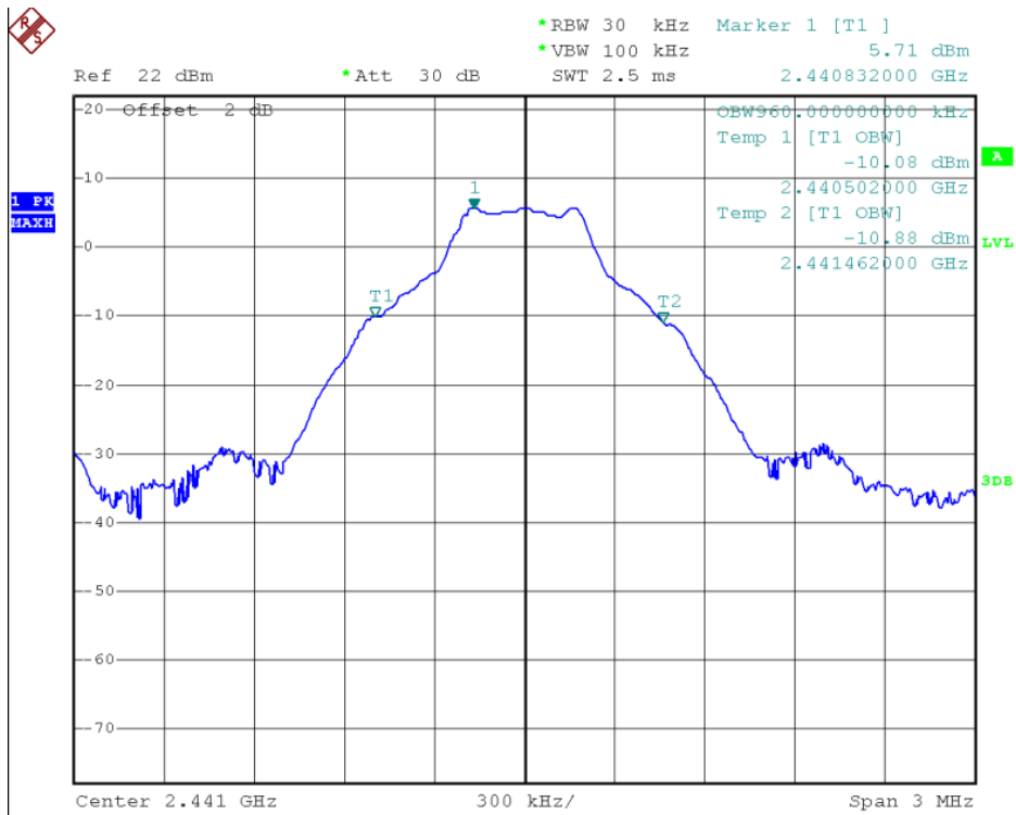
39 Channel @ GFSK
