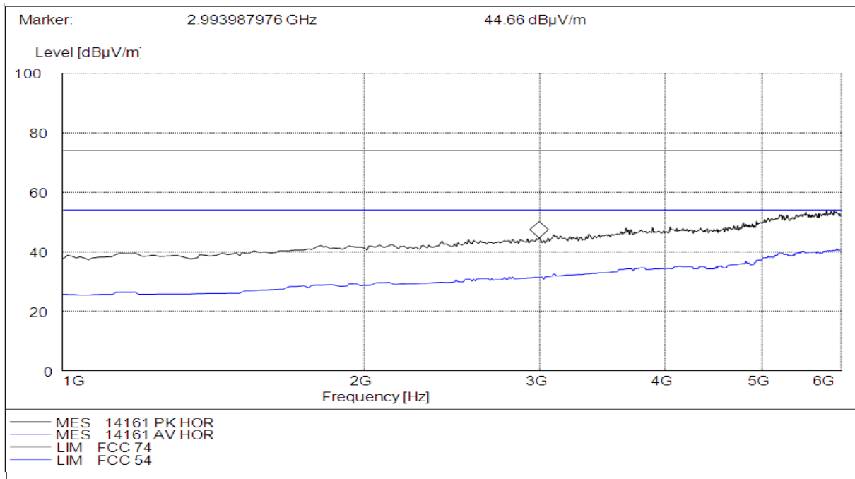
(Plot E: Test Antenna Horizontal 1G – 6G)
