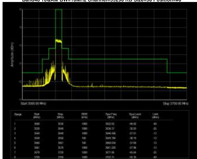
Band48 16QAM BW=10MHz Channel=55290 RB Size=50 Position=#0
