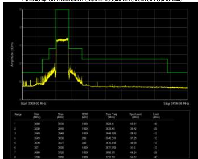
Band48 QPSK BW=20MHz Channel=55340 RB Size=100 Position=#0
