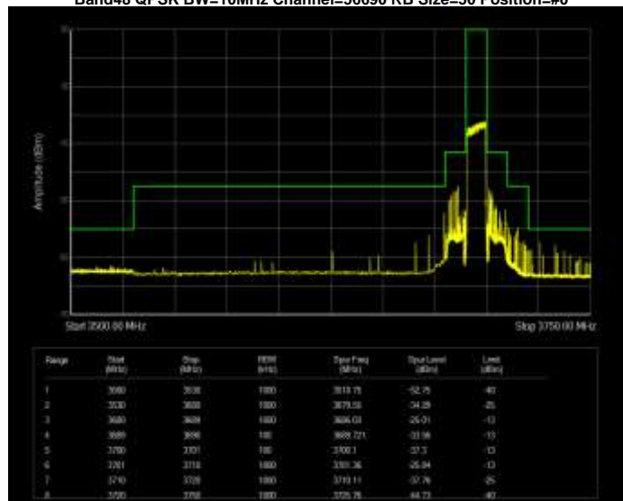
Band48 QPSK BW=10MHz Channel=56690 RB Size=50 Position=#0
