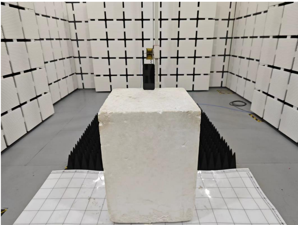
Set-up for Radiated Emission (RE), Above 1GHz
