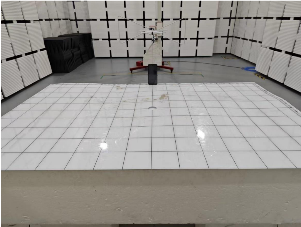
Set-up for Radiated Emission (RE), Below 1GHz
