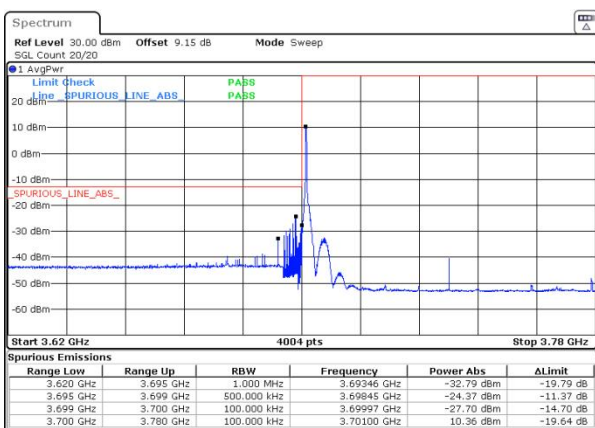
n77(3700-3980) SCS=30kHz DFT_16QAM BW=80MHz LowChannel=649334 RB=1@0
