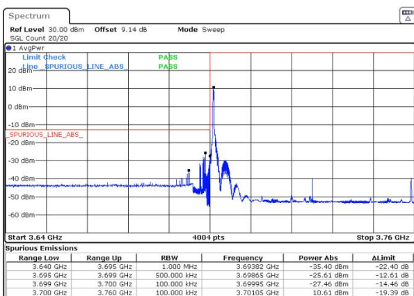
n77(3700-3980) SCS=30kHz DFT_64QAM BW=60MHz LowChannel=648668 RB=1@0
