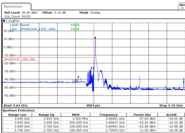
n77(3700-3980) SCS=30kHz DFT_BPSK BW=60MHz LowChannel=648668 RB=1@0
