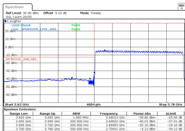
n77(3700-3980) SCS=30kHz DFT_16QAM BW=80MHz LowChannel=649334 RB=216@0
