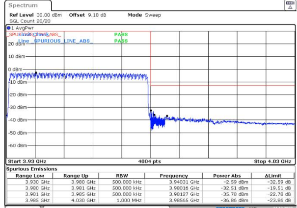
n77(3700-3980) SCS=30kHz CP_QPSK BW=50MHz HighChannel=663666 RB=133@0
