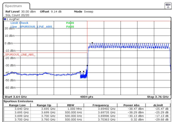
n77(3700-3980) SCS=30kHz DFT_BPSK BW=60MHz LowChannel=648668 RB=162@0
