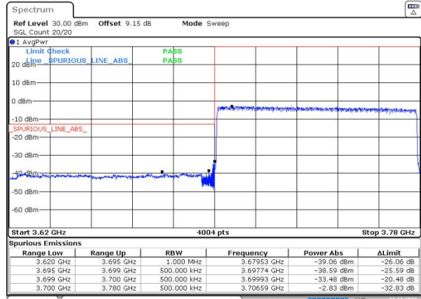
n77(3700-3980) SCS=30kHz DFT_QPSK BW=80MHz LowChannel=649334 RB=216@0
