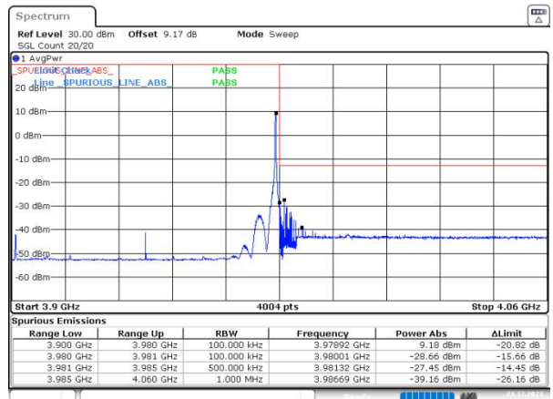
n77(3700-3980) SCS=30kHz DFT_64QAM BW=80MHz HighChannel=662666 RB=1@216
