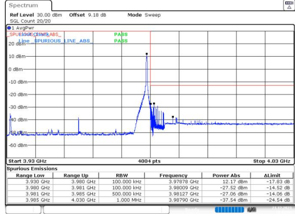
n77(3700-3980) SCS=30kHz DFT_16QAM BW=50MHz HighChannel=663666 RB=1@132
