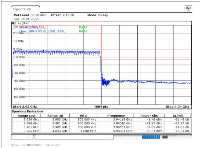
n77(3700-3980) SCS=30kHz DFT_QPSK BW=60MHz HighChannel=663332 RB=162@0
