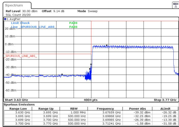
n77(3700-3980) SCS=30kHz DFT_BPSK BW=70MHz LowChannel=649000 RB=180@0
