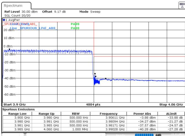
n77(3700-3980) SCS=30kHz DFT_16QAM BW=80MHz HighChannel=662666 RB=216@0
