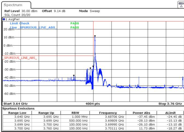
n77(3700-3980) SCS=30kHz DFT_16QAM BW=60MHz LowChannel=648668 RB=1@0
