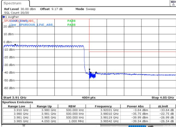
n77(3700-3980) SCS=30kHz DFT_64QAM BW=70MHz HighChannel=663000 RB=180@0
