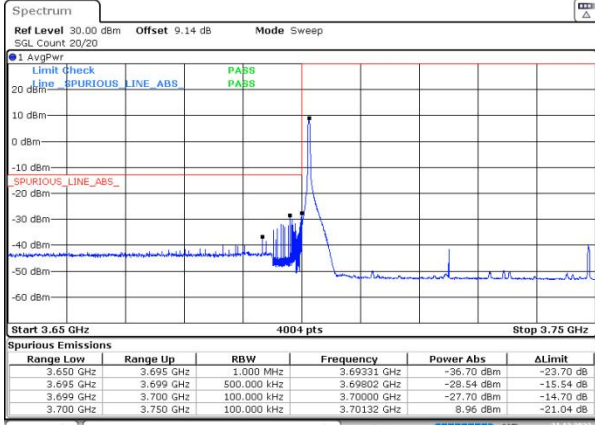
n77(3700-3980) SCS=30kHz DFT_256QAM BW=50MHz LowChannel=648334 RB=1@0
