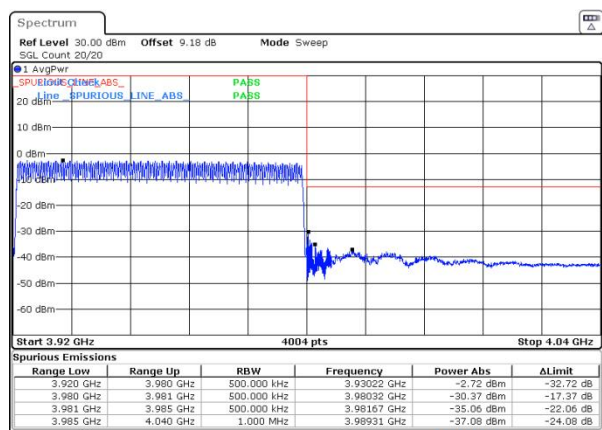
n77(3700-3980) SCS=30kHz DFT_256QAM BW=60MHz HighChannel=663332 RB=1@161
