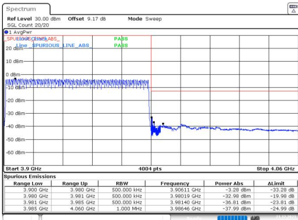
n77(3700-3980) SCS=30kHz DFT_QPSK BW=80MHz HighChannel=662666 RB=216@0
