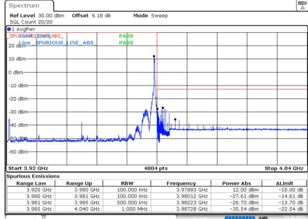
n77(3700-3980) SCS=30kHz DFT_64QAM BW=60MHz HighChannel=663332 RB=1@161
