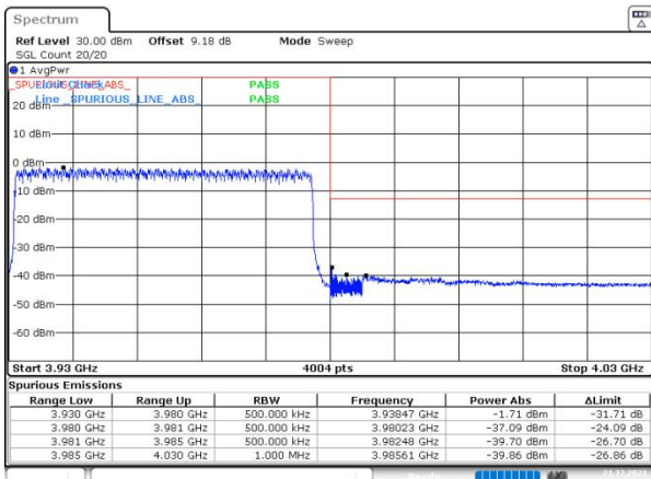
n77(3700-3980) SCS=30kHz DFT_16QAM BW=50MHz HighChannel=663666 RB=128@0
