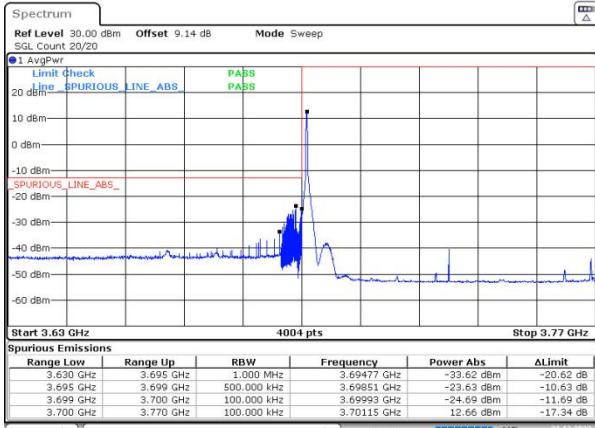
n77(3700-3980) SCS=30kHz DFT_BPSK BW=70MHz LowChannel=649000 RB=1@0
