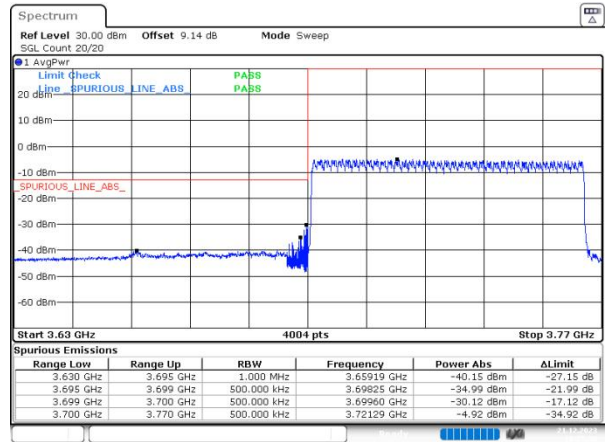
n77(3700-3980) SCS=30kHz DFT_64QAM BW=70MHz LowChannel=649000 RB=180@0
