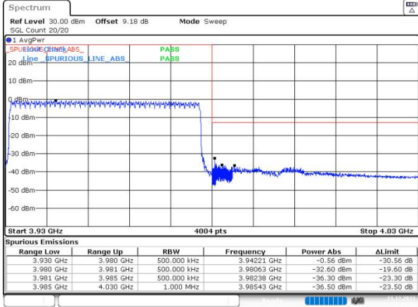
n77(3700-3980) SCS=30kHz DFT_QPSK BW=50MHz HighChannel=663666 RB=128@0
