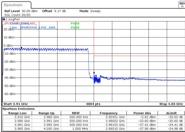
n77(3700-3980) SCS=30kHz DFT_QPSK BW=70MHz HighChannel=663000 RB=180@0
