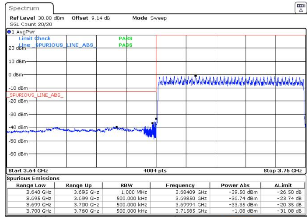
n77(3700-3980) SCS=30kHz DFT_16QAM BW=60MHz LowChannel=648668 RB=162@0
