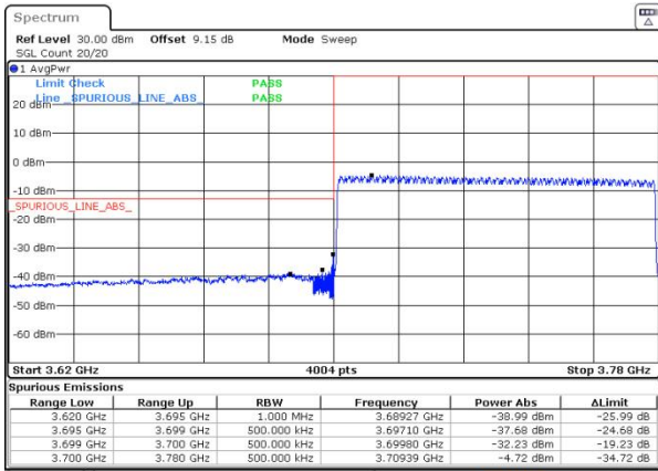
n77(3700-3980) SCS=30kHz DFT_256QAM BW=80MHz LowChannel=649334 RB=1@0
