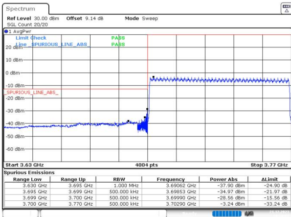
n77(3700-3980) SCS=30kHz DFT_256QAM BW=70MHz LowChannel=649000 RB=1@0
