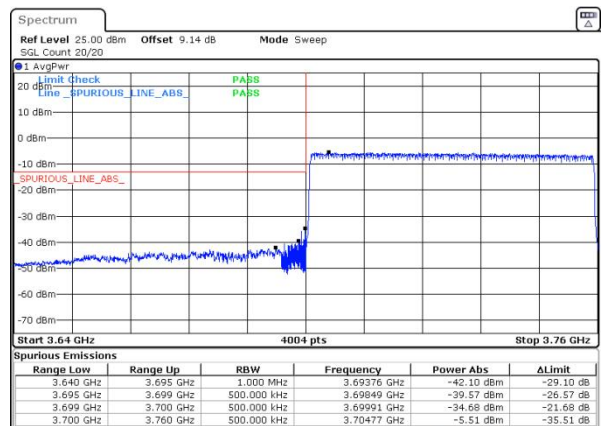
n77(3700-3980) SCS=30kHz DFT_64QAM BW=60MHz LowChannel=648668 RB=162@0
