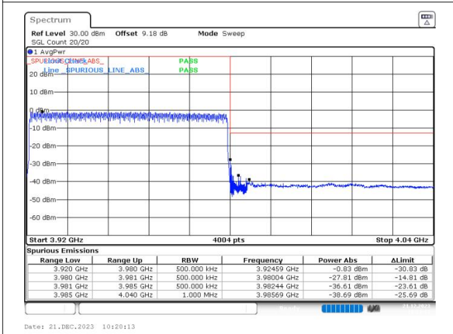
n77(3700-3980) SCS=30kHz DFT_BPSK BW=60MHz HighChannel=663332 RB=162@0
