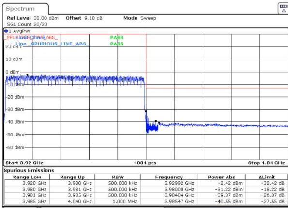
n77(3700-3980) SCS=30kHz DFT_16QAM BW=60MHz HighChannel=663332 RB=162@0
