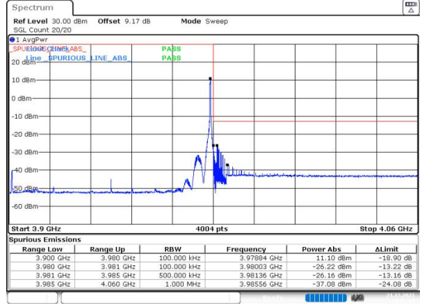
n77(3700-3980) SCS=30kHz DFT_16QAM BW=80MHz HighChannel=662666 RB=1@216
