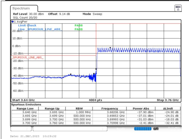
n77(3700-3980) SCS=30kHz CP_QPSK BW=60MHz LowChannel=648668 RB=162@0
