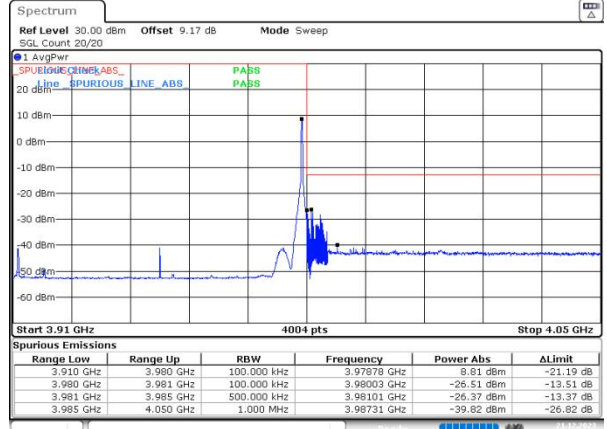
n77(3700-3980) SCS=30kHz DFT_256QAM BW=70MHz HighChannel=663000 RB=1@188
