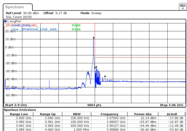
n77(3700-3980) SCS=30kHz DFT_BPSK BW=80MHz HighChannel=662666 RB=1@216
