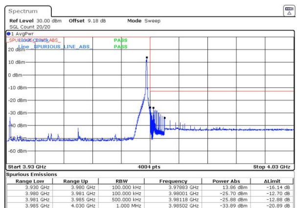
n77(3700-3980) SCS=30kHz DFT_BPSK BW=50MHz HighChannel=663666 RB=1@132
