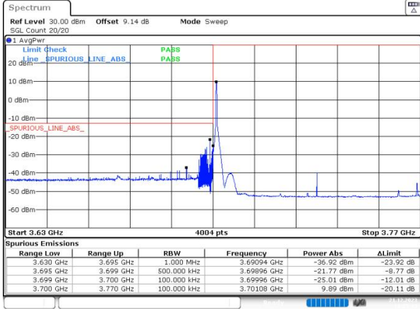
n77(3700-3980) SCS=30kHz DFT_64QAM BW=70MHz LowChannel=649000 RB=1@0
