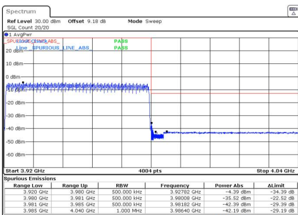
n77(3700-3980) SCS=30kHz DFT_64QAM BW=60MHz HighChannel=663332 RB=162@0
