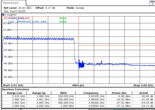
n77(3700-3980) SCS=30kHz DFT_BPSK BW=70MHz HighChannel=663000 RB=180@0
