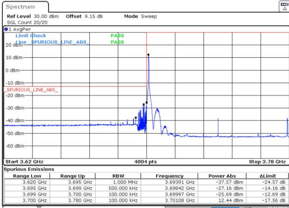
n77(3700-3980) SCS=30kHz DFT_QPSK BW=80MHz LowChannel=649334 RB=1@0
