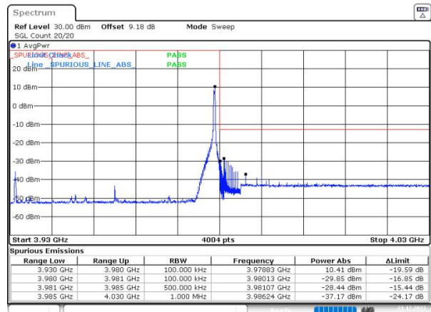
n77(3700-3980) SCS=30kHz DFT_64QAM BW=50MHz HighChannel=663666 RB=1@132
