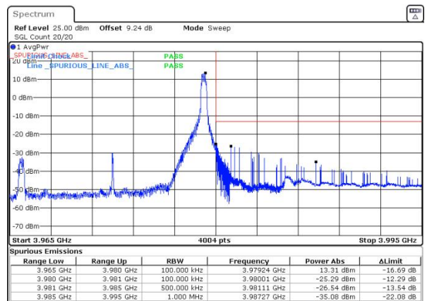
n77(3700-3980) SCS=30kHz DFT_BPSK BW=15MHz HighChannel=664832 RB=1@37
