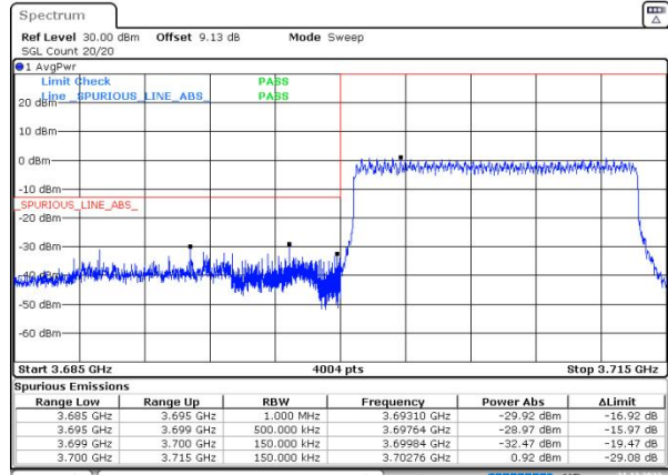
n77(3700-3980) SCS=30kHz DFT_QPSK BW=15MHz LowChannel=647168 RB=36@0
