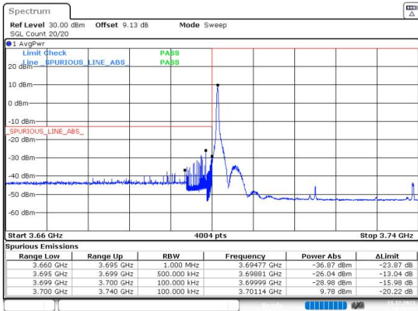
n77(3700-3980) SCS=30kHz DFT_64QAM BW=40MHz LowChannel=648000 RB=1@0
