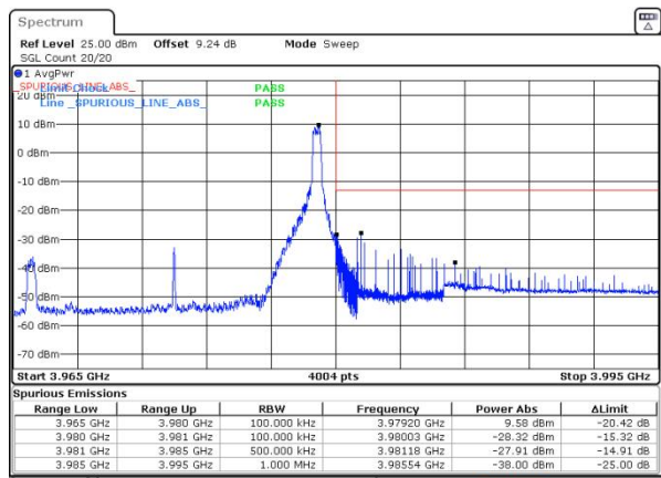
n77(3700-3980) SCS=30kHz DFT_64QAM BW=15MHz HighChannel=664832 RB=1@37
