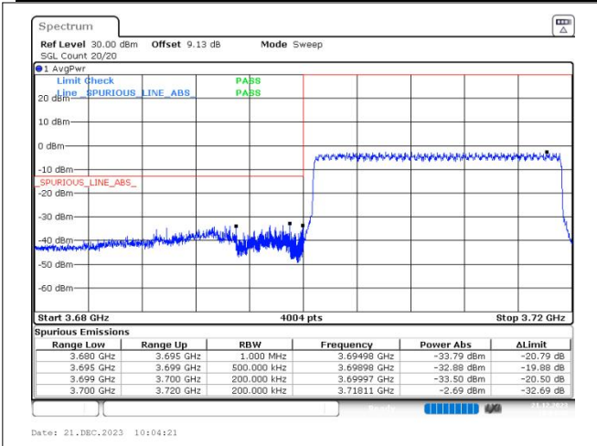
n77(3700-3980) SCS=30kHz CP_QPSK BW=20MHz LowChannel=647334 RB=51@0
