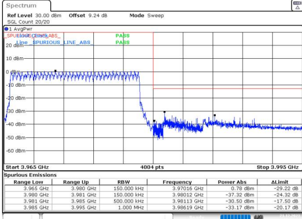
n77(3700-3980) SCS=30kHz DFT_QPSK BW=15MHz HighChannel=664832 RB=36@0
