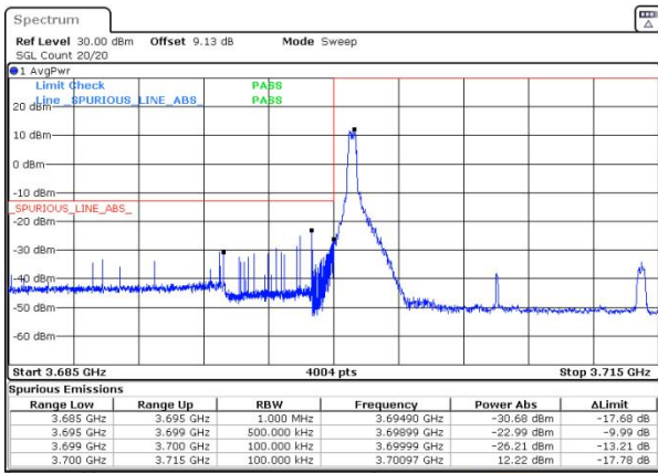
n77(3700-3980) SCS=30kHz DFT_QPSK BW=15MHz LowChannel=647168 RB=1@0
