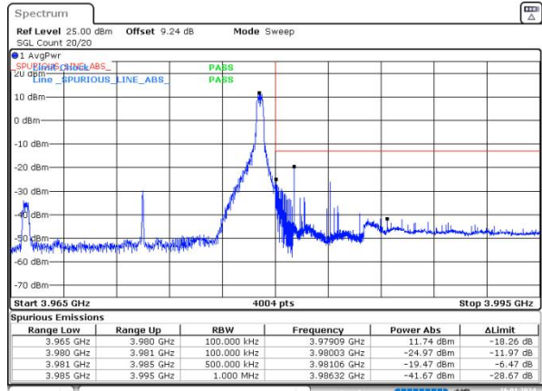
n77(3700-3980) SCS=30kHz DFT_16QAM BW=15MHz HighChannel=664832 RB=1@37
