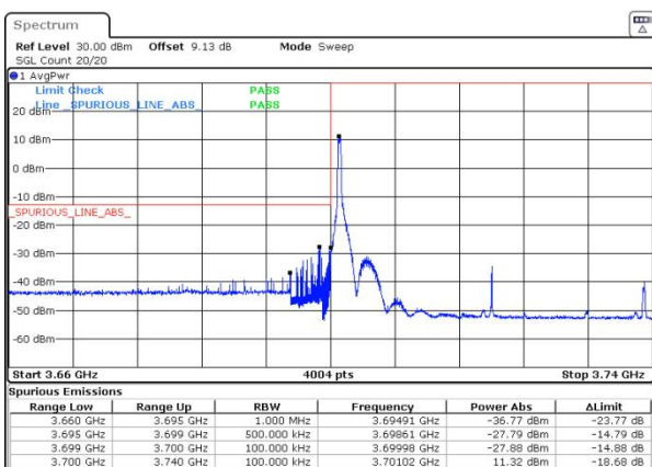
n77(3700-3980) SCS=30kHz DFT_QPSK BW=40MHz LowChannel=648000 RB=1@0
