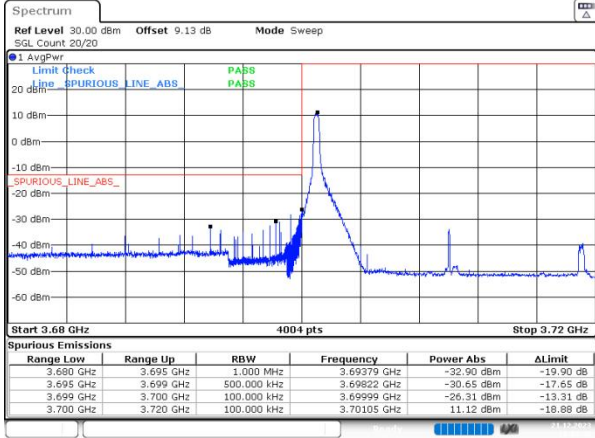
n77(3700-3980) SCS=30kHz DFT_16QAM BW=20MHz LowChannel=647334 RB=1@0
