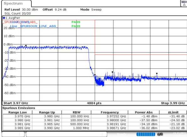
n77(3700-3980) SCS=30kHz DFT_64QAM BW=10MHz HighChannel=665000 RB=24@0
