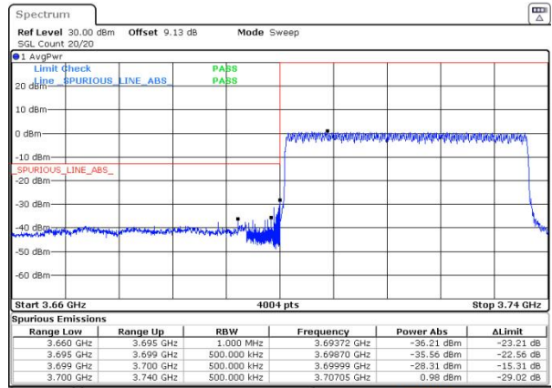
n77(3700-3980) SCS=30kHz DFT_BPSK BW=40MHz LowChannel=648000 RB=100@0
