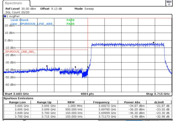
n77(3700-3980) SCS=30kHz DFT_256QAM BW=15MHz LowChannel=647168 RB=36@0
