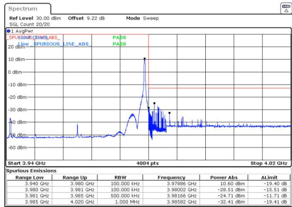
n77(3700-3980) SCS=30kHz DFT_16QAM BW=40MHz HighChannel=664000 RB=1@105
