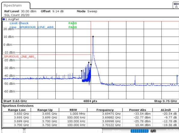
n77(3700-3980) SCS=30kHz DFT_16QAM BW=50MHz LowChannel=648334 RB=1@0
