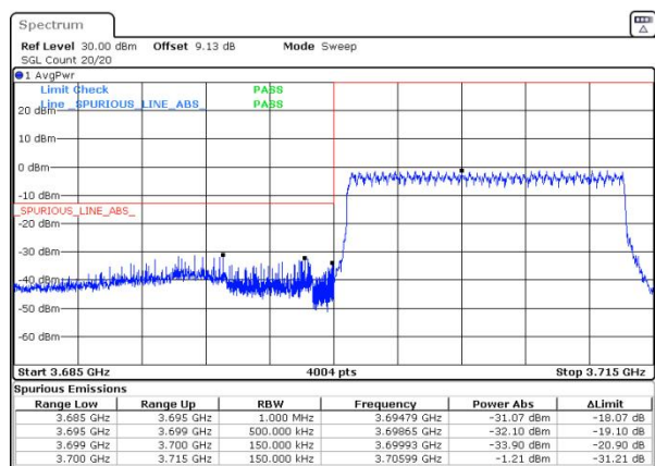
n77(3700-3980) SCS=30kHz DFT_16QAM BW=15MHz LowChannel=647168 RB=36@0
