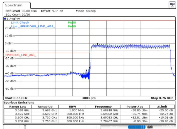
n77(3700-3980) SCS=30kHz DFT_16QAM BW=50MHz LowChannel=648334 RB=128@0
