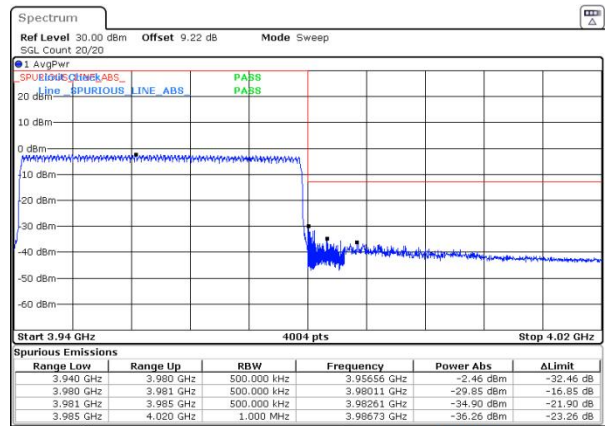
n77(3700-3980) SCS=30kHz DFT_256QAM BW=40MHz HighChannel=664000 RB=1@105
