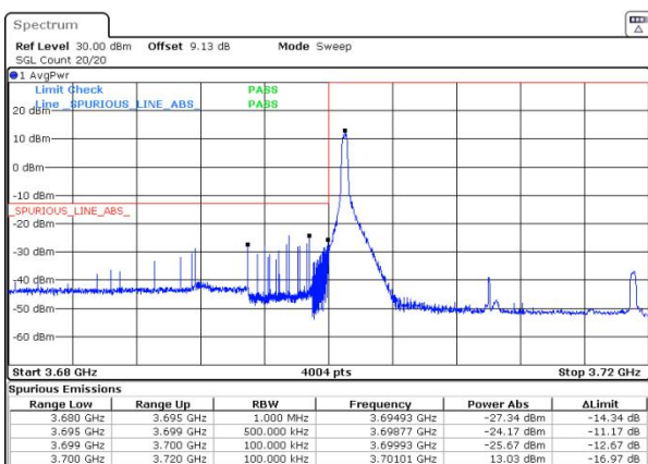
n77(3700-3980) SCS=30kHz DFT_BPSK BW=20MHz LowChannel=647334 RB=1@0
