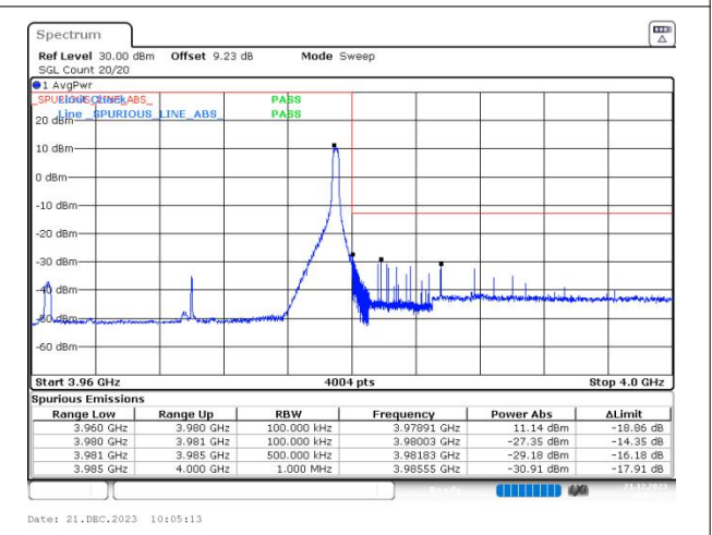
n77(3700-3980) SCS=30kHz DFT_16QAM BW=20MHz HighChannel=664666 RB=1@50
