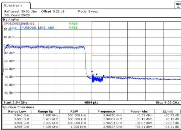
n77(3700-3980) SCS=30kHz DFT_QPSK BW=40MHz HighChannel=664000 RB=100@0
