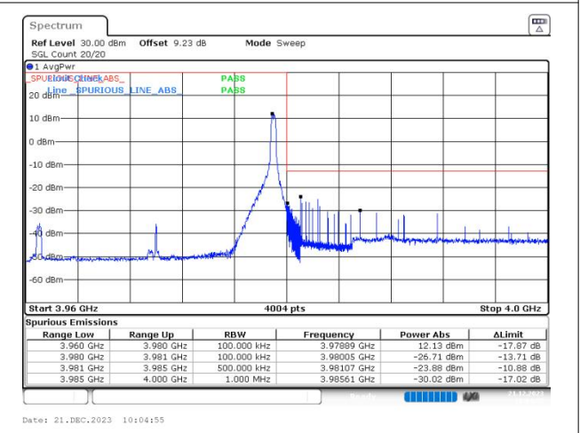
n77(3700-3980) SCS=30kHz DFT_QPSK BW=20MHz HighChannel=664666 RB=1@50
