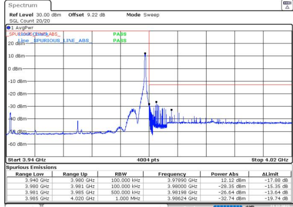
n77(3700-3980) SCS=30kHz DFT_QPSK BW=40MHz HighChannel=664000 RB=1@105
