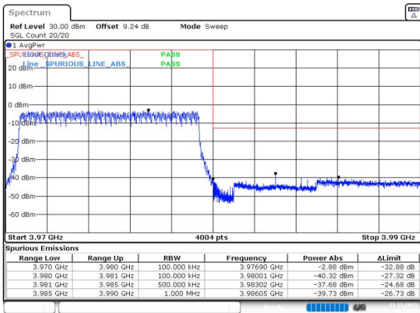
n77(3700-3980) SCS=30kHz DFT_64QAM BW=10MHz HighChannel=665000 RB=24@0
