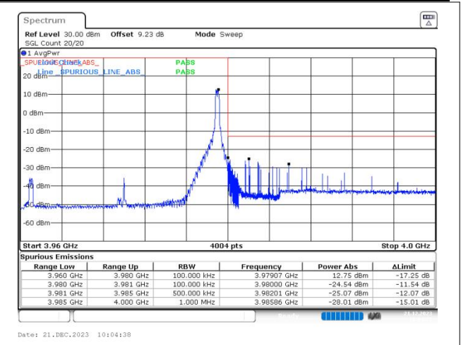
n77(3700-3980) SCS=30kHz DFT_BPSK BW=20MHz HighChannel=664666 RB=1@50
