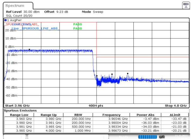
n77(3700-3980) SCS=30kHz DFT_256QAM BW=20MHz HighChannel=664666 RB=1@50
