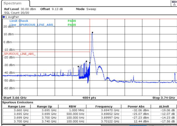
n77(3700-3980) SCS=30kHz DFT_BPSK BW=40MHz LowChannel=648000 RB=1@0
