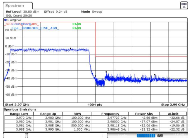
n77(3700-3980) SCS=30kHz DFT_256QAM BW=10MHz HighChannel=665000 RB=1@23
