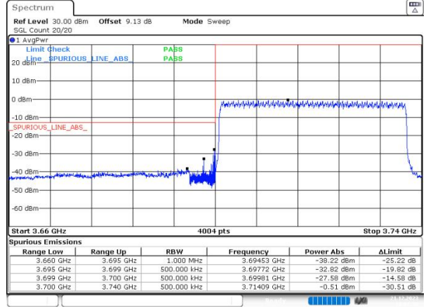
n77(3700-3980) SCS=30kHz DFT_64QAM BW=40MHz LowChannel=648000 RB=100@0
