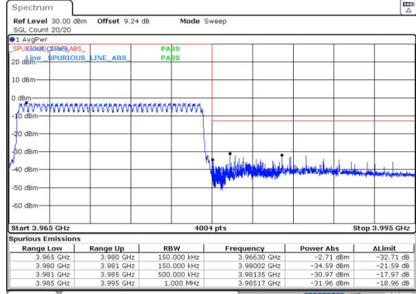
n77(3700-3980) SCS=30kHz CP_QPSK BW=15MHz HighChannel=664832 RB=38@0
