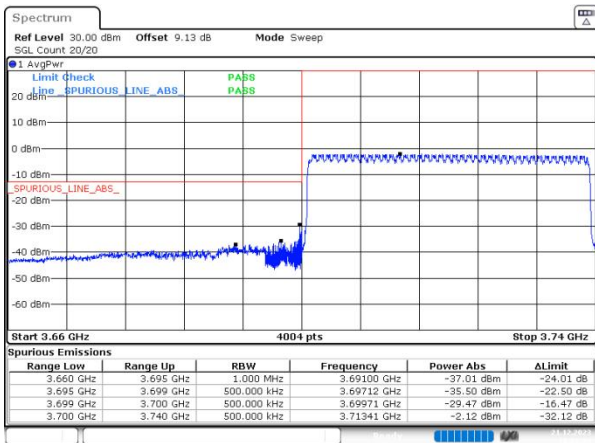
n77(3700-3980) SCS=30kHz DFT_256QAM BW=40MHz LowChannel=648000 RB=1@0
