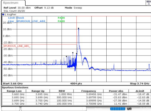
n77(3700-3980) SCS=30kHz DFT_64QAM BW=40MHz LowChannel=648000 RB=1@0
