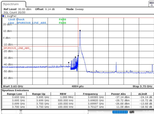
n77(3700-3980) SCS=30kHz DFT_QPSK BW=50MHz LowChannel=648334 RB=1@0
