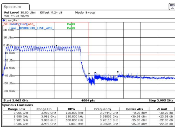
n77(3700-3980) SCS=30kHz DFT_16QAM BW=15MHz HighChannel=664832 RB=36@0
