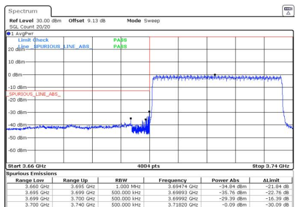
n77(3700-3980) SCS=30kHz DFT_QPSK BW=40MHz LowChannel=648000 RB=100@0
