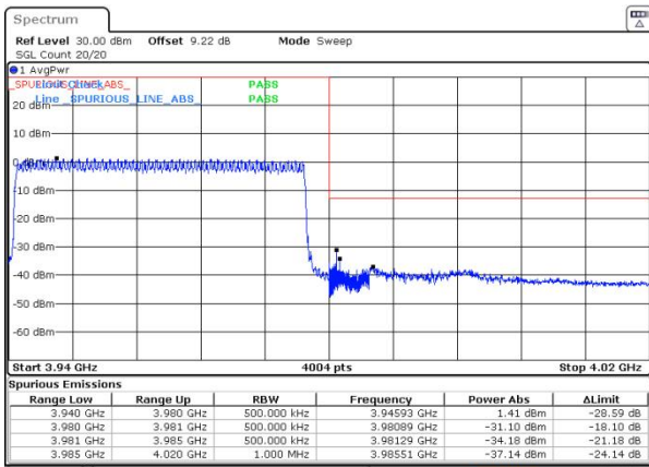
n77(3700-3980) SCS=30kHz DFT_BPSK BW=40MHz HighChannel=664000 RB=100@0
