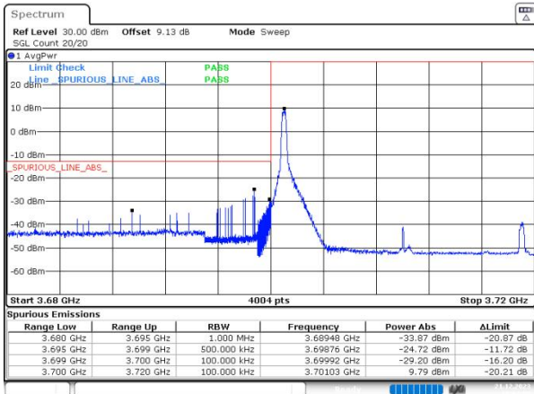
n77(3700-3980) SCS=30kHz DFT_64QAM BW=20MHz LowChannel=647334 RB=1@0
