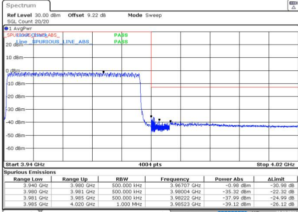
n77(3700-3980) SCS=30kHz DFT_64QAM BW=40MHz HighChannel=664000 RB=100@0
