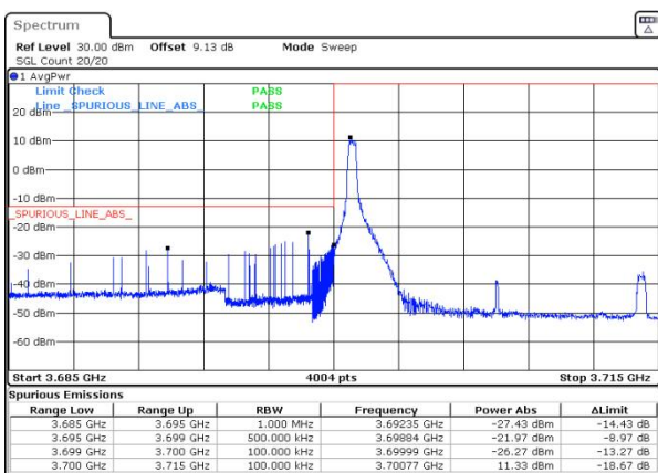
n77(3700-3980) SCS=30kHz DFT_16QAM BW=15MHz LowChannel=647168 RB=1@0
