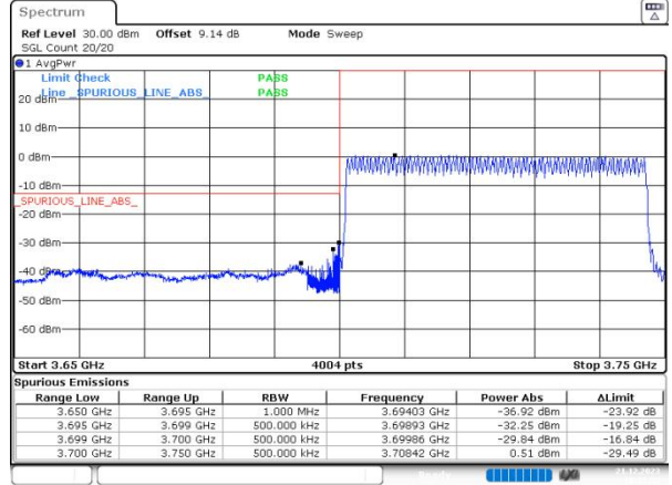
n77(3700-3980) SCS=30kHz DFT_QPSK BW=50MHz LowChannel=648334 RB=128@0
