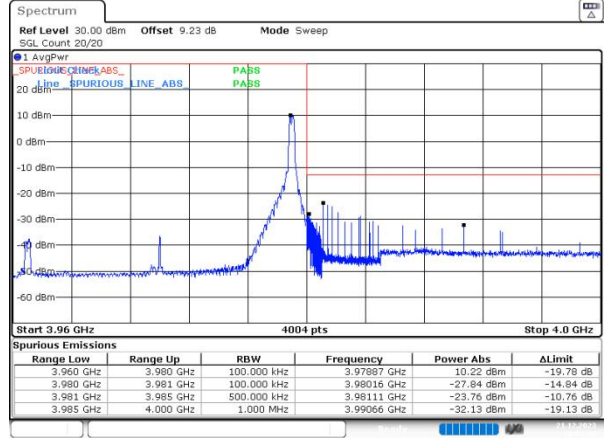
n77(3700-3980) SCS=30kHz DFT_64QAM BW=20MHz HighChannel=664666 RB=1@50
