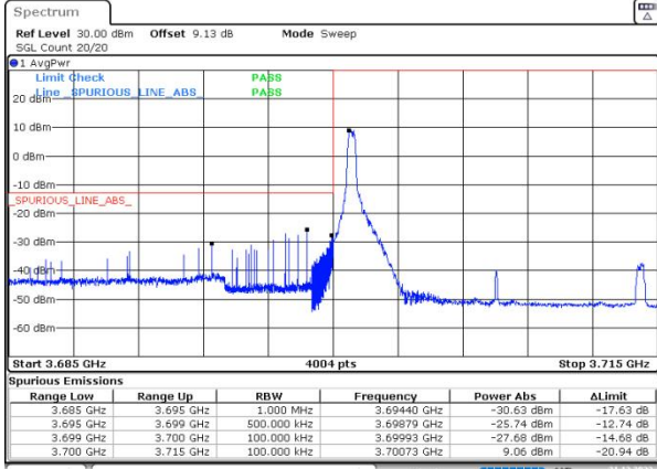
n77(3700-3980) SCS=30kHz DFT_256QAM BW=15MHz LowChannel=647168 RB=1@0
