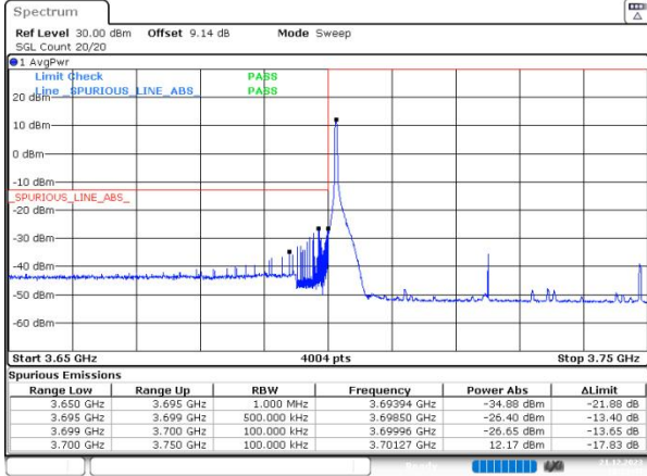
n77(3700-3980) SCS=30kHz DFT_QPSK BW=50MHz LowChannel=648334 RB=1@0
