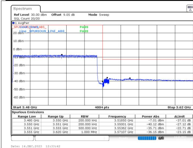
n78(3450-3550) SCS=30kHz DFT_BPSK BW=70MHz HighChannel=634332 RB=180@0
