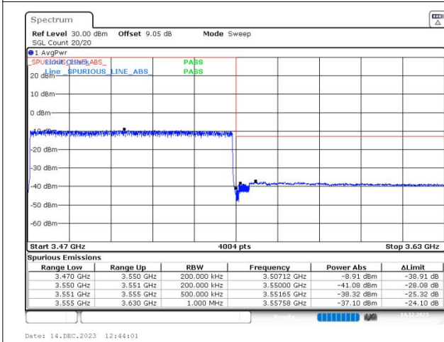
n78(3450-3550) SCS=30kHz DFT_16QAM BW=80MHz HighChannel=634000 RB=216@0
