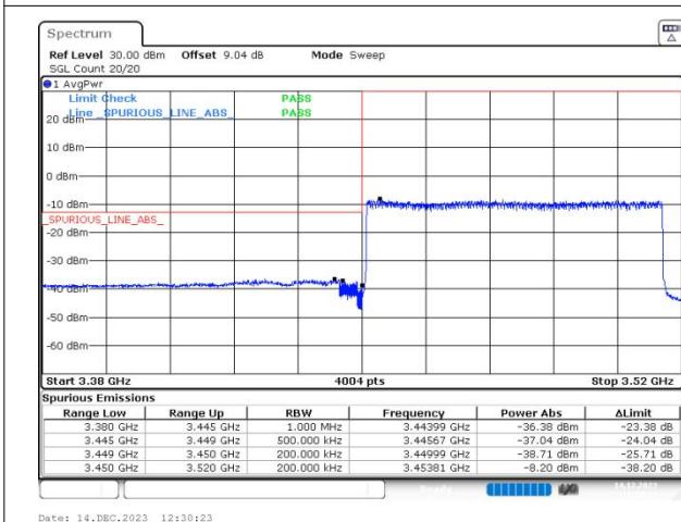
n78(3450-3550) SCS=30kHz DFT_16QAM BW=70MHz LowChannel=632334 RB=180@0
