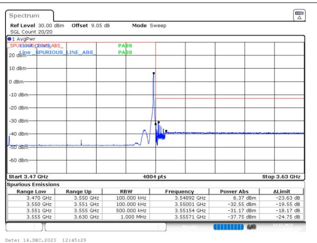
n78(3450-3550) SCS=30kHz DFT_256QAM BW=80MHz HighChannel=634000 RB=1@216
