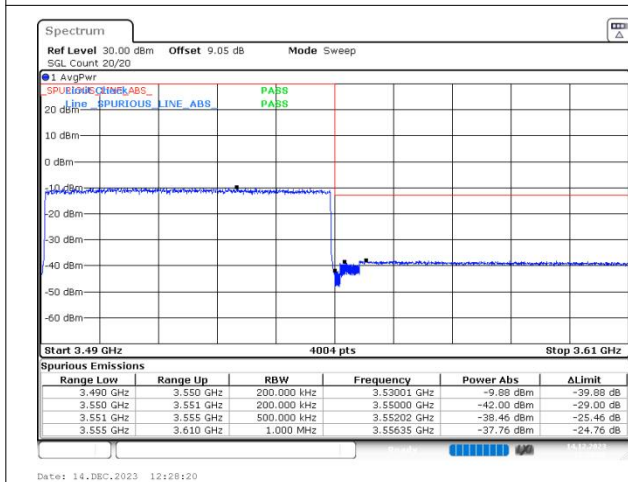
n78(3450-3550) SCS=30kHz DFT_256QAM BW=60MHz HighChannel=634666 RB=162@0
