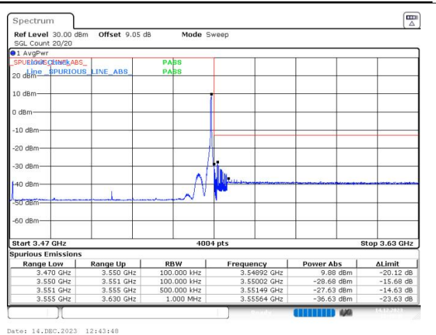
n78(3450-3550) SCS=30kHz DFT_16QAM BW=80MHz HighChannel=634000 RB=1@216
