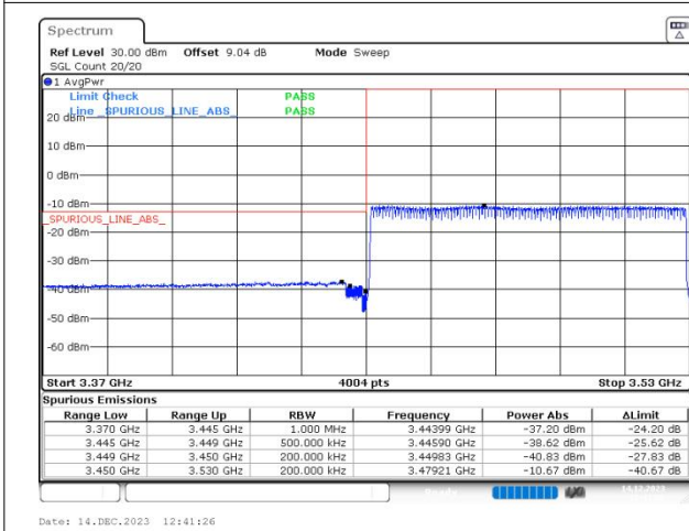
n78(3450-3550) SCS=30kHz CP_QPSK BW=80MHz LowChannel=632668 RB=217@0
