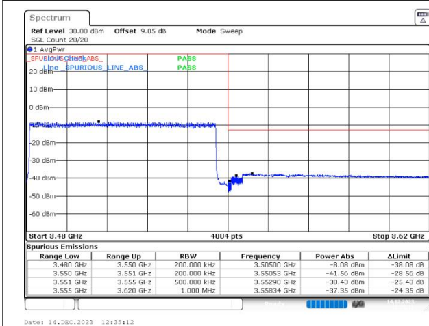
n78(3450-3550) SCS=30kHz DFT_16QAM BW=70MHz HighChannel=634332 RB=180@0
