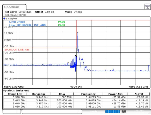
n78(3450-3550) SCS=30kHz DFT_BPSK BW=60MHz LowChannel=632000 RB=1@0
