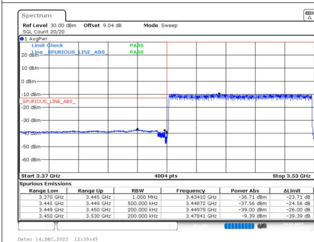
n78(3450-3550) SCS=30kHz DFT_64QAM BW=80MHz LowChannel=632668 RB=216@0
