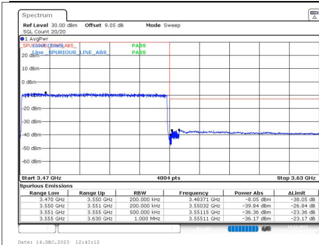
n78(3450-3550) SCS=30kHz DFT_QPSK BW=80MHz HighChannel=634000 RB=216@0
