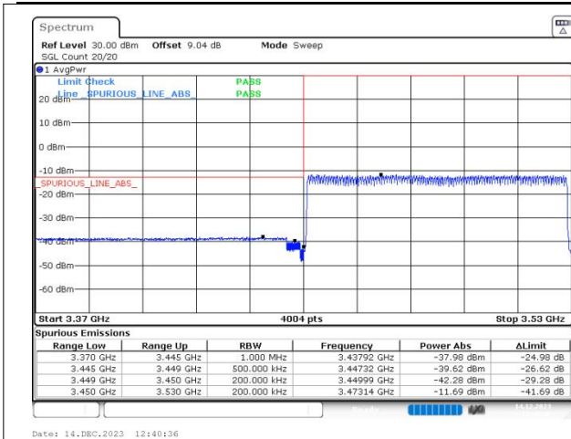
n78(3450-3550) SCS=30kHz DFT_256QAM BW=80MHz LowChannel=632668 RB=216@0
