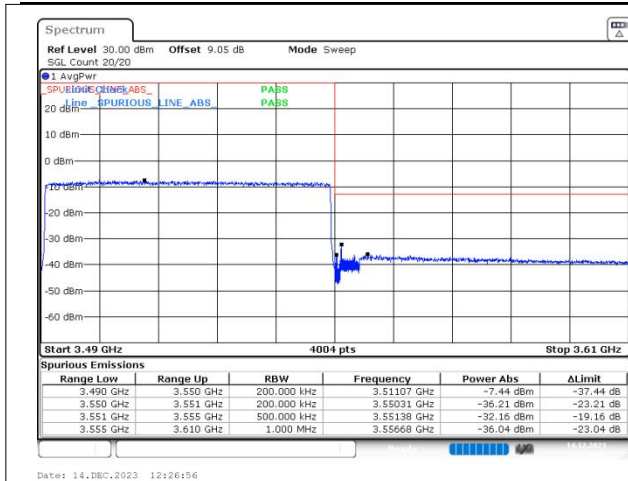
n78(3450-3550) SCS=30kHz DFT_16QAM BW=60MHz HighChannel=634666 RB=162@0
