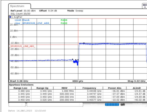
n78(3450-3550) SCS=30kHz CP_QPSK BW=70MHz LowChannel=632334 RB=189@0
