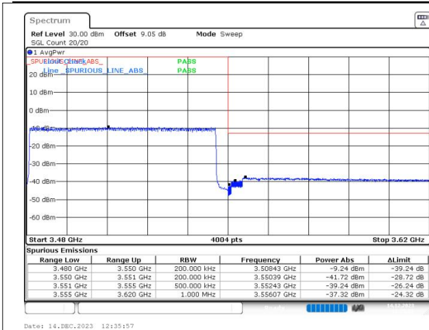
n78(3450-3550) SCS=30kHz DFT_64QAM BW=70MHz HighChannel=634332 RB=180@0
