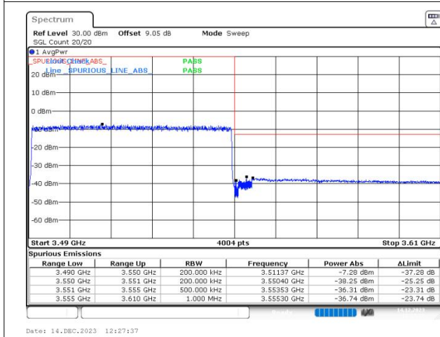
n78(3450-3550) SCS=30kHz DFT_64QAM BW=60MHz HighChannel=634666 RB=162@0
