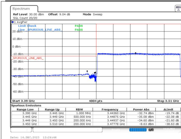
n78(3450-3550) SCS=30kHz CP_QPSK BW=60MHz LowChannel=632000 RB=162@0
