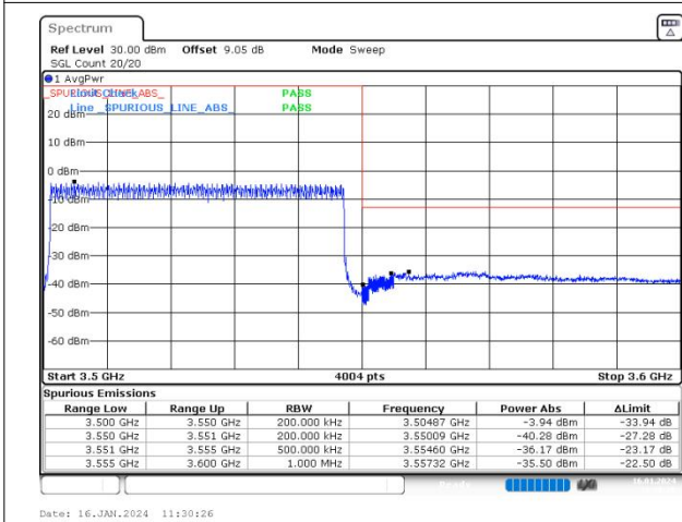
n78(3450-3550) SCS=30kHz DFT_16QAM BW=50MHz HighChannel=635000 RB=128@0
