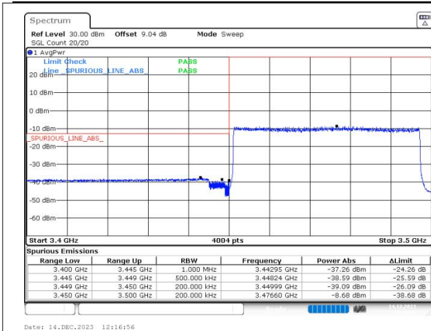
n78(3450-3550) SCS=30kHz DFT_256QAM BW=50MHz LowChannel=631668 RB=128@0
