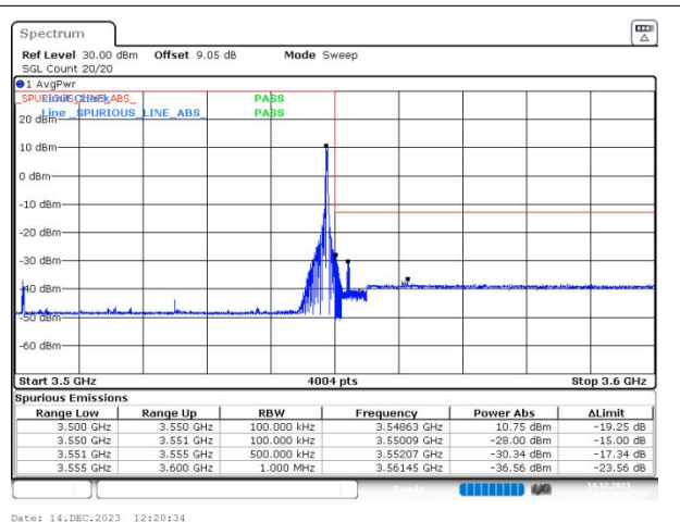
n78(3450-3550) SCS=30kHz DFT_256QAM BW=50MHz HighChannel=635000 RB=1@132
