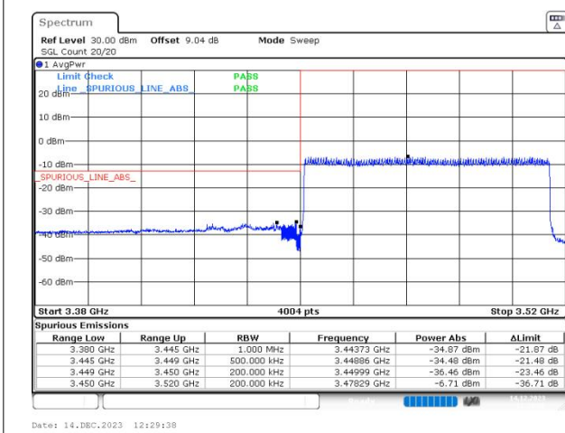
n78(3450-3550) SCS=30kHz DFT_QPSK BW=70MHz LowChannel=632334 RB=180@0
