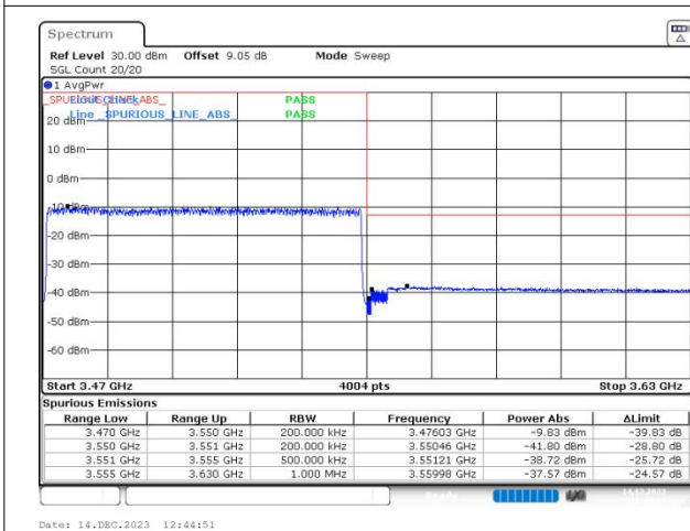
n78(3450-3550) SCS=30kHz DFT_64QAM BW=80MHz HighChannel=634000 RB=216@0
