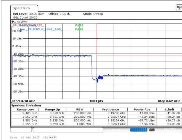
n78(3450-3550) SCS=30kHz DFT_256QAM BW=70MHz HighChannel=634332 RB=180@0
