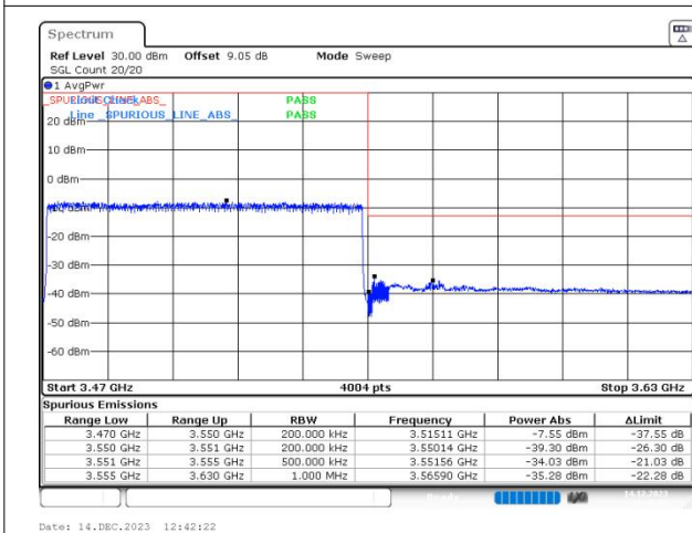
n78(3450-3550) SCS=30kHz DFT_BPSK BW=80MHz HighChannel=634000 RB=216@0
