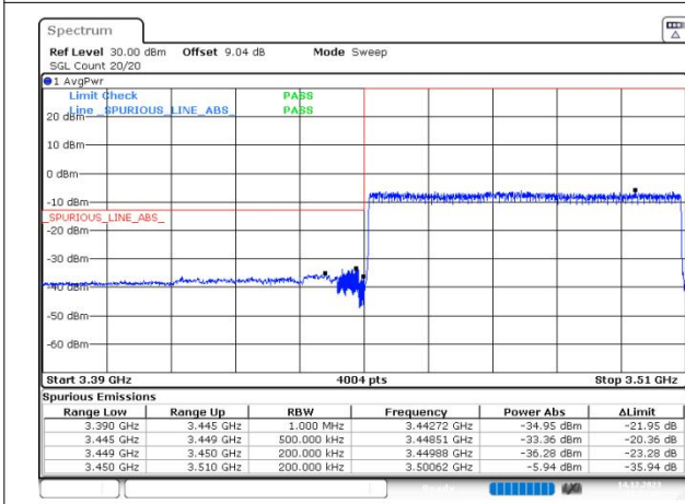
n78(3450-3550) SCS=30kHz DFT_BPSK BW=60MHz LowChannel=632000 RB=162@0
