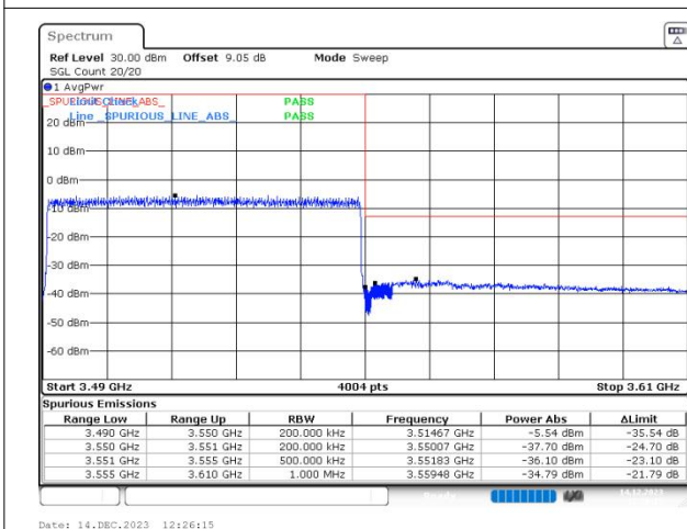
n78(3450-3550) SCS=30kHz DFT_QPSK BW=60MHz HighChannel=634666 RB=162@0
