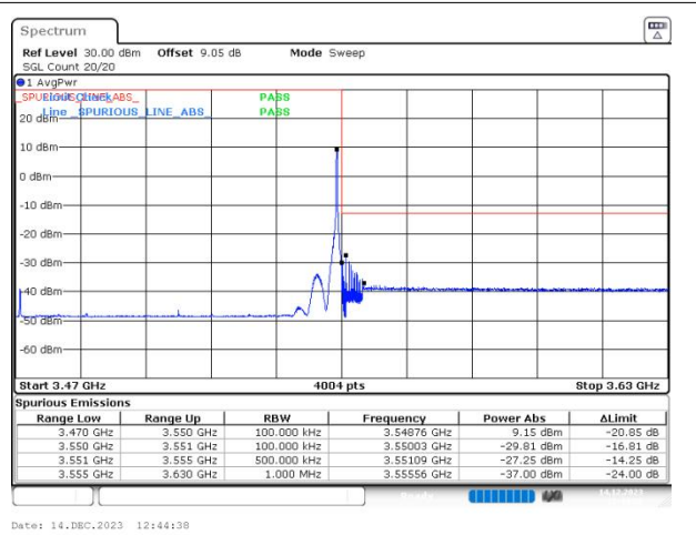
n78(3450-3550) SCS=30kHz DFT_64QAM BW=80MHz HighChannel=634000 RB=1@216
