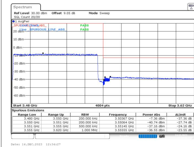
n78(3450-3550) SCS=30kHz DFT_QPSK BW=70MHz HighChannel=634332 RB=180@0
