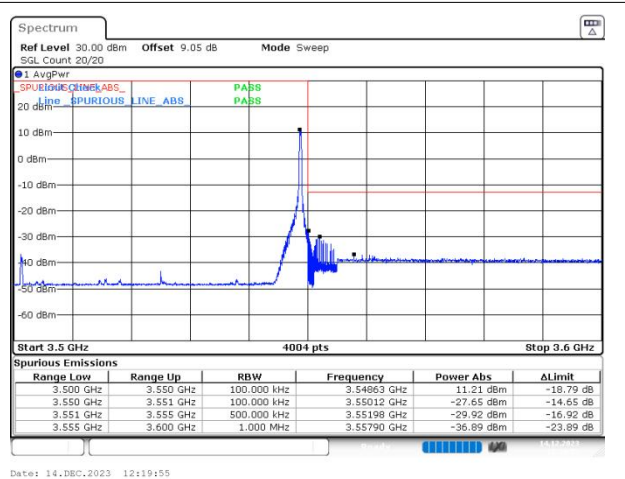
n78(3450-3550) SCS=30kHz DFT_64QAM BW=50MHz HighChannel=635000 RB=1@132
