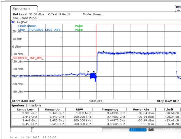
n78(3450-3550) SCS=30kHz DFT_BPSK BW=70MHz LowChannel=632334 RB=180@0
