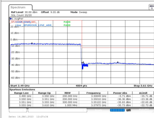
n78(3450-3550) SCS=30kHz DFT_BPSK BW=60MHz HighChannel=634666 RB=162@0
