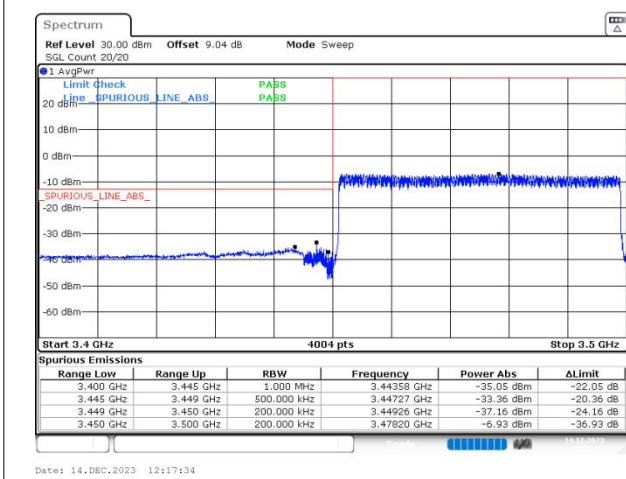
n78(3450-3550) SCS=30kHz CP_QPSK BW=50MHz LowChannel=631668 RB=133@0
