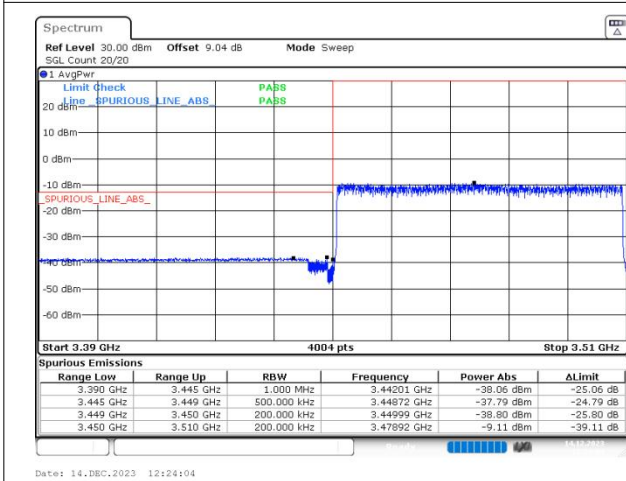
n78(3450-3550) SCS=30kHz DFT_256QAM BW=60MHz LowChannel=632000 RB=162@0
