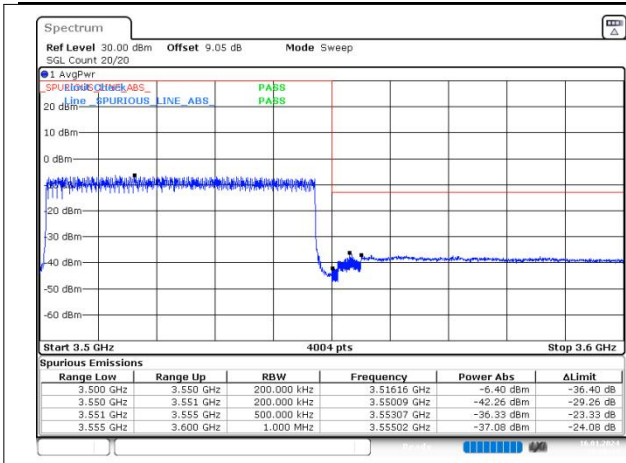
n78(3450-3550) SCS=30kHz DFT_256QAM BW=50MHz HighChannel=635000 RB=128@0
