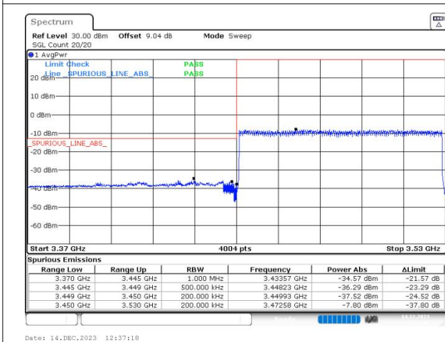
n78(3450-3550) SCS=30kHz DFT_BPSK BW=80MHz LowChannel=632668 RB=216@0
