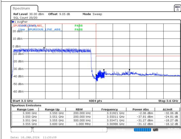
n78(3450-3550) SCS=30kHz DFT_BPSK BW=50MHz HighChannel=635000 RB=128@0
