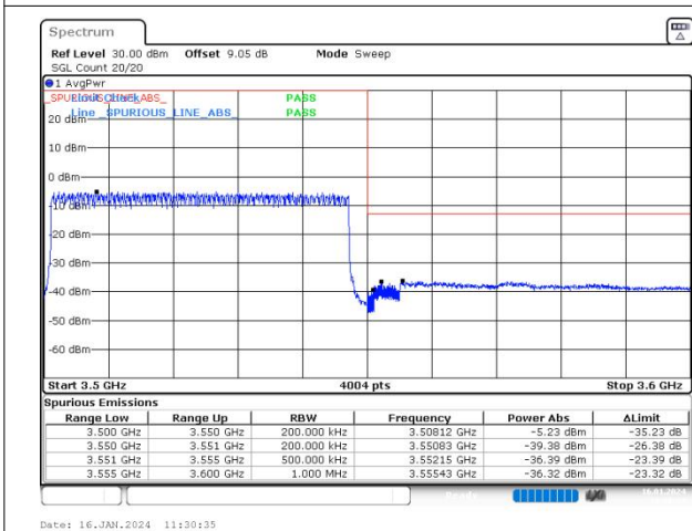
n78(3450-3550) SCS=30kHz DFT_64QAM BW=50MHz HighChannel=635000 RB=128@0
