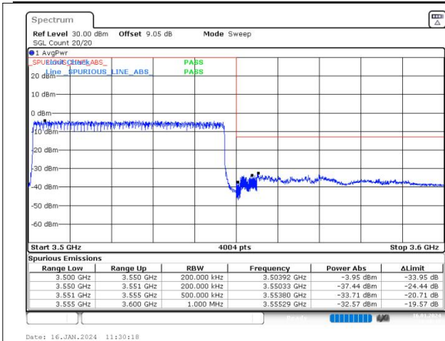
n78(3450-3550) SCS=30kHz DFT_QPSK BW=50MHz HighChannel=635000 RB=128@0
