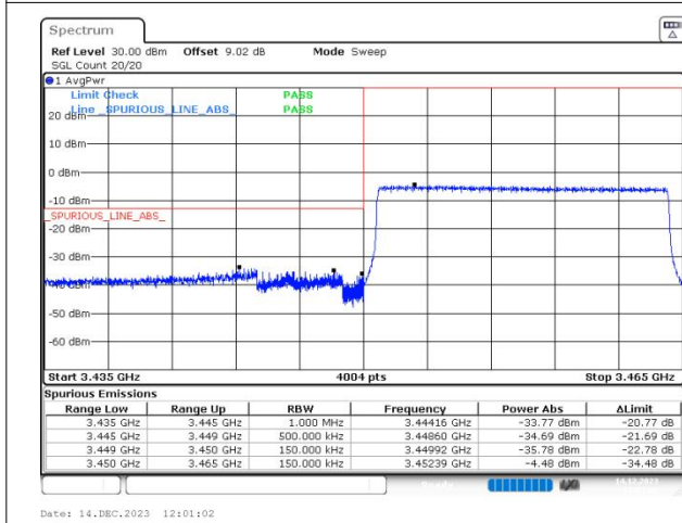
n78(3450-3550) SCS=30kHz CP_QPSK BW=15MHz LowChannel=630500 RB=38@0
