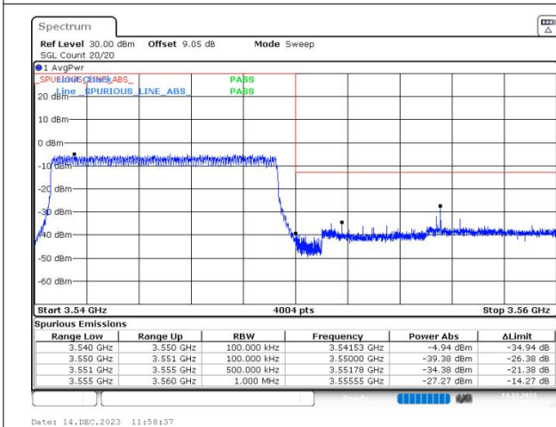
n78(3450-3550) SCS=30kHz DFT_256QAM BW=10MHz HighChannel=636332 RB=24@0
