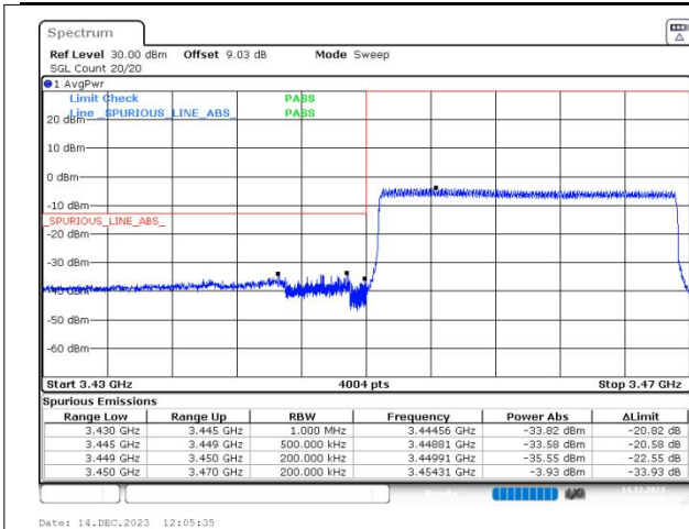
n78(3450-3550) SCS=30kHz CP_QPSK BW=20MHz LowChannel=630668 RB=51@0
