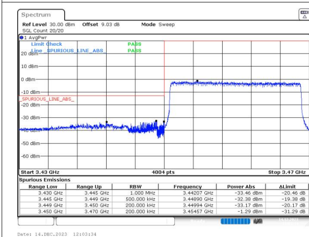
n78(3450-3550) SCS=30kHz DFT_BPSK BW=20MHz LowChannel=630668 RB=50@0
