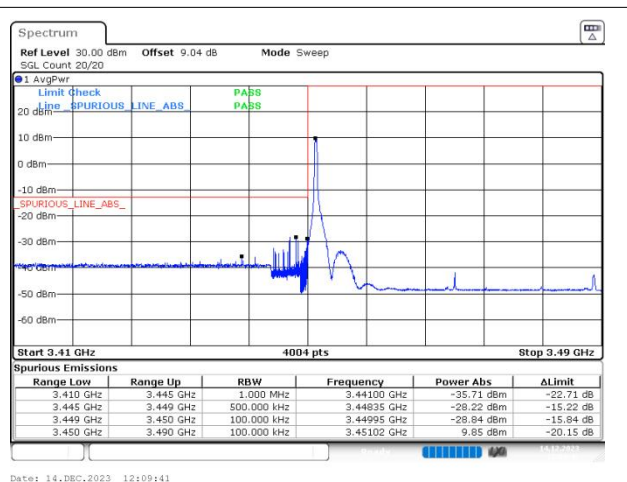
n78(3450-3550) SCS=30kHz DFT_16QAM BW=40MHz LowChannel=631334 RB=1@0
