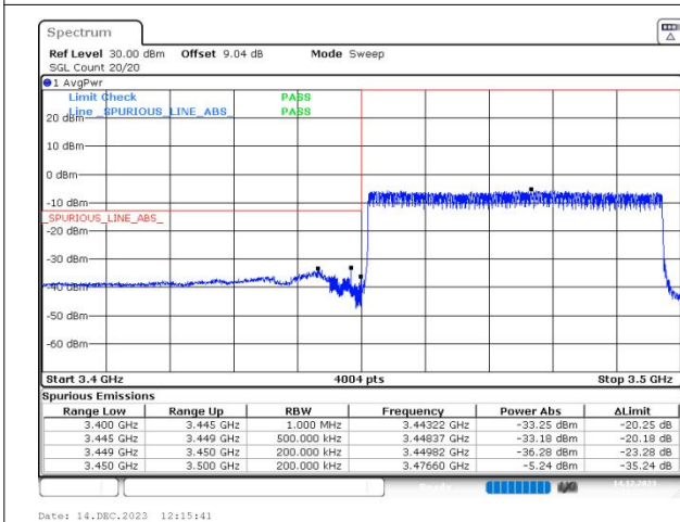
n78(3450-3550) SCS=30kHz DFT_16QAM BW=50MHz LowChannel=631668 RB=128@0
