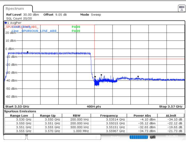
n78(3450-3550) SCS=30kHz DFT_256QAM BW=20MHz HighChannel=636000 RB=1@50
