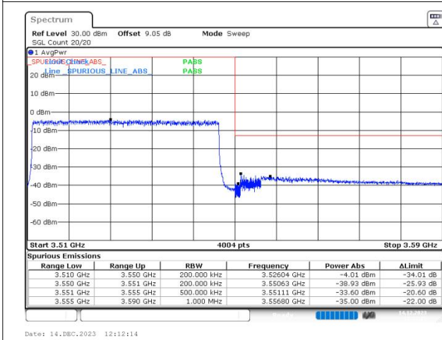
n78(3450-3550) SCS=30kHz DFT_QPSK BW=40MHz HighChannel=635332 RB=100@0
