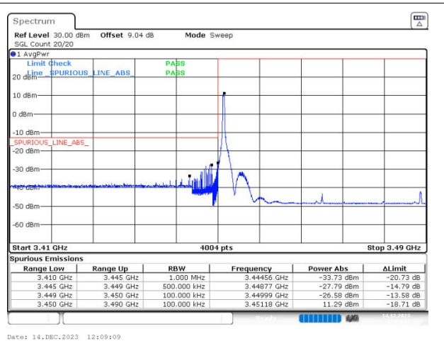
n78(3450-3550) SCS=30kHz DFT_QPSK BW=40MHz LowChannel=631334 RB=1@0
