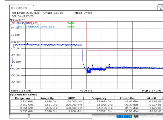
n78(3450-3550) SCS=30kHz DFT_16QAM BW=20MHz HighChannel=636000 RB=50@0
