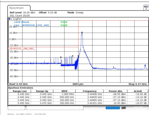
n78(3450-3550) SCS=30kHz CP_QPSK BW=20MHz LowChannel=630668 RB=1@0
