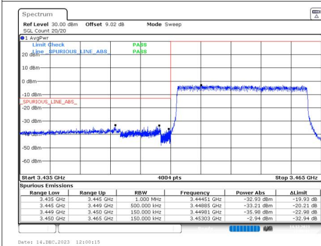
n78(3450-3550) SCS=30kHz DFT_64QAM BW=15MHz LowChannel=630500 RB=36@0
