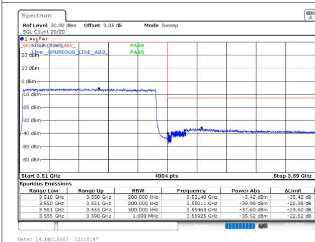
n78(3450-3550) SCS=30kHz DFT_16QAM BW=40MHz HighChannel=635332 RB=100@0
