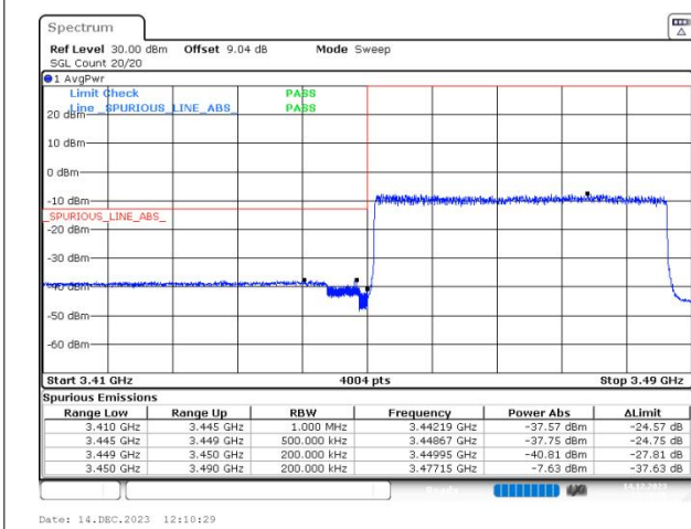
n78(3450-3550) SCS=30kHz DFT_256QAM BW=40MHz LowChannel=631334 RB=100@0
