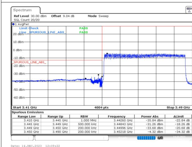
n78(3450-3550) SCS=30kHz DFT_16QAM BW=40MHz LowChannel=631334 RB=100@0
