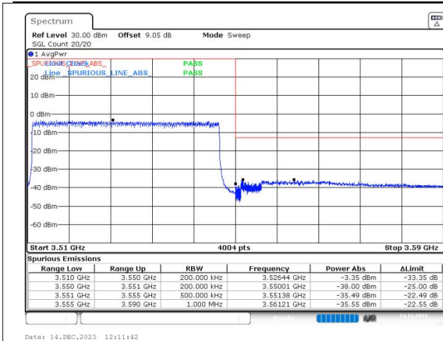
n78(3450-3550) SCS=30kHz DFT_BPSK BW=40MHz HighChannel=635332 RB=100@0
