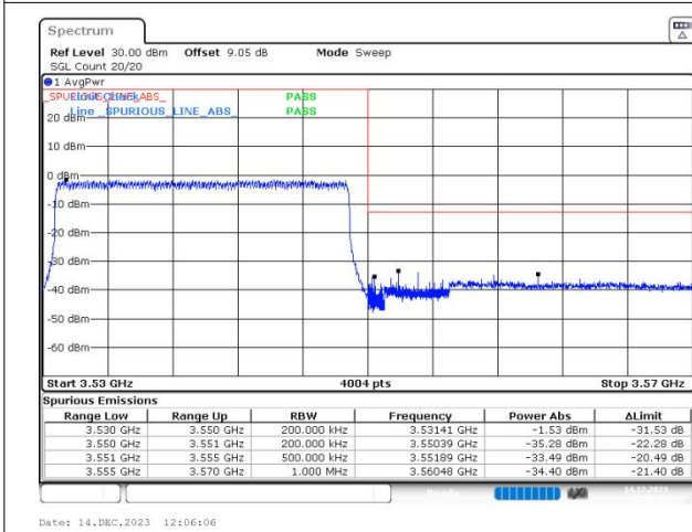
n78(3450-3550) SCS=30kHz DFT_BPSK BW=20MHz HighChannel=636000 RB=50@0
