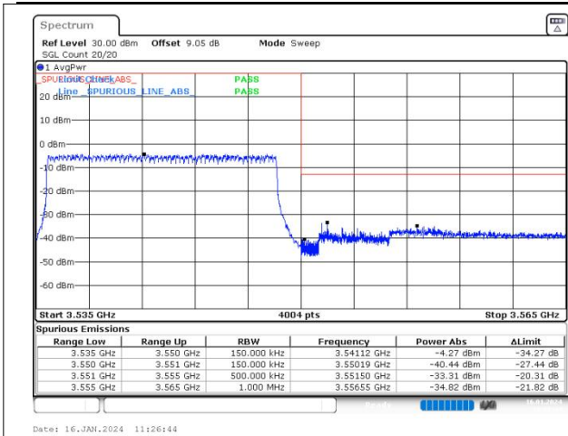
n78(3450-3550) SCS=30kHz DFT_256QAM BW=15MHz HighChannel=636166 RB=36@0
