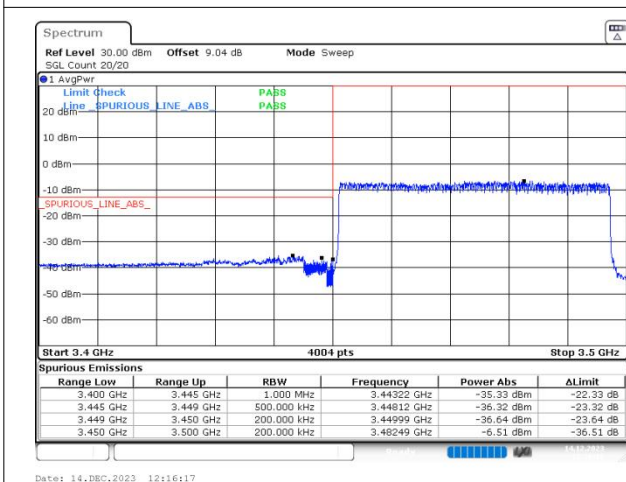
n78(3450-3550) SCS=30kHz DFT_64QAM BW=50MHz LowChannel=631668 RB=128@0
