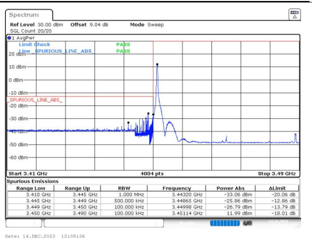
n78(3450-3550) SCS=30kHz DFT_BPSK BW=40MHz LowChannel=631334 RB=1@0
