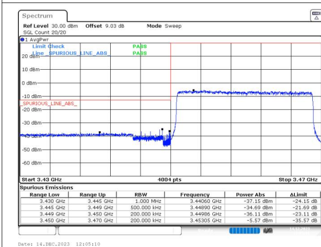
n78(3450-3550) SCS=30kHz DFT_256QAM BW=20MHz LowChannel=630668 RB=50@0
