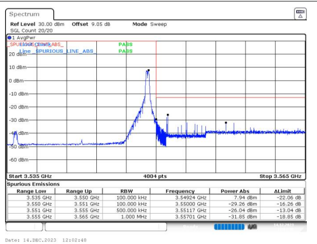
n78(3450-3550) SCS=30kHz DFT_256QAM BW=15MHz HighChannel=636166 RB=1@37
