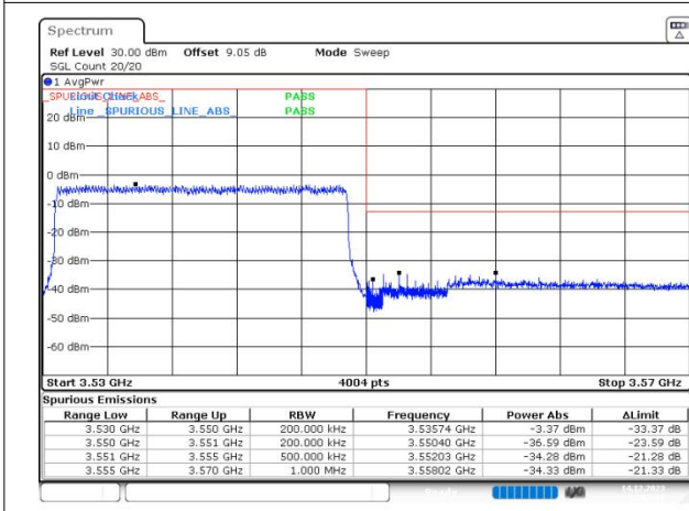
n78(3450-3550) SCS=30kHz DFT_16QAM BW=20MHz HighChannel=636000 RB=50@0
