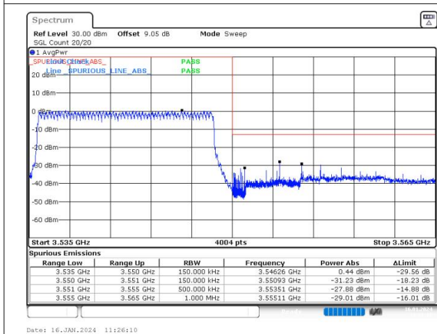
n78(3450-3550) SCS=30kHz DFT_BPSK BW=15MHz HighChannel=636166 RB=36@0
