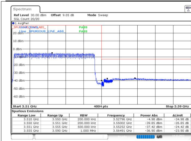
n78(3450-3550) SCS=30kHz DFT_64QAM BW=40MHz HighChannel=635332 RB=100@0
