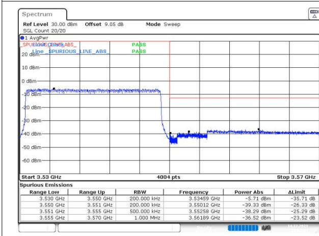
n78(3450-3550) SCS=30kHz DFT_64QAM BW=20MHz HighChannel=636000 RB=50@0
