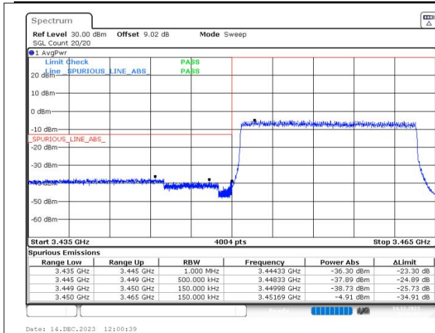
n78(3450-3550) SCS=30kHz DFT_256QAM BW=15MHz LowChannel=630500 RB=36@0
