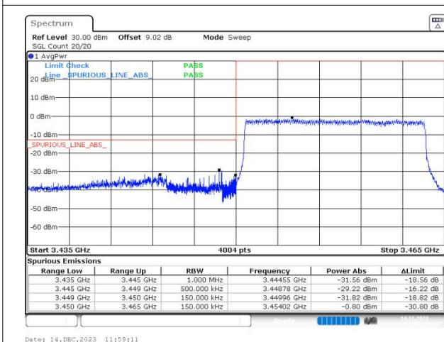
n78(3450-3550) SCS=30kHz DFT_BPSK BW=15MHz LowChannel=630500 RB=36@0
