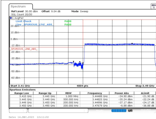
n78(3450-3550) SCS=30kHz CP_QPSK BW=40MHz LowChannel=631334 RB=106@0
