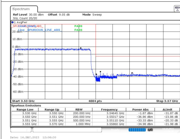
n78(3450-3550) SCS=30kHz DFT_QPSK BW=20MHz HighChannel=636000 RB=50@0
