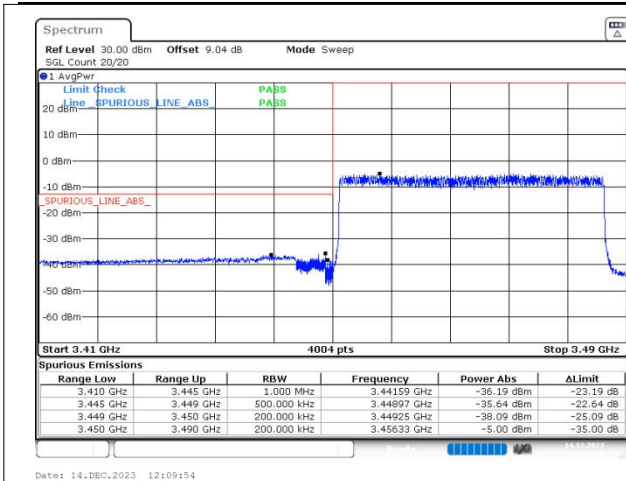
n78(3450-3550) SCS=30kHz DFT_64QAM BW=40MHz LowChannel=631334 RB=100@0
