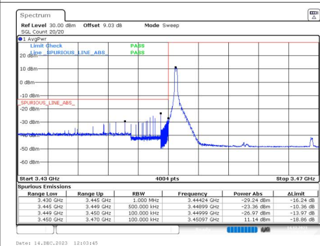
n78(3450-3550) SCS=30kHz DFT_BPSK BW=20MHz LowChannel=630668 RB=1@0
