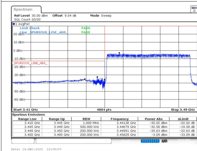
n78(3450-3550) SCS=30kHz DFT_QPSK BW=40MHz LowChannel=631334 RB=100@0
