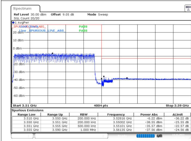
n78(3450-3550) SCS=30kHz DFT_64QAM BW=40MHz HighChannel=635332 RB=100@0
