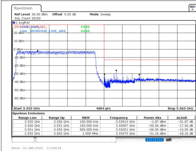
n78(3450-3550) SCS=30kHz DFT_64QAM BW=15MHz HighChannel=636166 RB=36@0
