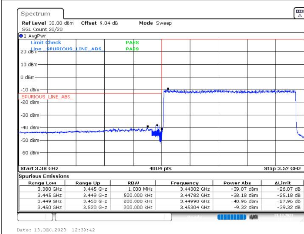
n77(3450-3550) SCS=30kHz DFT_256QAM BW=70MHz LowChannel=632334 RB=180@0
