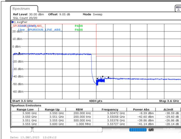
n77(3450-3550) SCS=30kHz DFT_256QAM BW=50MHz HighChannel=635000 RB=128@0
