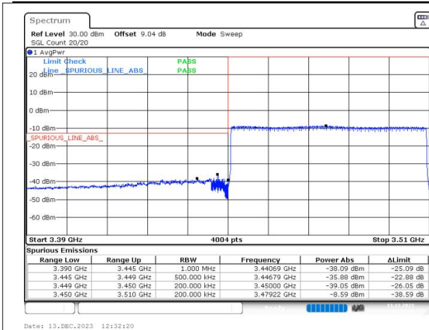
n77(3450-3550) SCS=30kHz CP_QPSK BW=60MHz LowChannel=632000 RB=162@0
