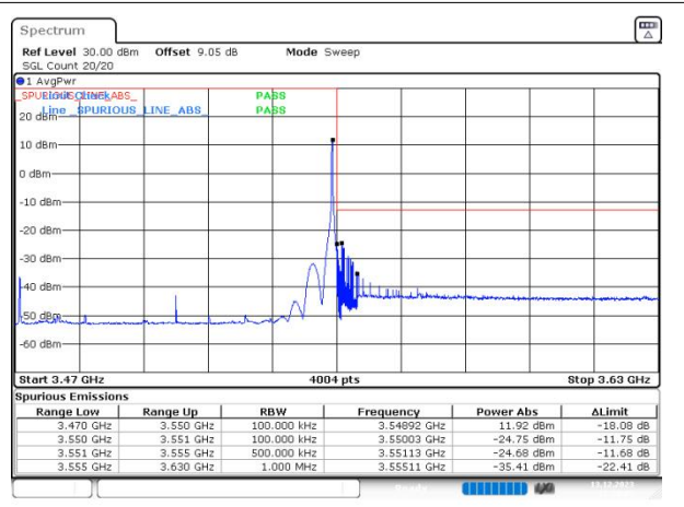
n77(3450-3550) SCS=30kHz DFT_256QAM BW=80MHz LowChannel=632668 RB=1@0
