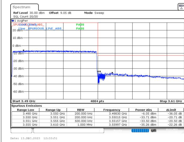
n77(3450-3550) SCS=30kHz DFT_QPSK BW=60MHz HighChannel=634666 RB=162@0
