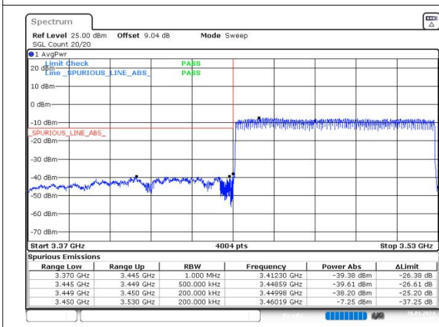
n77(3450-3550) SCS=30kHz DFT_16QAM BW=80MHz LowChannel=632668 RB=216@0
