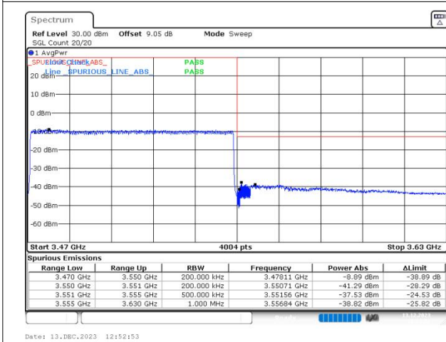
n77(3450-3550) SCS=30kHz DFT_64QAM BW=80MHz HighChannel=634000 RB=216@0
