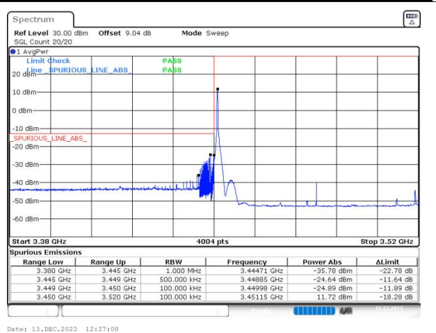
n77(3450-3550) SCS=30kHz DFT_BPSK BW=70MHz LowChannel=632334 RB=1@0
