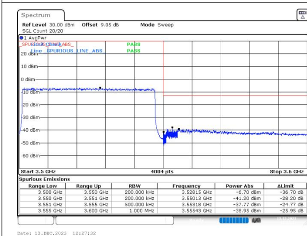
n77(3450-3550) SCS=30kHz DFT_64QAM BW=50MHz HighChannel=635000 RB=128@0
