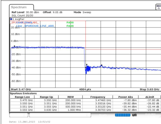
n77(3450-3550) SCS=30kHz DFT_16QAM BW=80MHz HighChannel=634000 RB=216@0
