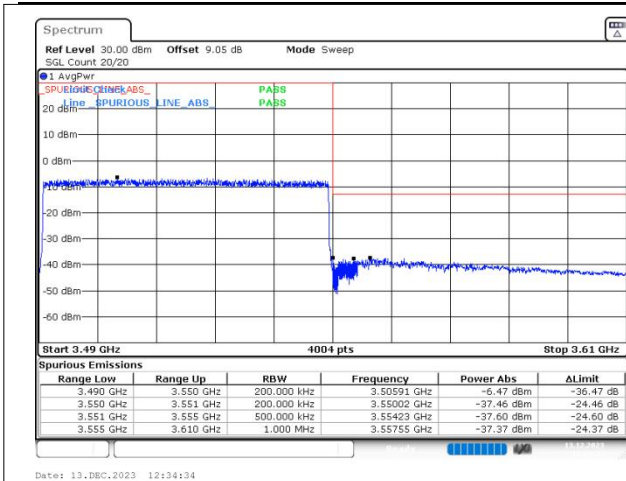
n77(3450-3550) SCS=30kHz DFT_16QAM BW=60MHz HighChannel=634666 RB=162@0
