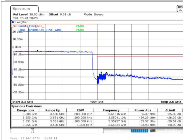
n77(3450-3550) SCS=30kHz DFT_QPSK BW=50MHz HighChannel=635000 RB=128@0
