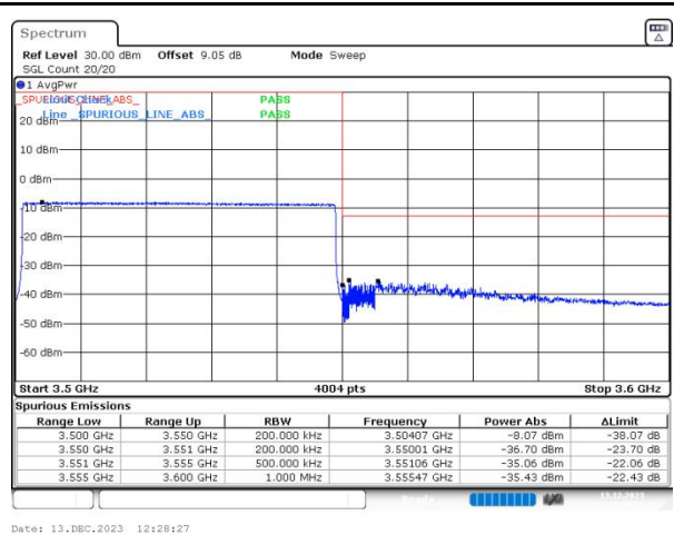
n77(3450-3550) SCS=30kHz CP_QPSK BW=50MHz HighChannel=635000 RB=133@0
