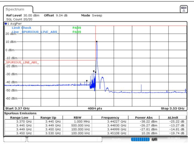
n77(3450-3550) SCS=30kHz DFT_QPSK BW=80MHz LowChannel=632668 RB=1@0
