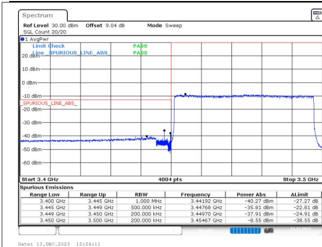
n77(3450-3550) SCS=30kHz DFT_256QAM BW=50MHz LowChannel=631668 RB=128@0
