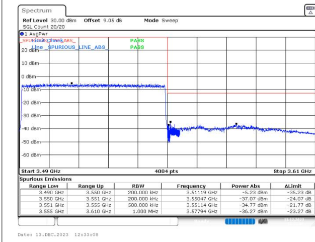
n77(3450-3550) SCS=30kHz DFT_BPSK BW=60MHz HighChannel=634666 RB=162@0
