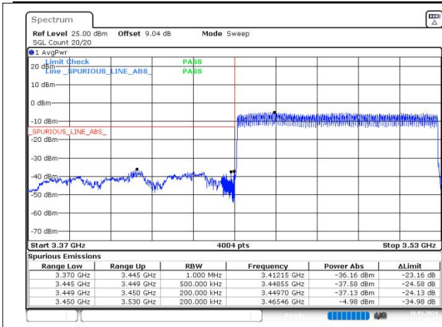
n77(3450-3550) SCS=30kHz DFT_QPSK BW=80MHz LowChannel=632668 RB=216@0
