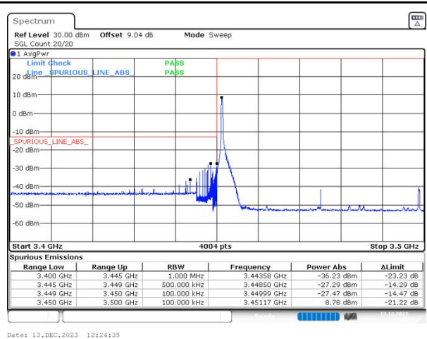
n77(3450-3550) SCS=30kHz DFT_256QAM BW=50MHz LowChannel=631668 RB=1@0
