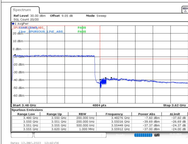
n77(3450-3550) SCS=30kHz DFT_16QAM BW=70MHz HighChannel=634332 RB=180@0
