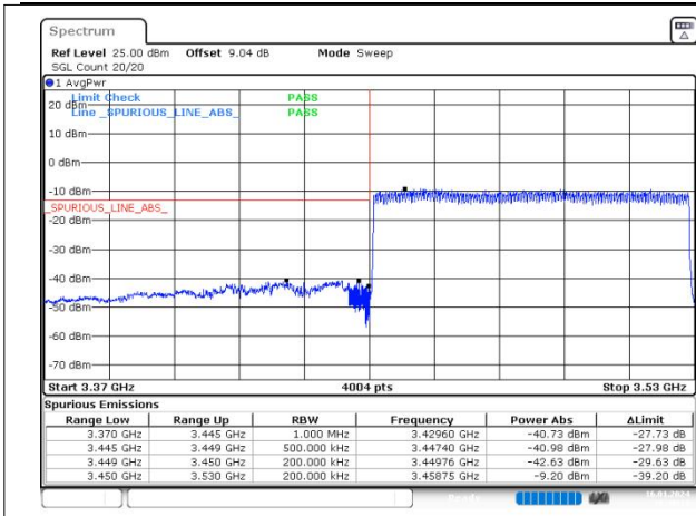
n77(3450-3550) SCS=30kHz DFT_256QAM BW=80MHz LowChannel=632668 RB=216@0
