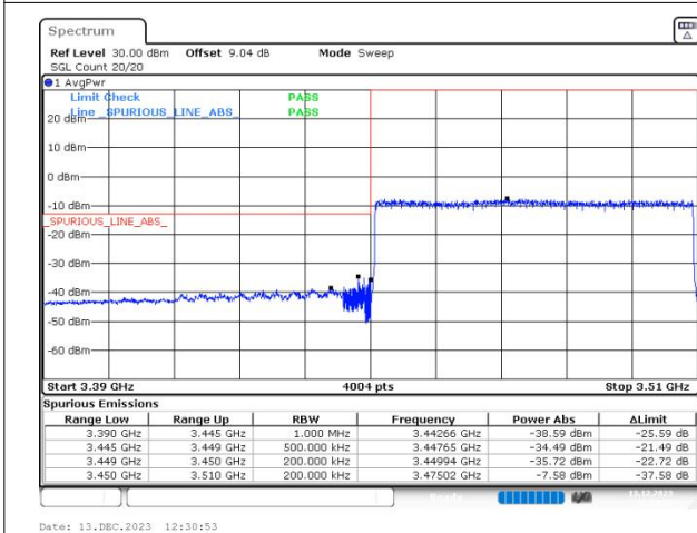
n77(3450-3550) SCS=30kHz DFT_64QAM BW=60MHz LowChannel=632000 RB=162@0
