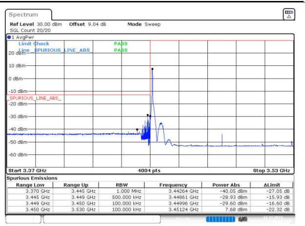
n77(3450-3550) SCS=30kHz DFT_256QAM BW=80MHz LowChannel=632668 RB=1@0
