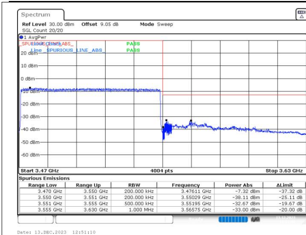
n77(3450-3550) SCS=30kHz DFT_QPSK BW=80MHz HighChannel=634000 RB=216@0
