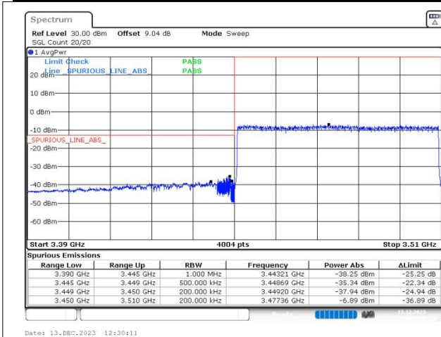
n77(3450-3550) SCS=30kHz DFT_16QAM BW=60MHz LowChannel=632000 RB=162@0
