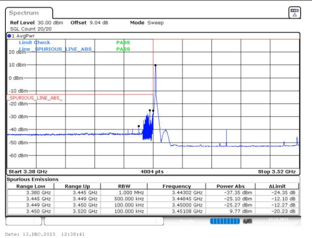
n77(3450-3550) SCS=30kHz DFT_16QAM BW=70MHz LowChannel=632334 RB=1@0
