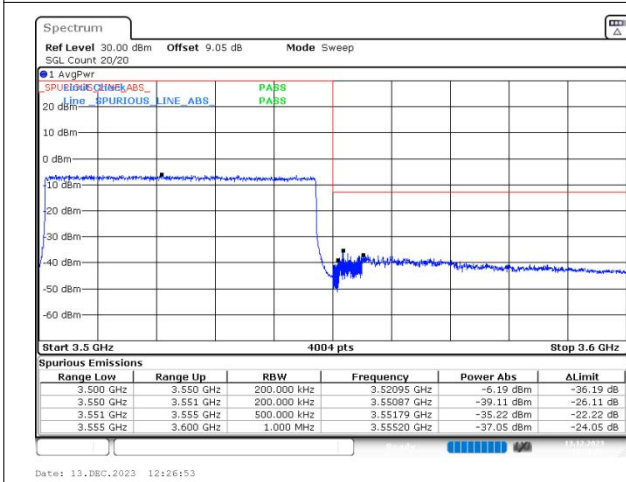
n77(3450-3550) SCS=30kHz DFT_16QAM BW=50MHz HighChannel=635000 RB=128@0
