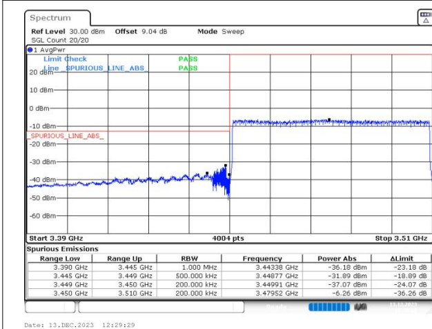
n77(3450-3550) SCS=30kHz DFT_QPSK BW=60MHz LowChannel=632000 RB=162@0
