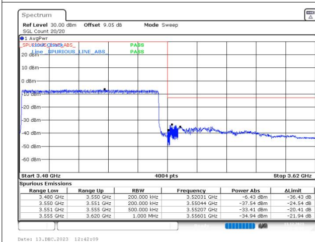
n77(3450-3550) SCS=30kHz DFT_QPSK BW=70MHz HighChannel=634332 RB=180@0
