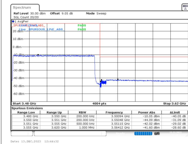
n77(3450-3550) SCS=30kHz DFT_256QAM BW=70MHz HighChannel=634332 RB=180@0
