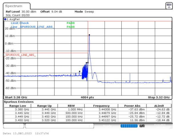
n77(3450-3550) SCS=30kHz DFT_QPSK BW=70MHz LowChannel=632334 RB=1@0
