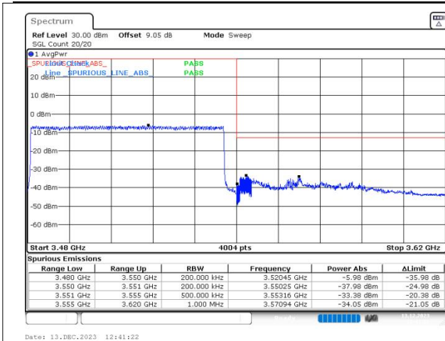
n77(3450-3550) SCS=30kHz DFT_BPSK BW=70MHz HighChannel=634332 RB=180@0
