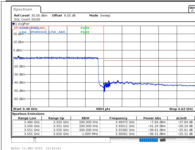
n77(3450-3550) SCS=30kHz DFT_64QAM BW=70MHz HighChannel=634332 RB=180@0
