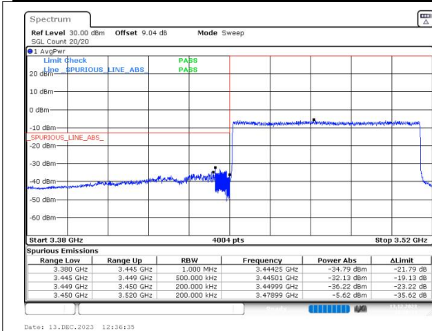
n77(3450-3550) SCS=30kHz DFT_BPSK BW=70MHz LowChannel=632334 RB=180@0
