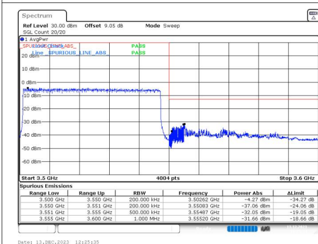
n77(3450-3550) SCS=30kHz DFT_BPSK BW=50MHz HighChannel=635000 RB=128@0
