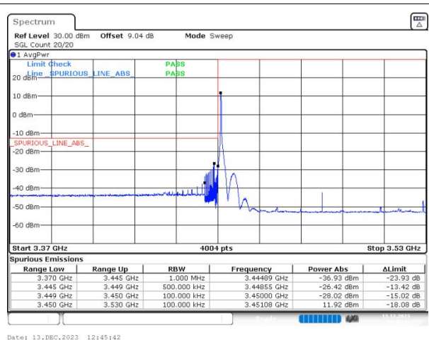
n77(3450-3550) SCS=30kHz DFT_BPSK BW=80MHz LowChannel=632668 RB=1@0
