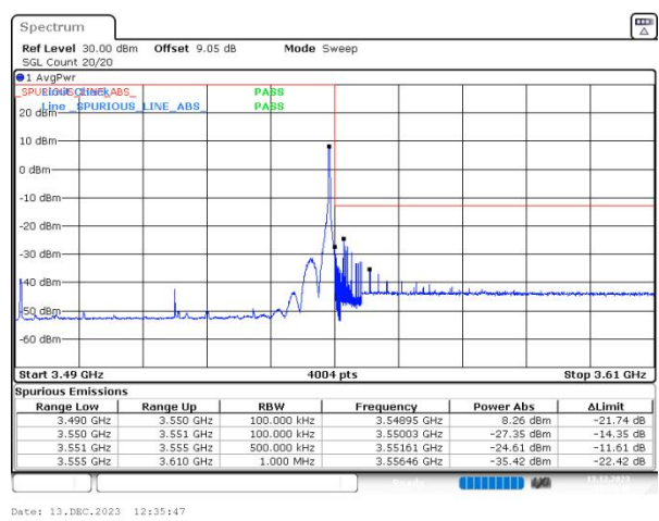
n77(3450-3550) SCS=30kHz DFT_256QAM BW=60MHz HighChannel=634666 RB=1@161
