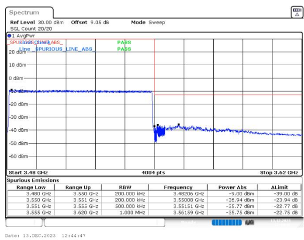
n77(3450-3550) SCS=30kHz CP_QPSK BW=70MHz HighChannel=634332 RB=189@0
