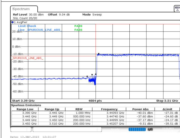
n77(3450-3550) SCS=30kHz DFT_256QAM BW=60MHz LowChannel=632000 RB=162@0
