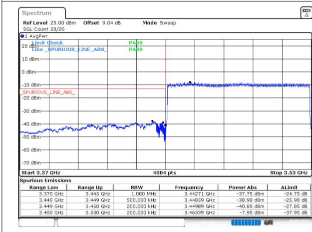
n77(3450-3550) SCS=30kHz DFT_256QAM BW=80MHz LowChannel=632668 RB=216@0
