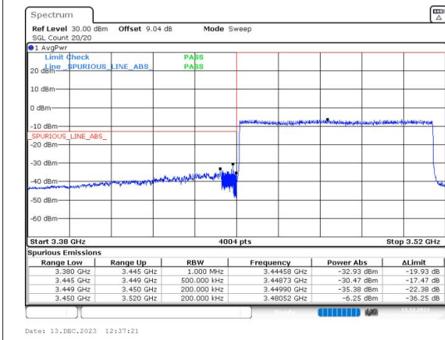
n77(3450-3550) SCS=30kHz DFT_QPSK BW=70MHz LowChannel=632334 RB=180@0
