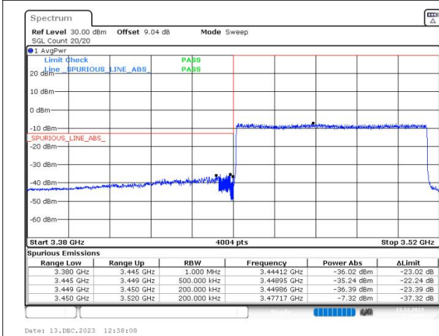
n77(3450-3550) SCS=30kHz DFT_16QAM BW=70MHz LowChannel=632334 RB=180@0
