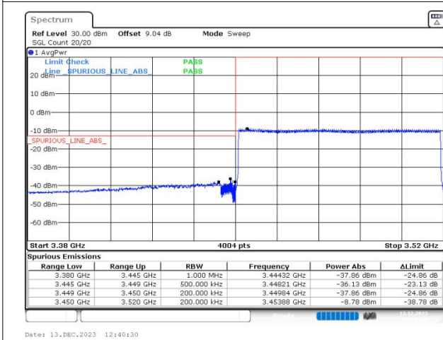
n77(3450-3550) SCS=30kHz CP_QPSK BW=70MHz LowChannel=632334 RB=189@0
