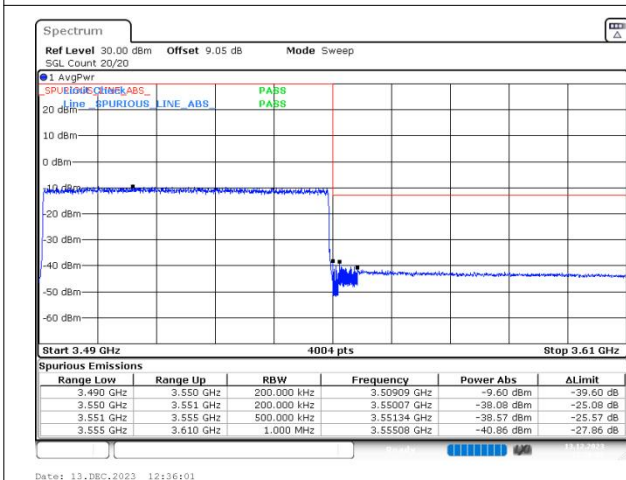
n77(3450-3550) SCS=30kHz DFT_256QAM BW=60MHz HighChannel=634666 RB=162@0
