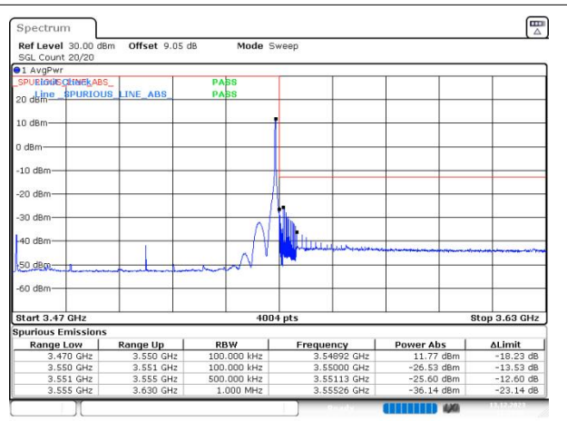
n77(3450-3550) SCS=30kHz DFT_BPSK BW=80MHz HighChannel=634000 RB=1@216
