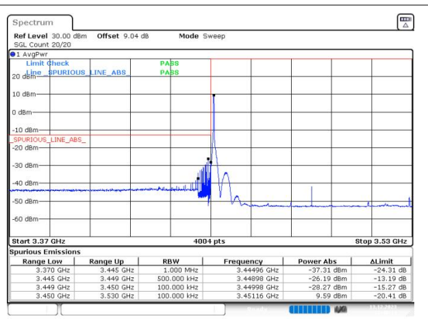
n77(3450-3550) SCS=30kHz DFT_16QAM BW=80MHz LowChannel=632668 RB=1@0
