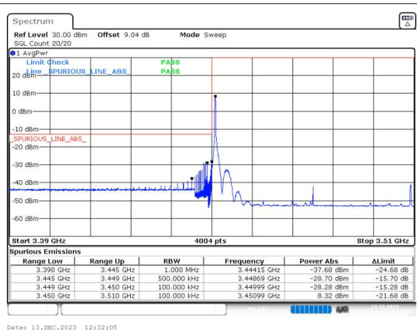
n77(3450-3550) SCS=30kHz DFT_256QAM BW=60MHz LowChannel=632000 RB=1@0
