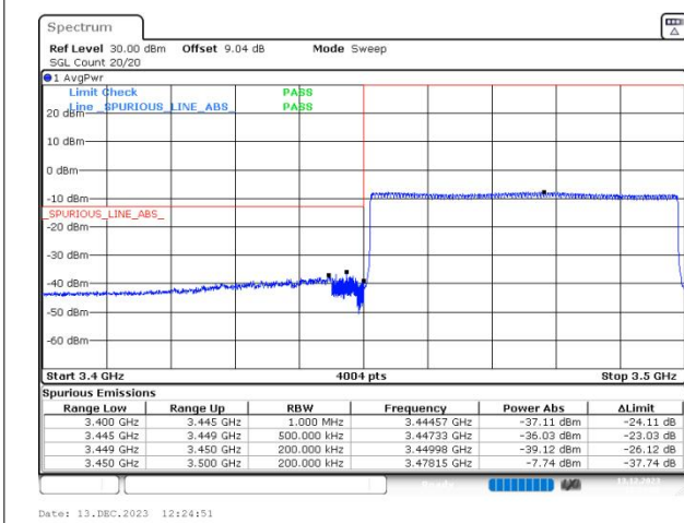
n77(3450-3550) SCS=30kHz CP_QPSK BW=50MHz LowChannel=631668 RB=133@0
