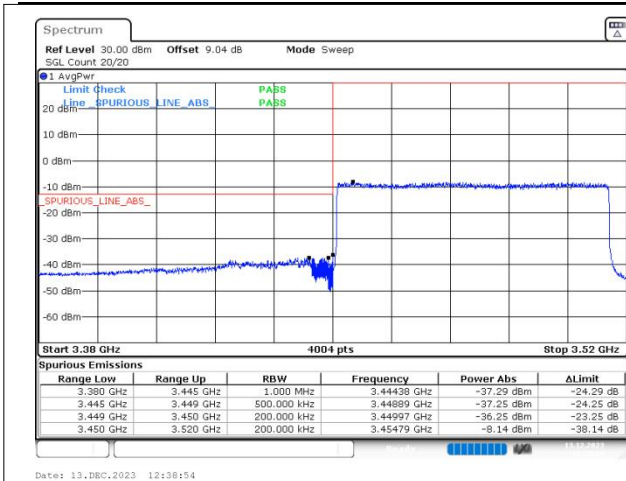
n77(3450-3550) SCS=30kHz DFT_64QAM BW=70MHz LowChannel=632334 RB=180@0
