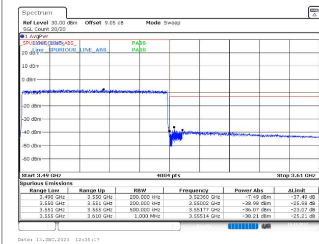
n77(3450-3550) SCS=30kHz DFT_64QAM BW=60MHz HighChannel=634666 RB=162@0
