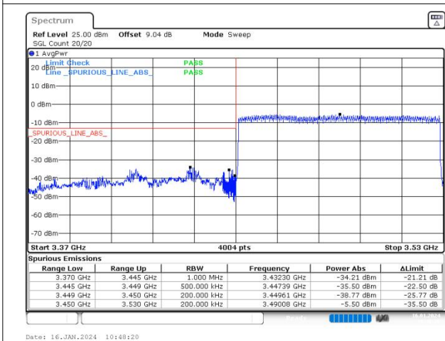
n77(3450-3550) SCS=30kHz DFT_BPSK BW=80MHz LowChannel=632668 RB=216@0
