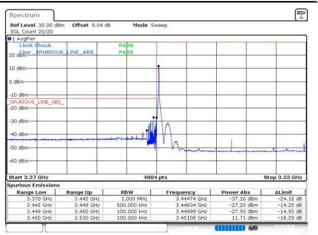
n77(3450-3550) SCS=30kHz DFT_QPSK BW=80MHz LowChannel=632668 RB=1@0
