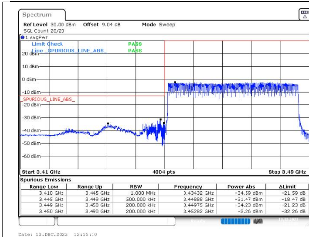
n77(3450-3550) SCS=30kHz DFT_BPSK BW=40MHz LowChannel=631334 RB=100@0
