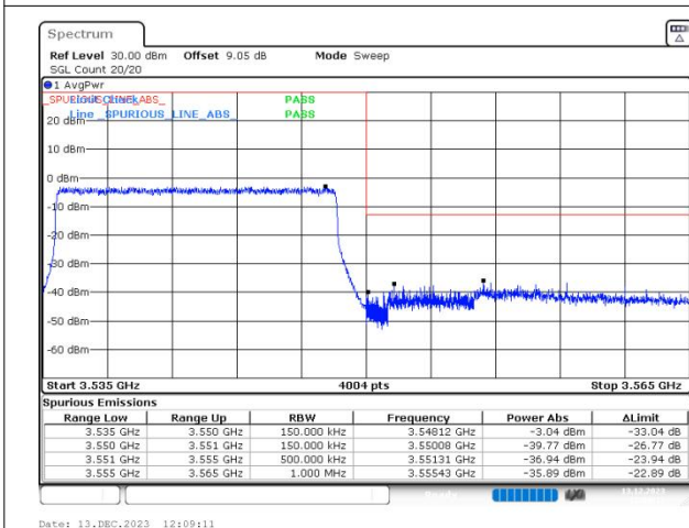
n77(3450-3550) SCS=30kHz DFT_64QAM BW=15MHz HighChannel=636166 RB=36@0
