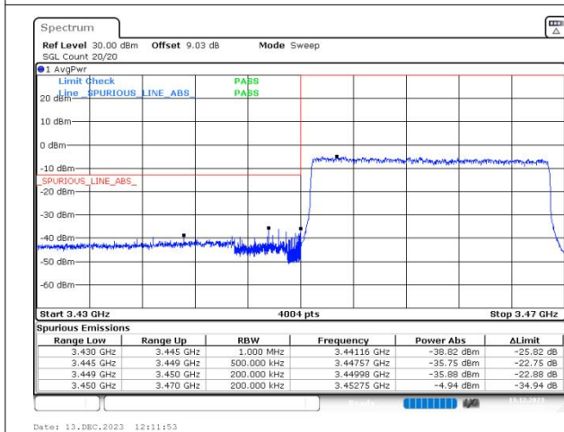
n77(3450-3550) SCS=30kHz DFT_256QAM BW=20MHz LowChannel=630668 RB=50@0
