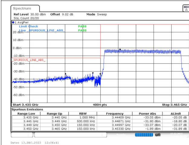
n77(3450-3550) SCS=30kHz DFT_64QAM BW=15MHz LowChannel=630500 RB=36@0
