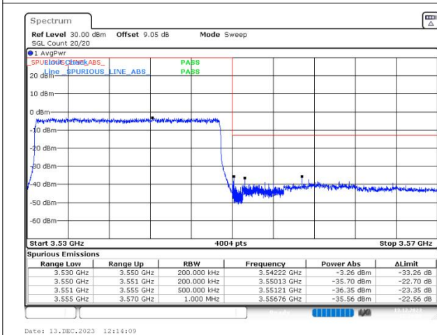
n77(3450-3550) SCS=30kHz DFT_64QAM BW=20MHz HighChannel=636000 RB=50@0
