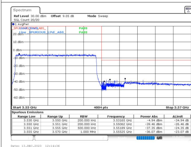
n77(3450-3550) SCS=30kHz DFT_256QAM BW=20MHz HighChannel=636000 RB=50@0
