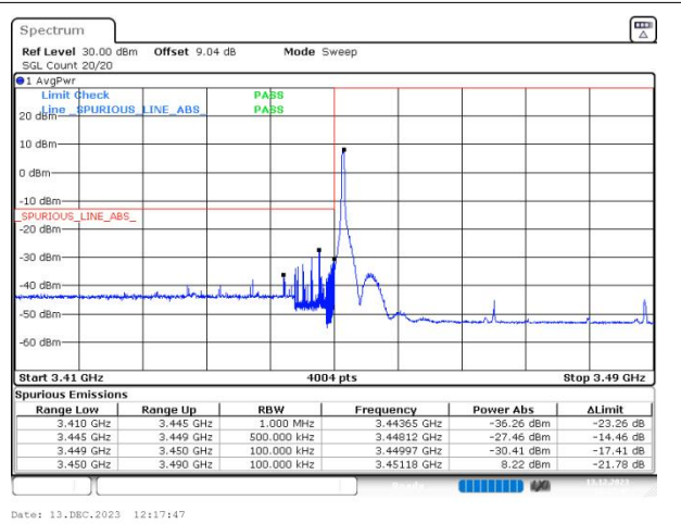
n77(3450-3550) SCS=30kHz DFT_256QAM BW=40MHz LowChannel=631334 RB=1@0
