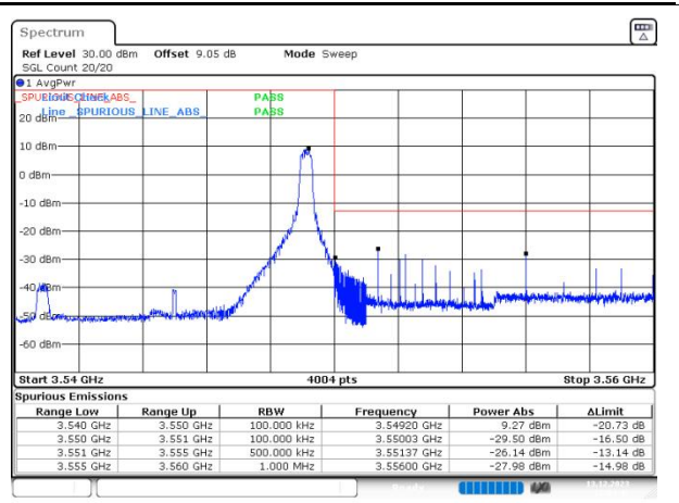
n77(3450-3550) SCS=30kHz DFT_256QAM BW=10MHz HighChannel=636332 RB=1@23
