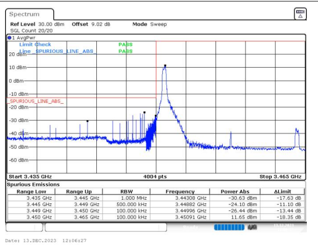
n77(3450-3550) SCS=30kHz DFT_16QAM BW=15MHz LowChannel=630500 RB=1@0
