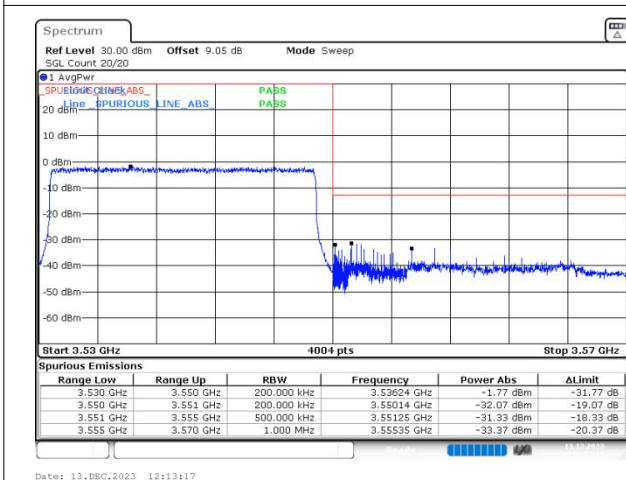
n77(3450-3550) SCS=30kHz DFT_QPSK BW=20MHz HighChannel=636000 RB=50@0
