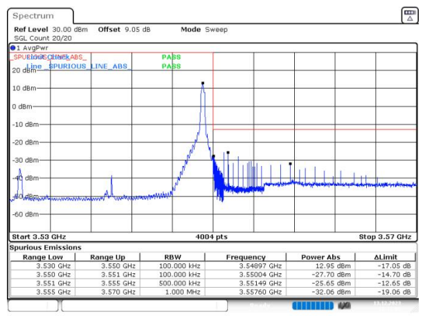
n77(3450-3550) SCS=30kHz DFT_BPSK BW=20MHz HighChannel=636000 RB=1@50
