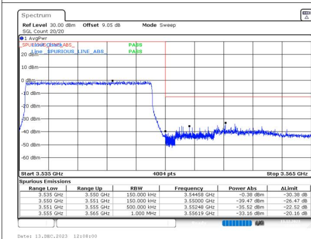
n77(3450-3550) SCS=30kHz DFT_BPSK BW=15MHz HighChannel=636166 RB=36@0
