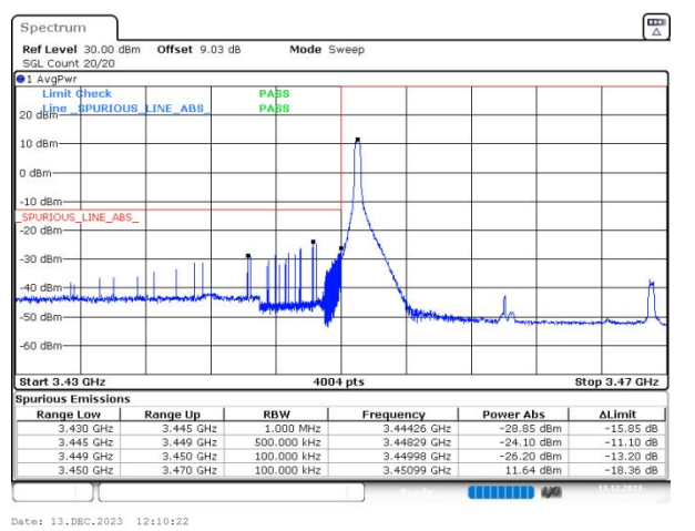
n77(3450-3550) SCS=30kHz DFT_BPSK BW=20MHz LowChannel=630668 RB=1@0
