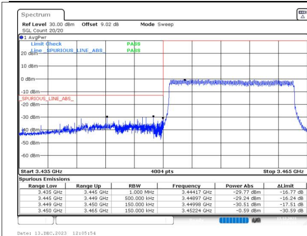
n77(3450-3550) SCS=30kHz DFT_QPSK BW=15MHz LowChannel=630500 RB=36@0
