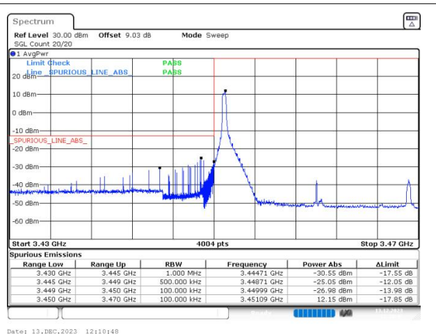
n77(3450-3550) SCS=30kHz DFT_QPSK BW=20MHz LowChannel=630668 RB=1@0
