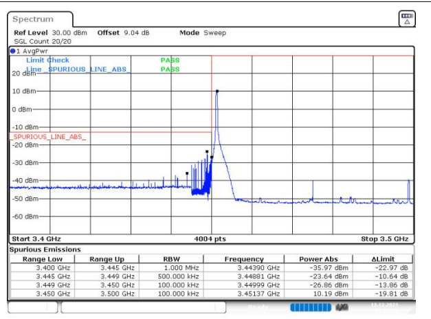
n77(3450-3550) SCS=30kHz DFT_QPSK BW=50MHz LowChannel=631668 RB=1@0
