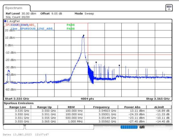
n77(3450-3550) SCS=30kHz DFT_BPSK BW=15MHz HighChannel=636166 RB=1@37
