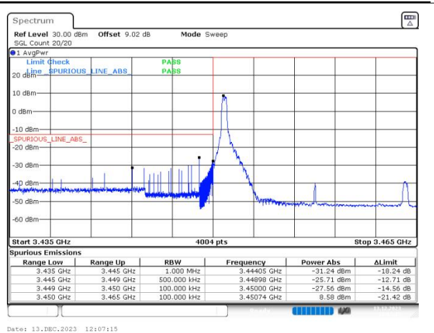
n77(3450-3550) SCS=30kHz DFT_256QAM BW=15MHz LowChannel=630500 RB=1@0
