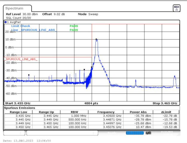
n77(3450-3550) SCS=30kHz DFT_64QAM BW=15MHz LowChannel=630500 RB=1@0
