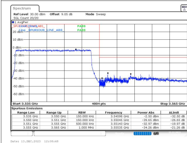
n77(3450-3550) SCS=30kHz DFT_16QAM BW=15MHz HighChannel=636166 RB=36@0
