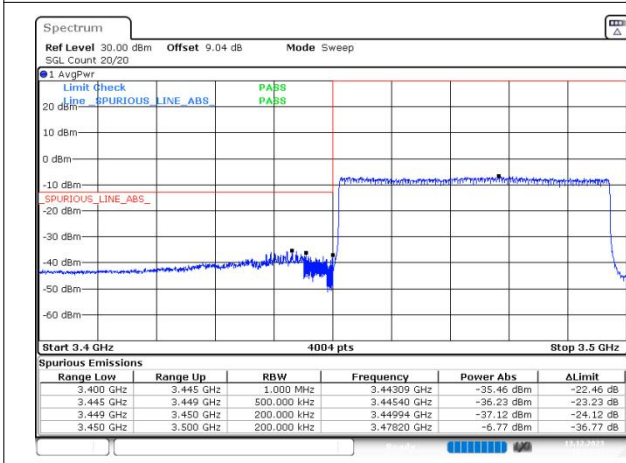
n77(3450-3550) SCS=30kHz DFT_16QAM BW=50MHz LowChannel=631668 RB=128@0
