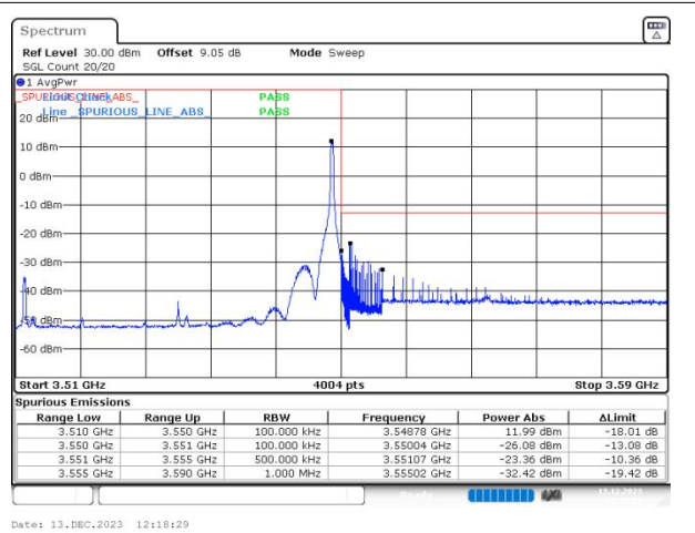
n77(3450-3550) SCS=30kHz DFT_BPSK BW=40MHz HighChannel=635332 RB=1@105
