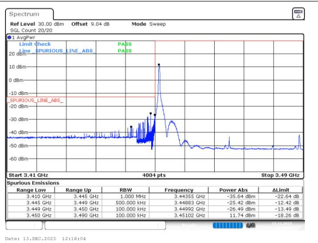
n77(3450-3550) SCS=30kHz DFT_QPSK BW=40MHz LowChannel=631334 RB=1@0
