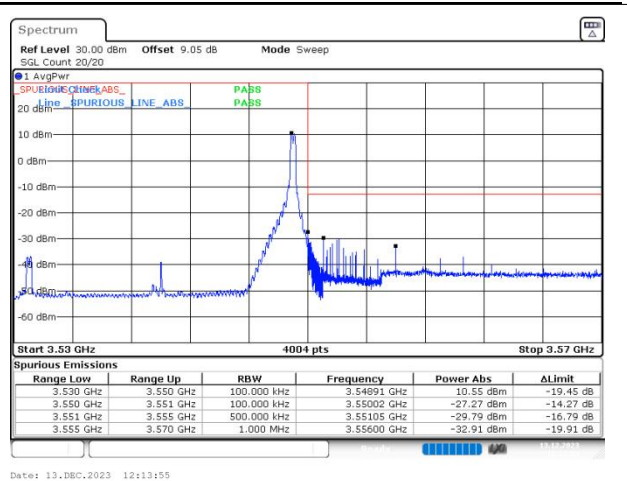
n77(3450-3550) SCS=30kHz DFT_64QAM BW=20MHz HighChannel=636000 RB=1@50
