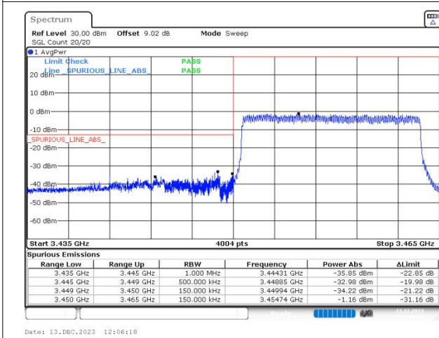
n77(3450-3550) SCS=30kHz DFT_16QAM BW=15MHz LowChannel=630500 RB=36@0
