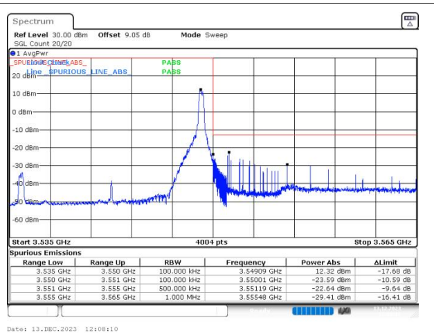
n77(3450-3550) SCS=30kHz DFT_QPSK BW=15MHz HighChannel=636166 RB=1@37
