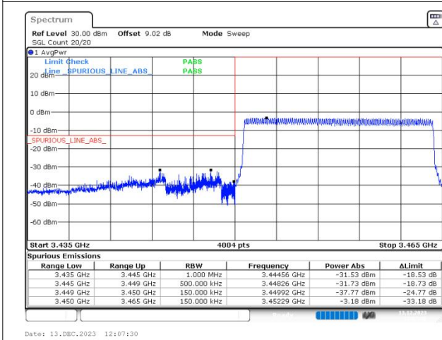
n77(3450-3550) SCS=30kHz CP_QPSK BW=15MHz LowChannel=630500 RB=38@0
