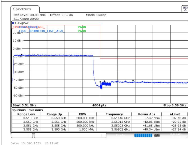
n77(3450-3550) SCS=30kHz DFT_256QAM BW=40MHz HighChannel=635332 RB=100@0
