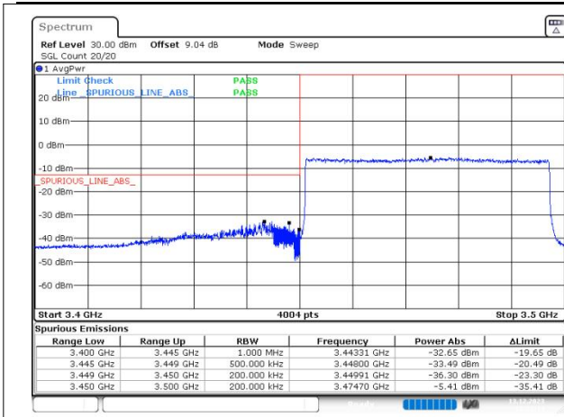
n77(3450-3550) SCS=30kHz DFT_QPSK BW=50MHz LowChannel=631668 RB=128@0
