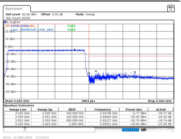
n77(3450-3550) SCS=30kHz CP_QPSK BW=15MHz HighChannel=636166 RB=38@0
