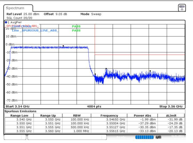
n77(3450-3550) SCS=30kHz DFT_256QAM BW=10MHz HighChannel=636332 RB=1@23
