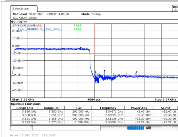
n77(3450-3550) SCS=30kHz DFT_16QAM BW=20MHz HighChannel=636000 RB=50@0
