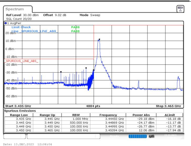
n77(3450-3550) SCS=30kHz DFT_QPSK BW=15MHz LowChannel=630500 RB=1@0
