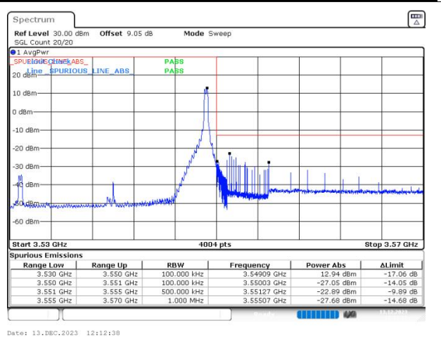
n77(3450-3550) SCS=30kHz DFT_BPSK BW=20MHz HighChannel=636000 RB=1@50
