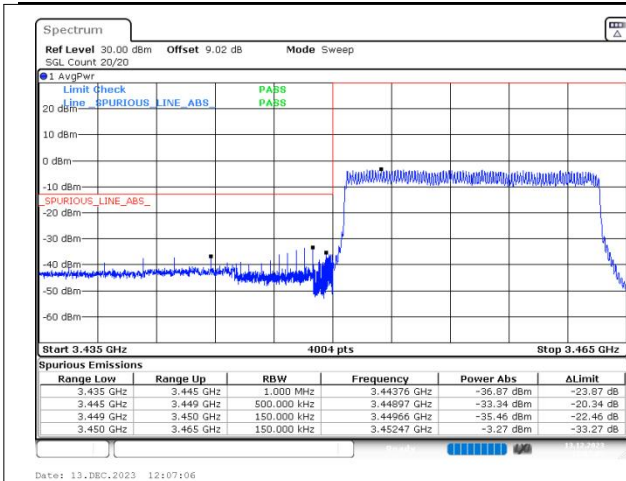
n77(3450-3550) SCS=30kHz DFT_256QAM BW=15MHz LowChannel=630500 RB=36@0
