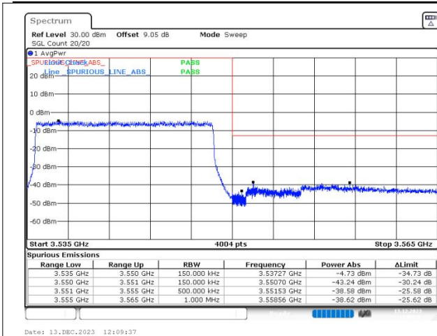
n77(3450-3550) SCS=30kHz DFT_256QAM BW=15MHz HighChannel=636166 RB=36@0
