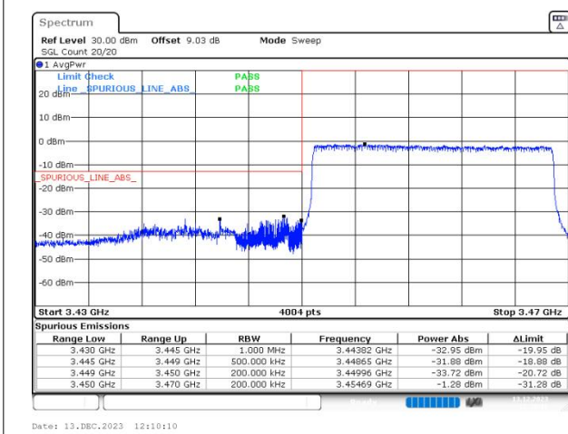
n77(3450-3550) SCS=30kHz DFT_BPSK BW=20MHz LowChannel=630668 RB=50@0
