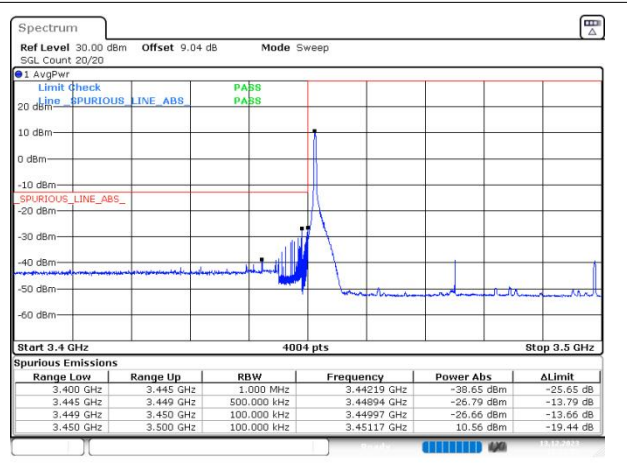
n77(3450-3550) SCS=30kHz DFT_16QAM BW=50MHz LowChannel=631668 RB=1@0
