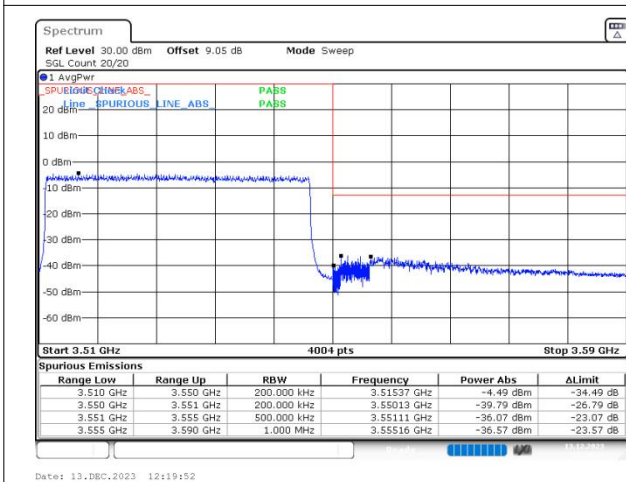
n77(3450-3550) SCS=30kHz DFT_16QAM BW=40MHz HighChannel=635332 RB=100@0
