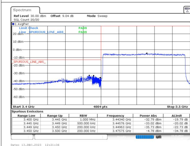
n77(3450-3550) SCS=30kHz DFT_BPSK BW=50MHz LowChannel=631668 RB=128@0
