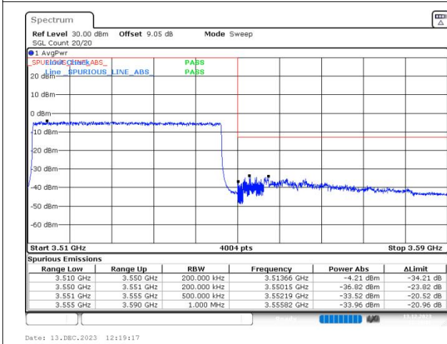
n77(3450-3550) SCS=30kHz DFT_QPSK BW=40MHz HighChannel=635332 RB=100@0
