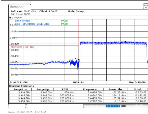
n77(3450-3550) SCS=30kHz CP_QPSK BW=40MHz LowChannel=631334 RB=106@0
