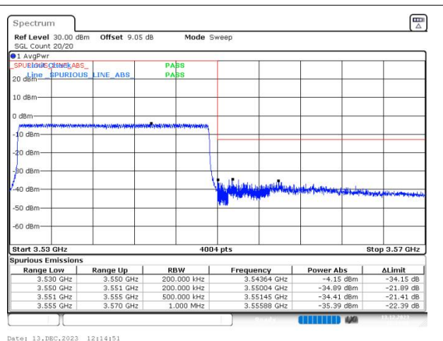
n77(3450-3550) SCS=30kHz CP_QPSK BW=20MHz HighChannel=636000 RB=51@0
