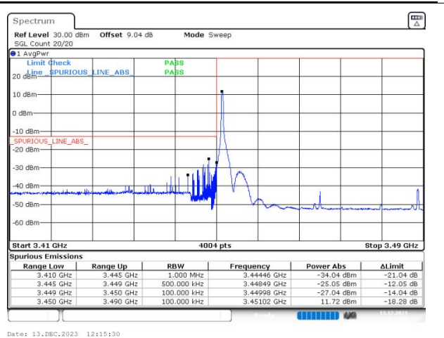
n77(3450-3550) SCS=30kHz DFT_BPSK BW=40MHz LowChannel=631334 RB=1@0
