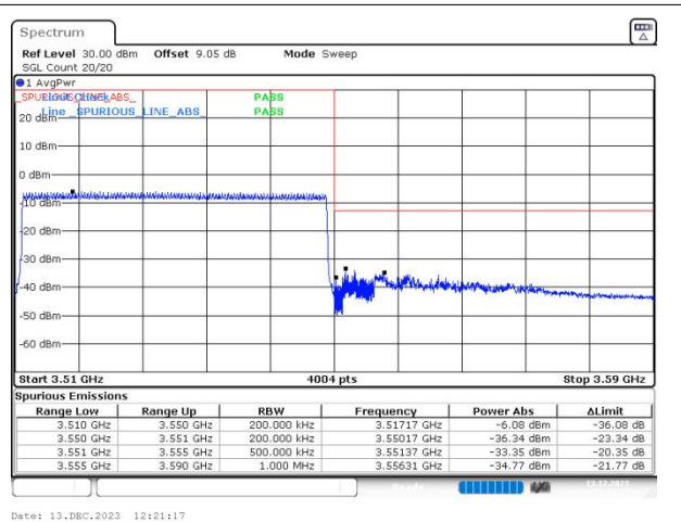
n77(3450-3550) SCS=30kHz CP_QPSK BW=40MHz HighChannel=635332 RB=106@0
