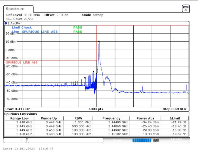
n77(3450-3550) SCS=30kHz DFT_16QAM BW=40MHz LowChannel=631334 RB=1@0
