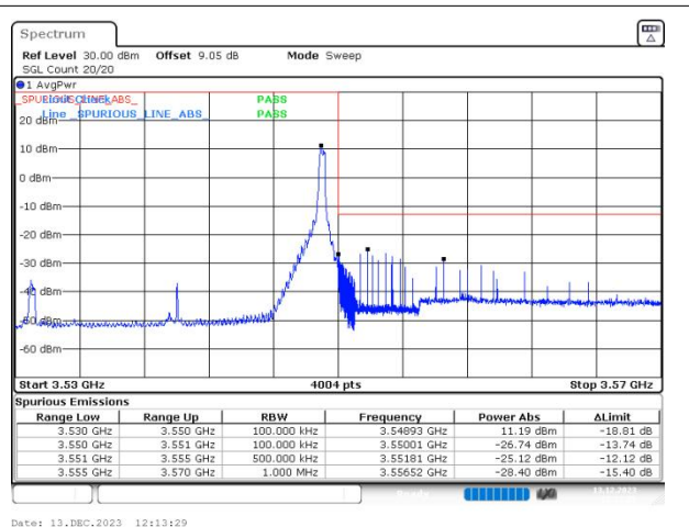
n77(3450-3550) SCS=30kHz DFT_16QAM BW=20MHz HighChannel=636000 RB=1@50
