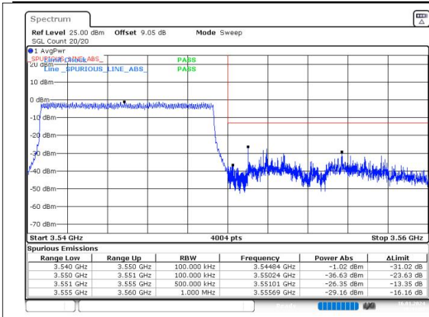
n77(3450-3550) SCS=30kHz DFT_64QAM BW=10MHz HighChannel=636332 RB=24@0
