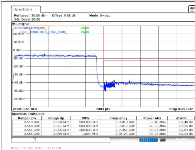
n77(3450-3550) SCS=30kHz DFT_64QAM BW=40MHz HighChannel=635332 RB=100@0
