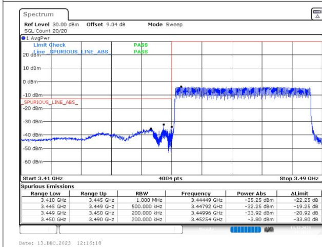
n77(3450-3550) SCS=30kHz DFT_16QAM BW=40MHz LowChannel=631334 RB=100@0
