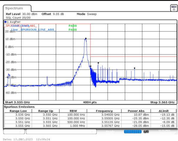
n77(3450-3550) SCS=30kHz DFT_16QAM BW=15MHz HighChannel=636166 RB=1@37
