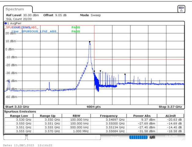
n77(3450-3550) SCS=30kHz DFT_256QAM BW=20MHz HighChannel=636000 RB=1@50
