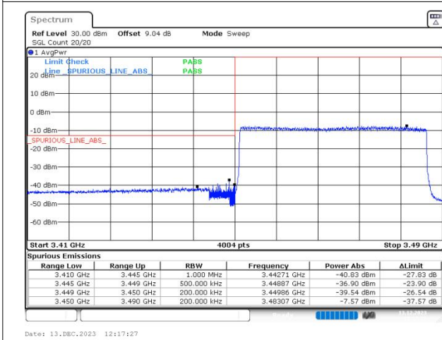
n77(3450-3550) SCS=30kHz DFT_256QAM BW=40MHz LowChannel=631334 RB=100@0
