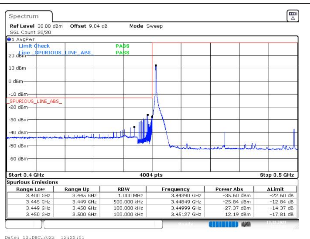
n77(3450-3550) SCS=30kHz DFT_BPSK BW=50MHz LowChannel=631668 RB=1@0
