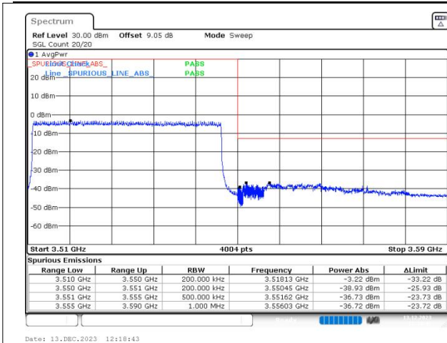
n77(3450-3550) SCS=30kHz DFT_BPSK BW=40MHz HighChannel=635332 RB=100@0
