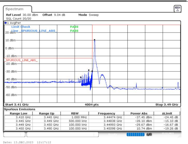
n77(3450-3550) SCS=30kHz DFT_64QAM BW=40MHz LowChannel=631334 RB=1@0
