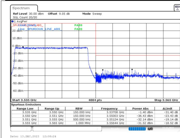
n77(3450-3550) SCS=30kHz DFT_QPSK BW=15MHz HighChannel=636166 RB=36@0
