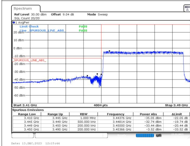
n77(3450-3550) SCS=30kHz DFT_QPSK BW=40MHz LowChannel=631334 RB=100@0
