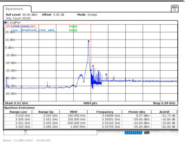
n77(3450-3550) SCS=30kHz DFT_256QAM BW=40MHz HighChannel=635332 RB=1@105
