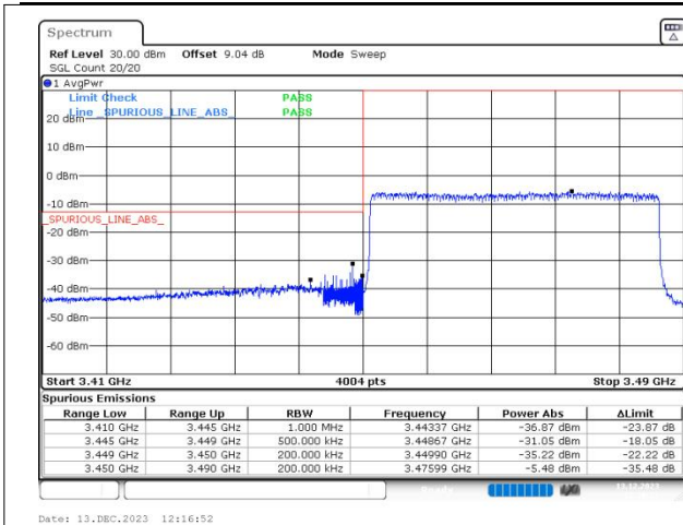
n77(3450-3550) SCS=30kHz DFT_64QAM BW=40MHz LowChannel=631334 RB=100@0
