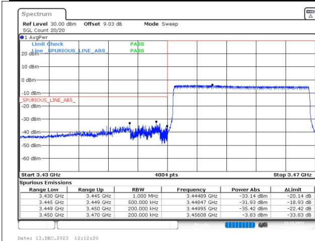
n77(3450-3550) SCS=30kHz CP_QPSK BW=20MHz LowChannel=630668 RB=51@0
