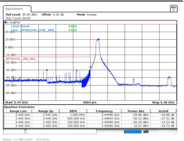
n77(3450-3550) SCS=30kHz DFT_64QAM BW=10MHz LowChannel=630334 RB=1@0
