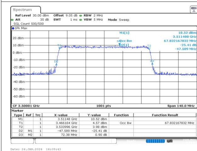
n77(3450-3550) SCS=30kHz CP_256QAM BW=70MHz Channel=633334 RB=189@0
