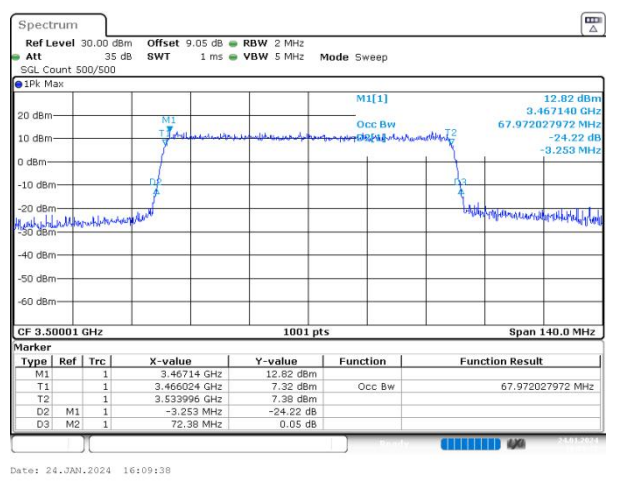
n77(3450-3550) SCS=30kHz CP_64QAM BW=70MHz Channel=633334 RB=189@0
