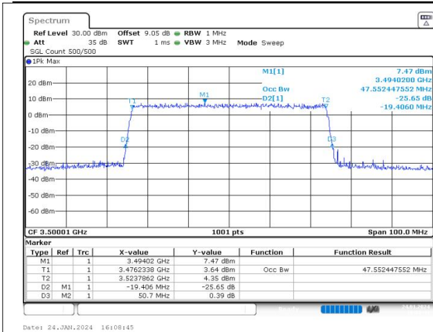
n77(3450-3550) SCS=30kHz CP_256QAM BW=50MHz Channel=633334 RB=133@0
