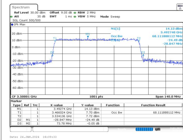
n77(3450-3550) SCS=30kHz CP_16QAM BW=70MHz Channel=633334 RB=189@0
