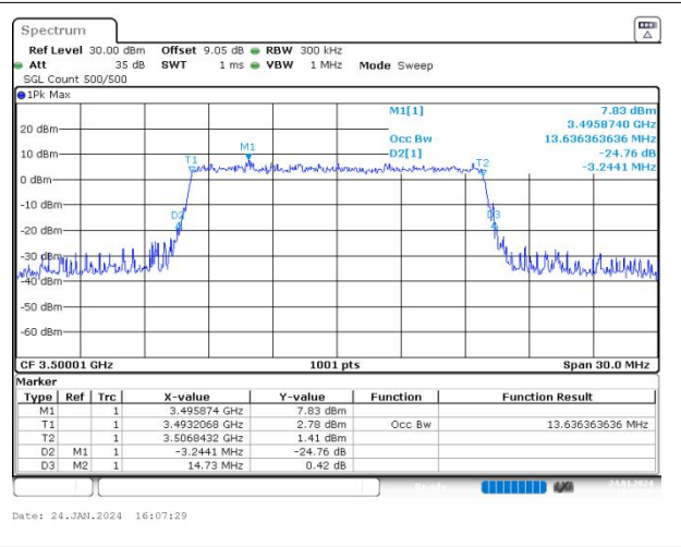
n77(3450-3550) SCS=30kHz CP_256QAM BW=15MHz Channel=633334 RB=38@0
