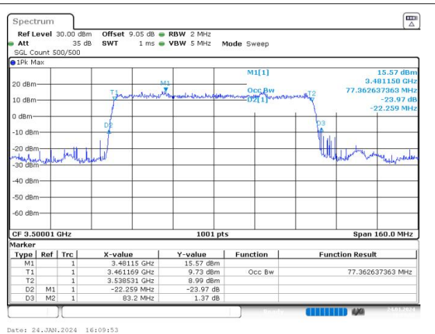
n77(3450-3550) SCS=30kHz DFT_BPSK BW=80MHz Channel=633334 RB=216@0
