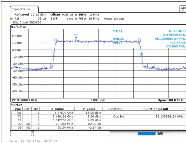
n77(3450-3550) SCS=30kHz DFT_BPSK BW=90MHz Channel=633334 RB=240@0
