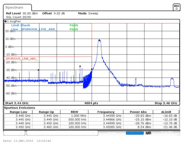
n77(3450-3550) SCS=30kHz DFT_256QAM BW=10MHz LowChannel=630334 RB=1@0
