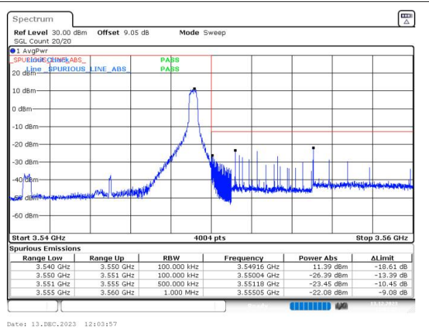
n77(3450-3550) SCS=30kHz DFT_16QAM BW=10MHz HighChannel=636332 RB=1@23
