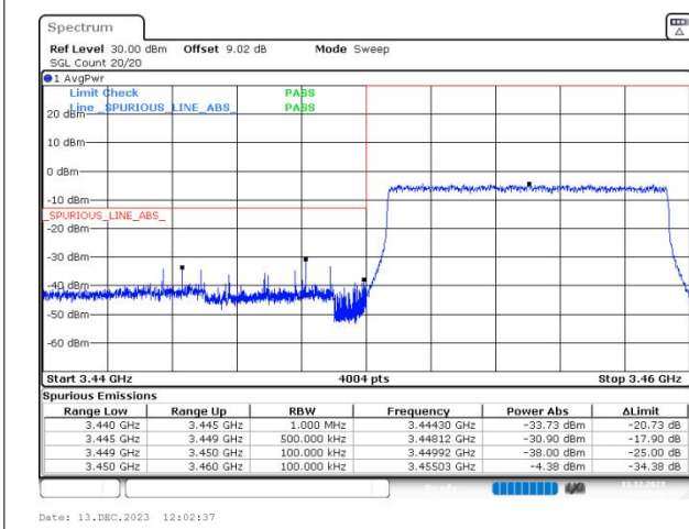
n77(3450-3550) SCS=30kHz DFT_256QAM BW=10MHz LowChannel=630334 RB=24@0
