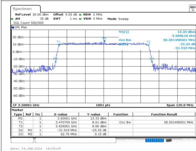
n77(3450-3550) SCS=30kHz CP_64QAM BW=60MHz Channel=633334 RB=162@0
