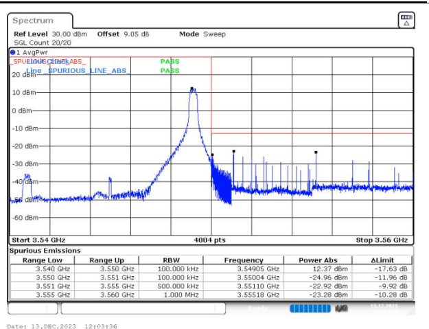
n77(3450-3550) SCS=30kHz DFT_QPSK BW=10MHz HighChannel=636332 RB=1@23
