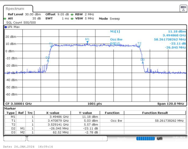
n77(3450-3550) SCS=30kHz CP_256QAM BW=60MHz Channel=633334 RB=162@0
