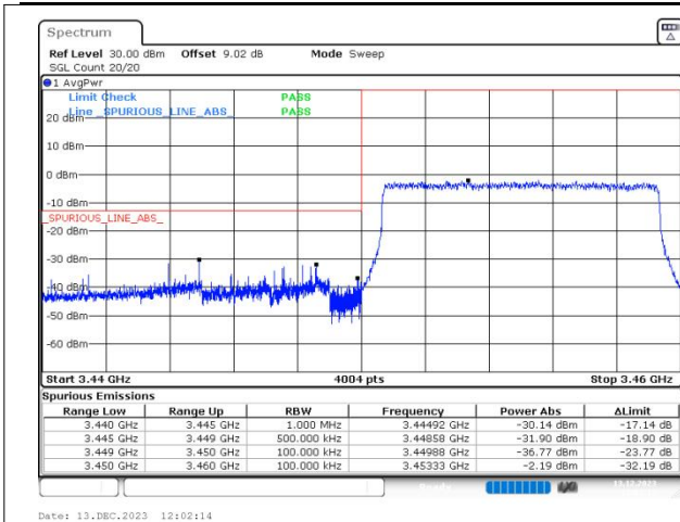
n77(3450-3550) SCS=30kHz DFT_64QAM BW=10MHz LowChannel=630334 RB=24@0
