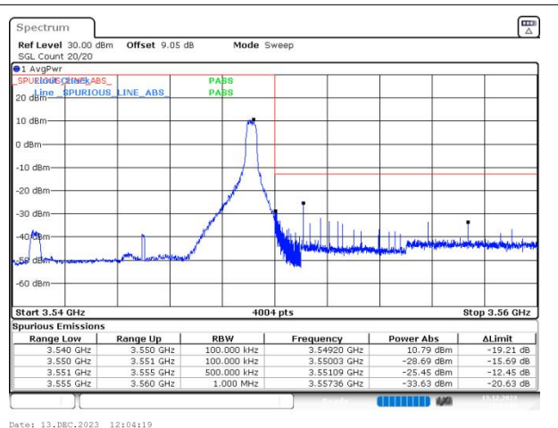
n77(3450-3550) SCS=30kHz DFT_64QAM BW=10MHz HighChannel=636332 RB=1@23
