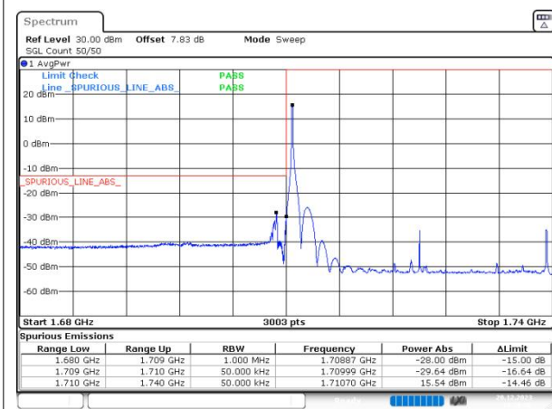
n66 SCS=15kHz DFT_64QAM BW=30MHz LowChannel=345000 RB=1@0
