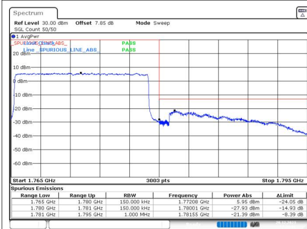
n66 SCS=15kHz DFT_BPSK BW=15MHz HighChannel=354500 RB=75@0
