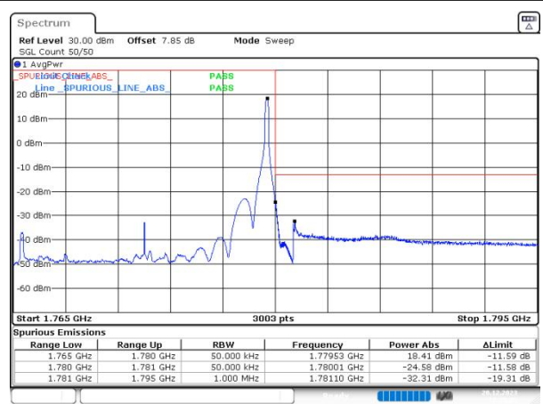
n66 SCS=15kHz DFT_QPSK BW=15MHz HighChannel=354500 RB=1@78
