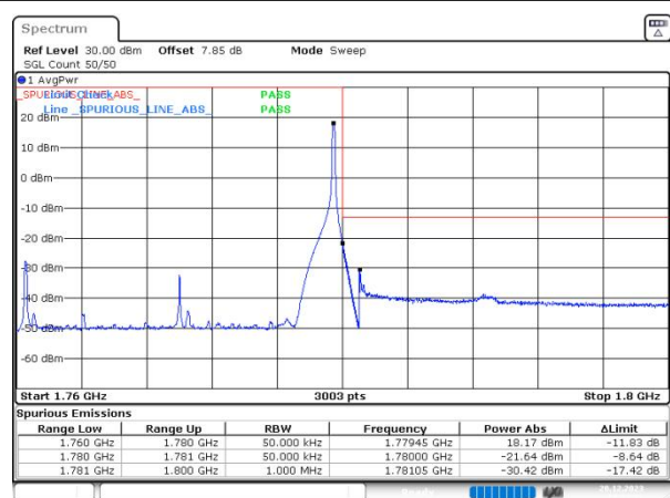
n66 SCS=15kHz DFT_16QAM BW=20MHz HighChannel=354000 RB=1@105
