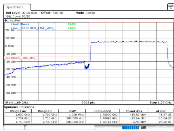
n66 SCS=15kHz DFT_BPSK BW=20MHz LowChannel=344000 RB=100@0
