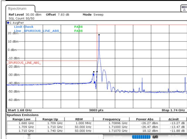
n66 SCS=15kHz DFT_16QAM BW=30MHz LowChannel=345000 RB=1@0
