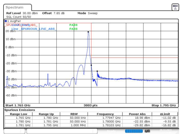
n66 SCS=15kHz DFT_BPSK BW=15MHz HighChannel=354500 RB=1@78
