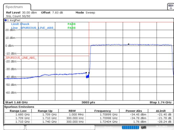
n66 SCS=15kHz DFT_64QAM BW=30MHz LowChannel=345000 RB=160@0
