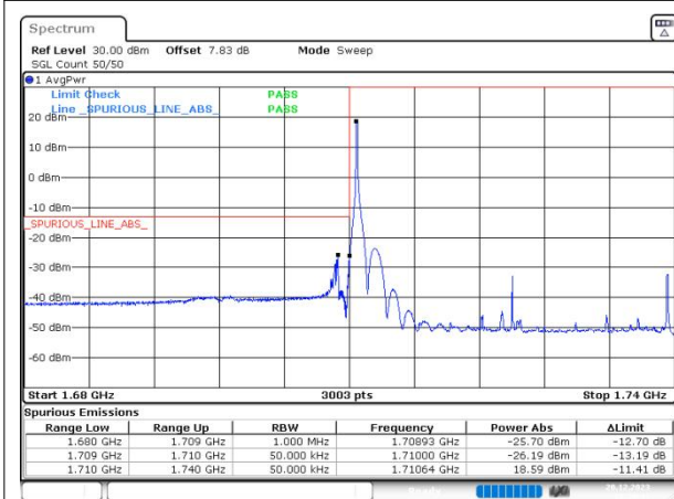
n66 SCS=15kHz DFT_BPSK BW=30MHz LowChannel=345000 RB=1@0
