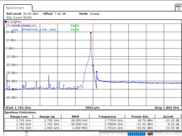
n66 SCS=15kHz DFT_BPSK BW=25MHz HighChannel=353500 RB=1@132
