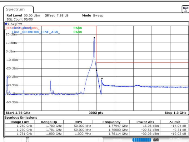
n66 SCS=15kHz DFT_256QAM BW=20MHz HighChannel=354000 RB=1@105
