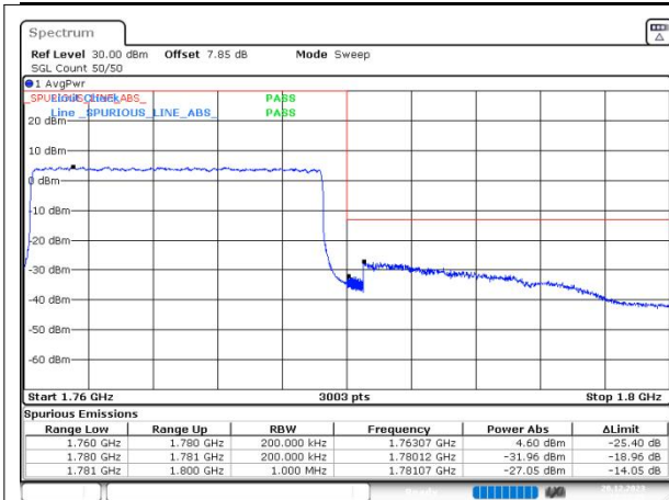
n66 SCS=15kHz DFT_64QAM BW=20MHz HighChannel=354000 RB=100@0
