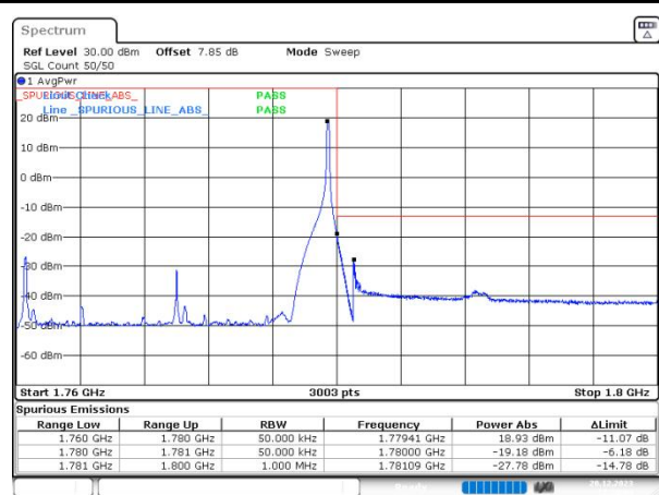
n66 SCS=15kHz DFT_QPSK BW=20MHz HighChannel=354000 RB=1@105
