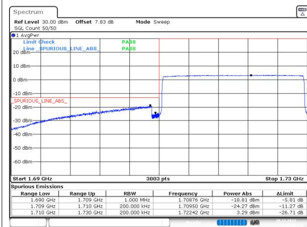
n66 SCS=15kHz DFT_256QAM BW=20MHz LowChannel=344000 RB=1@0
