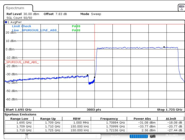
n66 SCS=15kHz DFT_64QAM BW=15MHz LowChannel=343500 RB=75@0
