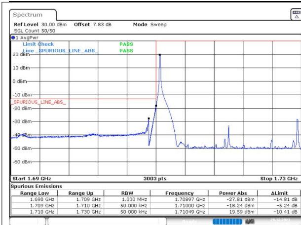
n66 SCS=15kHz DFT_BPSK BW=20MHz LowChannel=344000 RB=1@0
