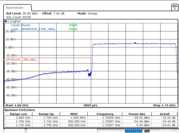
n66 SCS=15kHz DFT_BPSK BW=30MHz LowChannel=345000 RB=160@0
