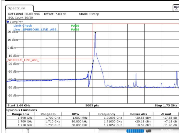
n66 SCS=15kHz DFT_64QAM BW=20MHz LowChannel=344000 RB=1@0
