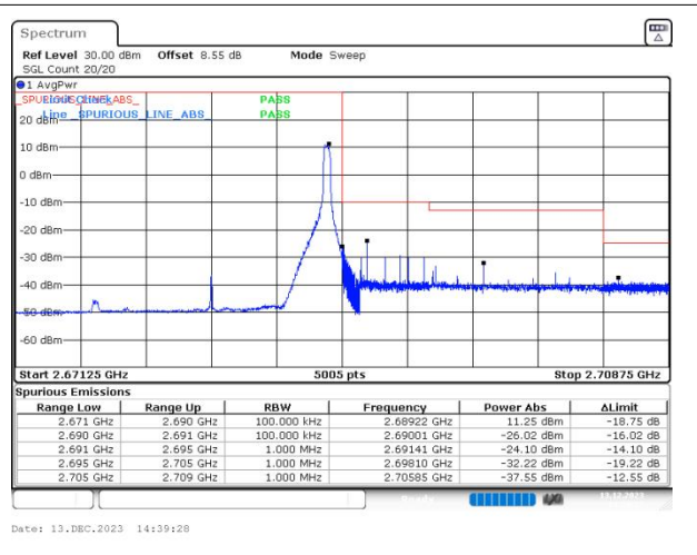
n41 SCS=30kHz DFT_64QAM BW=15MHz HighChannel=536496 RB=1@37
