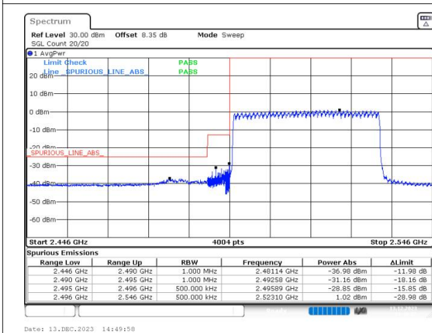
n41 SCS=30kHz DFT_BPSK BW=40MHz LowChannel=503202 RB=100@0
