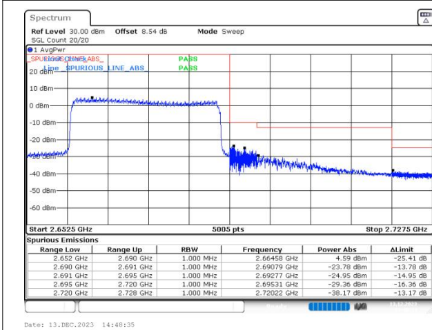
n41 SCS=30kHz DFT_16QAM BW=30MHz HighChannel=534996 RB=75@0
