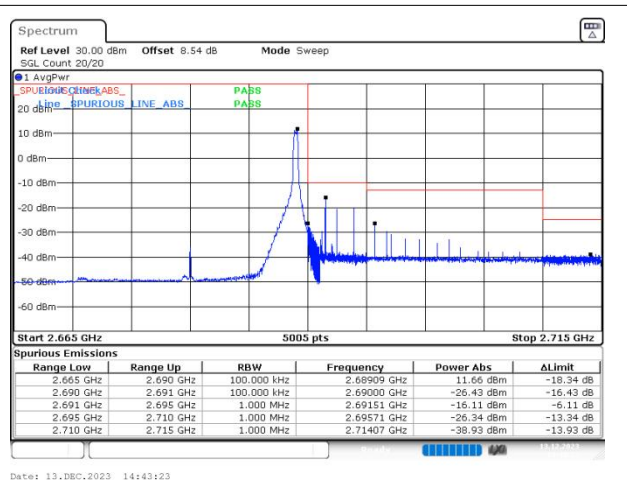
n41 SCS=30kHz DFT_16QAM BW=20MHz HighChannel=535998 RB=1@50
