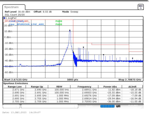
n41 SCS=30kHz DFT_16QAM BW=15MHz HighChannel=536496 RB=1@37
