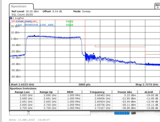
n41 SCS=30kHz DFT_QPSK BW=30MHz HighChannel=534996 RB=75@0
