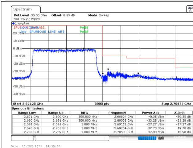
n41 SCS=30kHz DFT_256QAM BW=15MHz HighChannel=536496 RB=36@0
