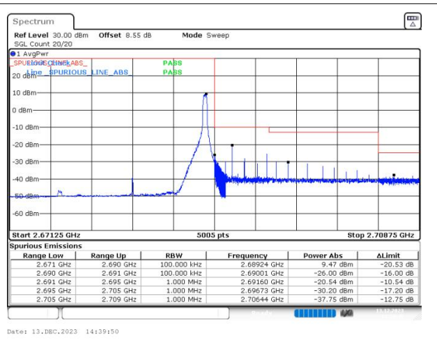
n41 SCS=30kHz DFT_256QAM BW=15MHz HighChannel=536496 RB=1@37
