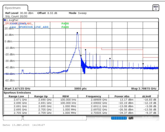
n41 SCS=30kHz DFT_BPSK BW=15MHz HighChannel=536496 RB=1@37
