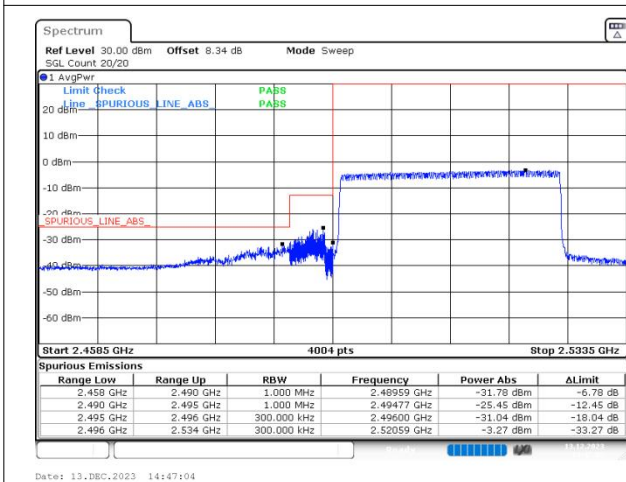
n41 SCS=30kHz CP_QPSK BW=30MHz LowChannel=502200 RB=78@0
