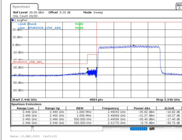
n41 SCS=30kHz DFT_16QAM BW=40MHz LowChannel=503202 RB=100@0
