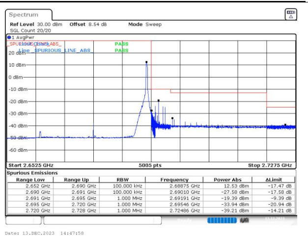
n41 SCS=30kHz DFT_QPSK BW=30MHz HighChannel=534996 RB=1@77
