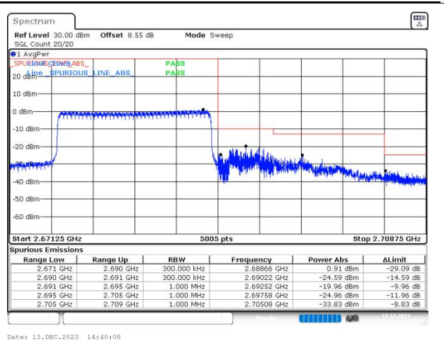
n41 SCS=30kHz CP_QPSK BW=15MHz HighChannel=536496 RB=38@0
