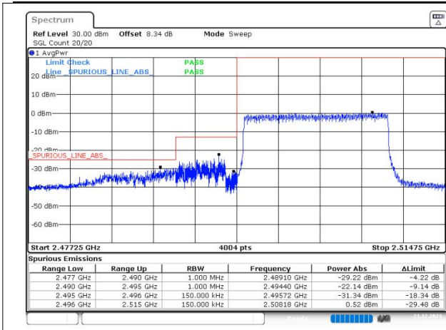
n41 SCS=30kHz DFT_QPSK BW=15MHz LowChannel=500700 RB=36@0
