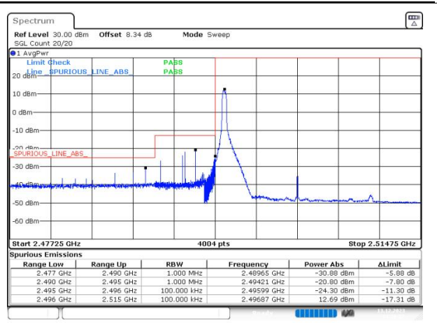
n41 SCS=30kHz DFT_QPSK BW=15MHz LowChannel=500700 RB=1@0
