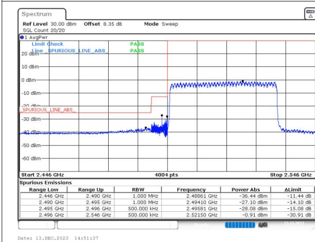
n41 SCS=30kHz DFT_64QAM BW=40MHz LowChannel=503202 RB=100@0
