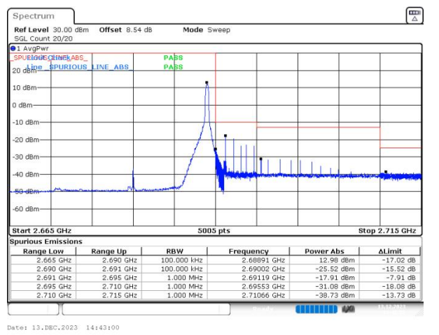
n41 SCS=30kHz DFT_QPSK BW=20MHz HighChannel=535998 RB=1@50
