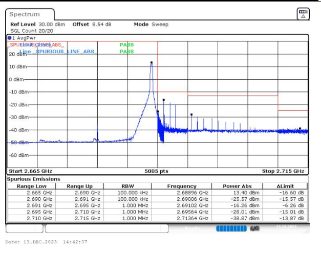
n41 SCS=30kHz DFT_BPSK BW=20MHz HighChannel=535998 RB=1@50
