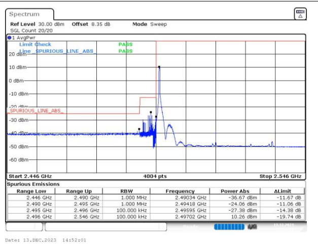
n41 SCS=30kHz DFT_64QAM BW=40MHz LowChannel=503202 RB=1@0
