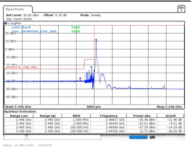
n41 SCS=30kHz DFT_QPSK BW=40MHz LowChannel=503202 RB=1@0
