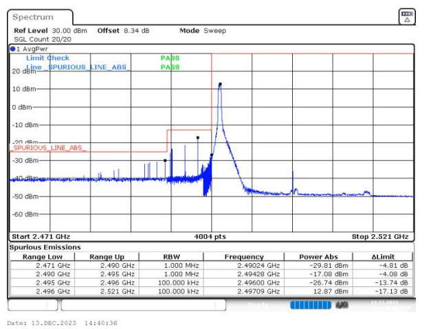
n41 SCS=30kHz DFT_BPSK BW=20MHz LowChannel=501204 RB=1@0
