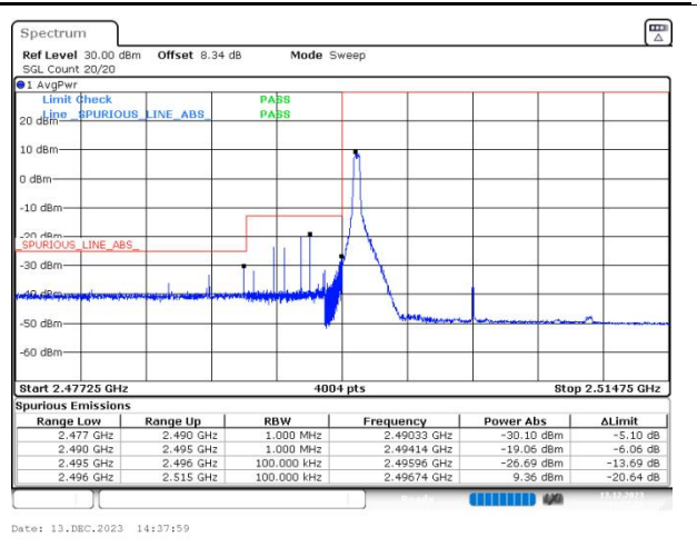
n41 SCS=30kHz DFT_256QAM BW=15MHz LowChannel=500700 RB=1@0
