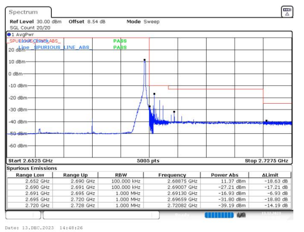
n41 SCS=30kHz DFT_16QAM BW=30MHz HighChannel=534996 RB=1@77
