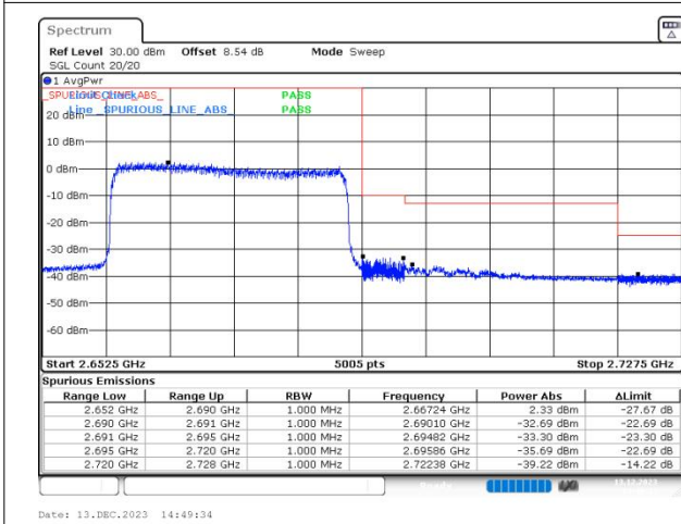
n41 SCS=30kHz DFT_256QAM BW=30MHz HighChannel=534996 RB=75@0
