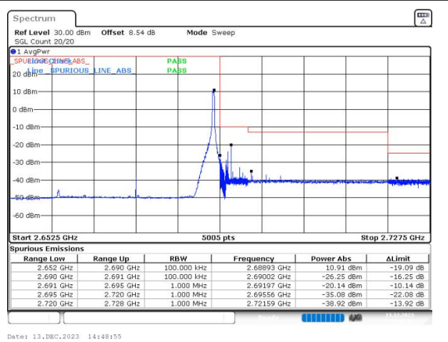
n41 SCS=30kHz DFT_64QAM BW=30MHz HighChannel=534996 RB=1@77
