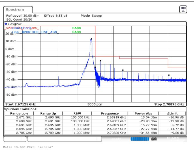
n41 SCS=30kHz DFT_QPSK BW=15MHz HighChannel=536496 RB=1@37
