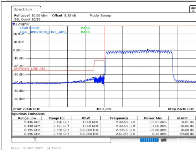
n41 SCS=30kHz DFT_QPSK BW=40MHz LowChannel=503202 RB=100@0
