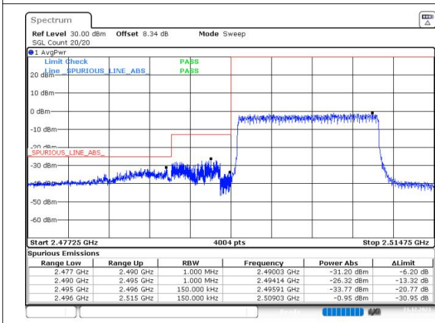
n41 SCS=30kHz DFT_16QAM BW=15MHz LowChannel=500700 RB=36@0
