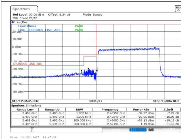
n41 SCS=30kHz DFT_16QAM BW=30MHz LowChannel=502200 RB=75@0
