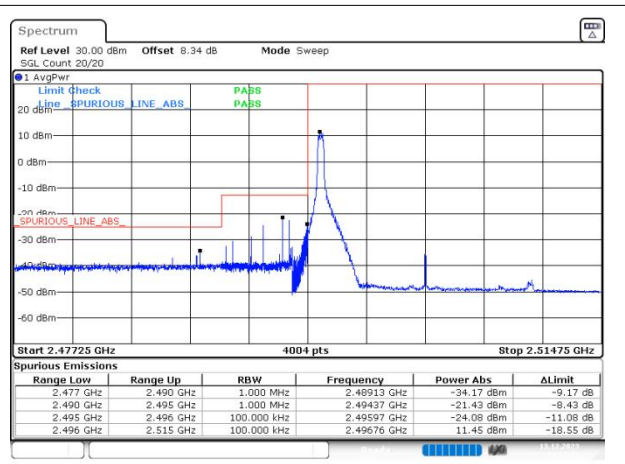
n41 SCS=30kHz DFT_16QAM BW=15MHz LowChannel=500700 RB=1@0
