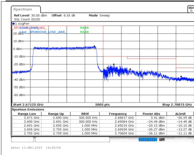
n41 SCS=30kHz DFT_QPSK BW=15MHz HighChannel=536496 RB=36@0
