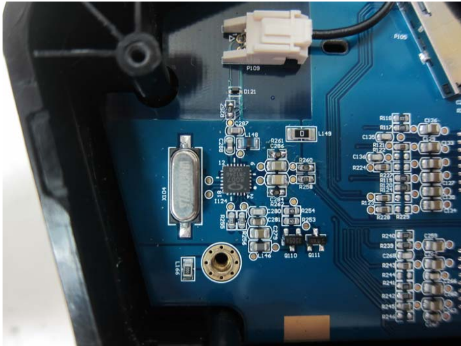
Front View of the EUT's FM Transmitter PCB
