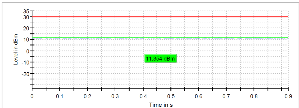
Gated Trace
