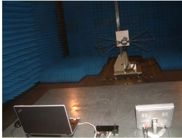
RE Below 1GHz-2
