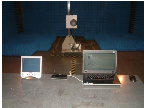
RE Above 1GHz-1
