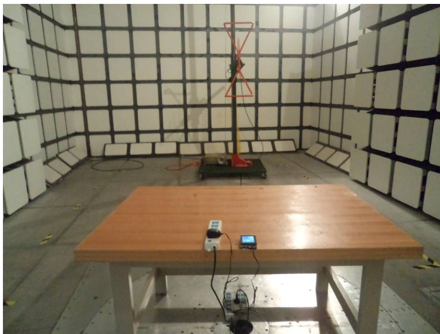
Radiated Emissions - Rear View (Test mode 2)
