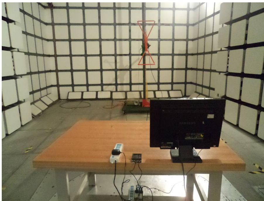
Radiated Emissions - Rear View (Test mode 3)
