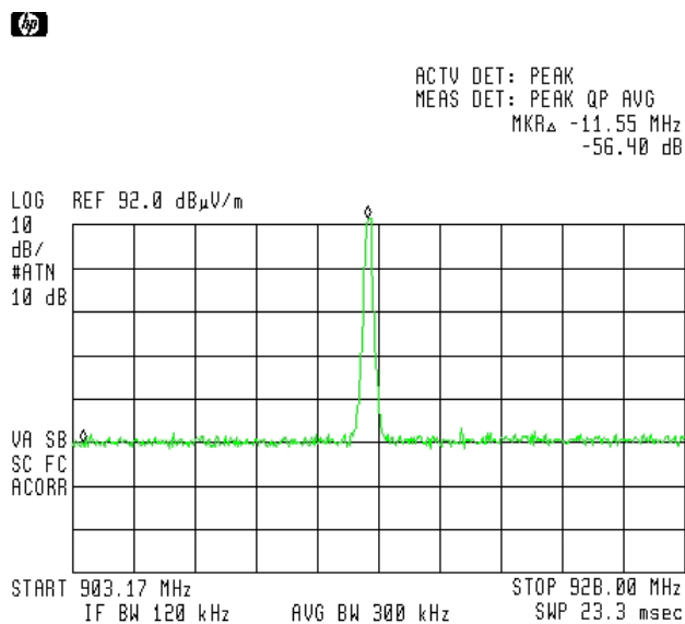
Figure 9. Band Edge Attenuation
