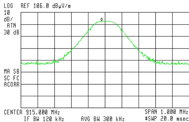
Figure 6. 915.00 MHz Antenna Polarization Vertical
