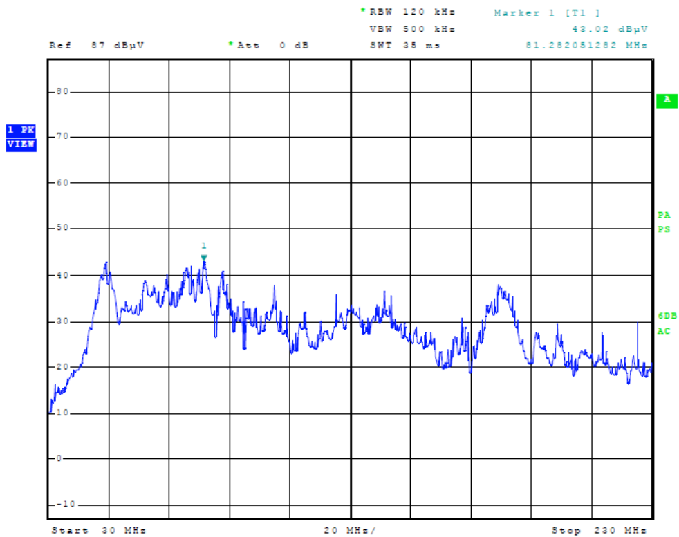
Figure 12 General Radiated Emissions taken at 1 meter in screen room (POE 2)
