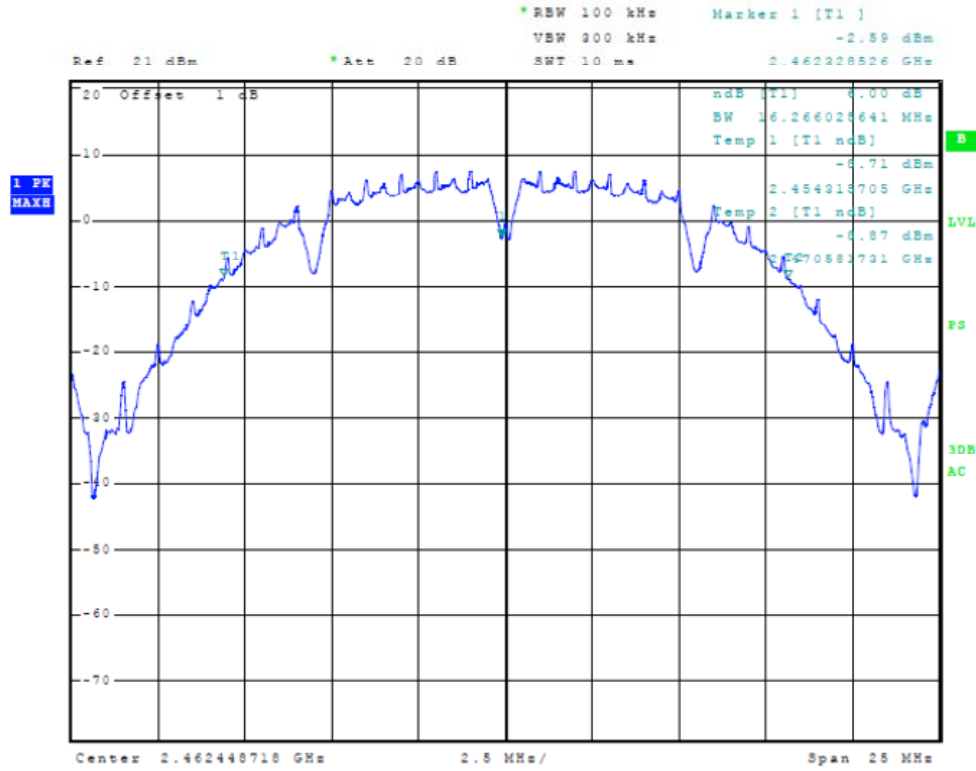
Figure 27 Plot of 6dB Band width (20 MHz Mode, CCK 2462 MHz)
