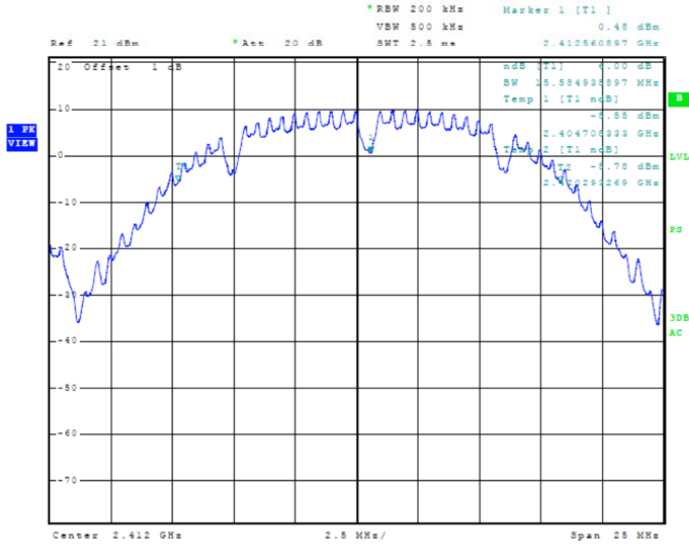
Figure 25 Plot of 6dB Band width (20 MHz Mode, CCK 2412 MHz)
