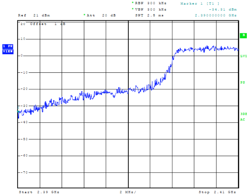
Figure 45 Plot of Band Edge Compliance at Antenna port (20 OFDM MHz)
