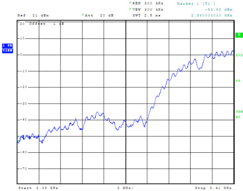
Figure 43 Plot of Band Edge Compliance at Antenna port (20 CCK MHz)
