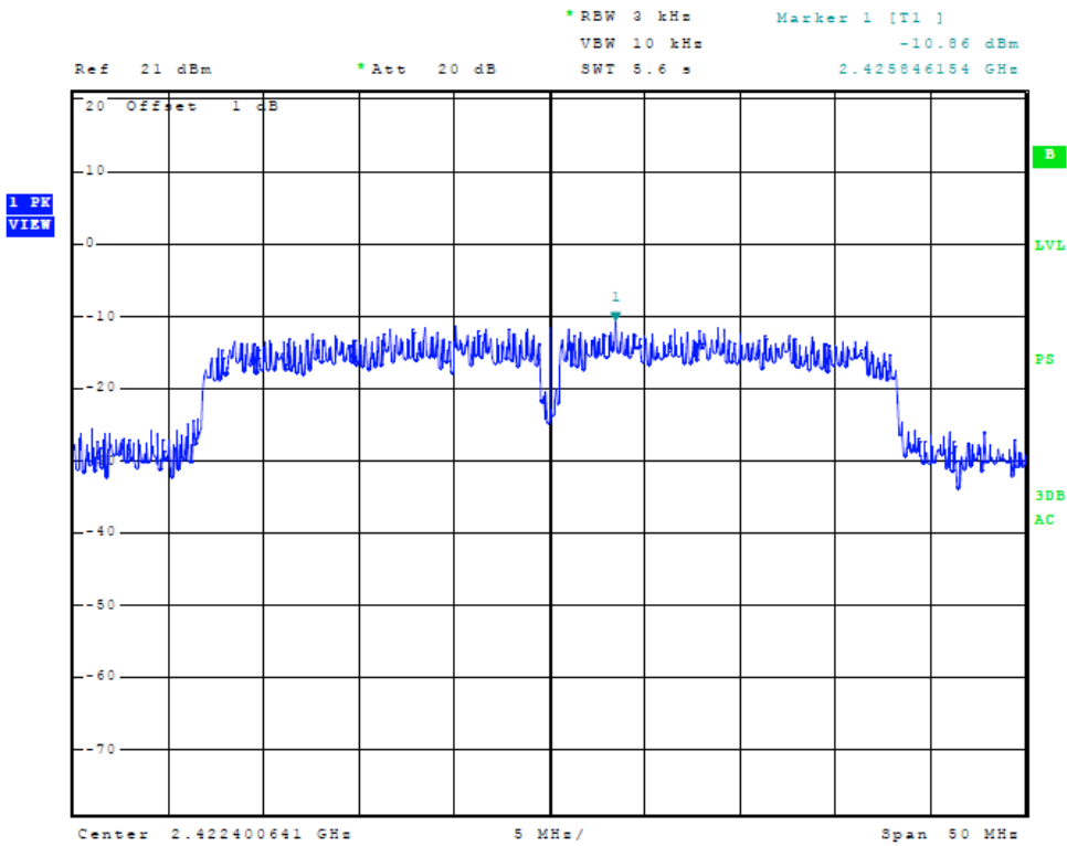
Figure 40 Plot of Power Spectral Density (40 MHz Mode, 2422 MHz)
