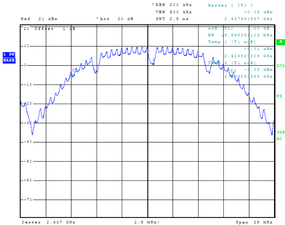
Figure 26 Plot of 6dB Band width (20 MHz Mode, CCK 2437 MHz)
