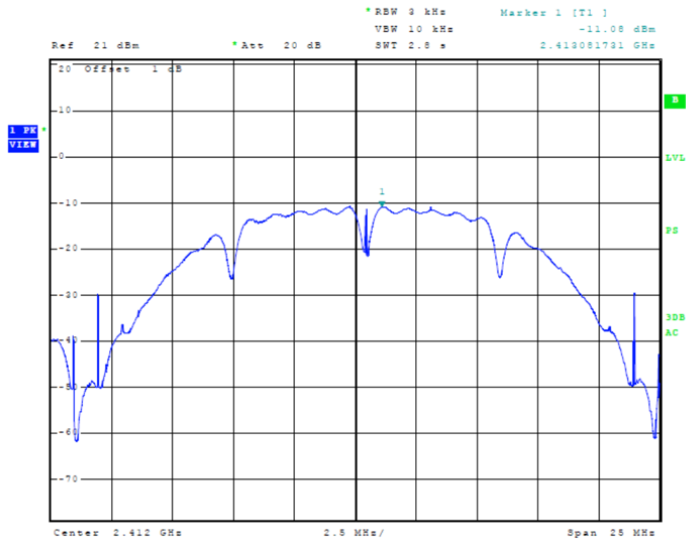
Figure 34 Plot of Power Spectral Density (20 MHz Mode, CCK 2412 MHz)
