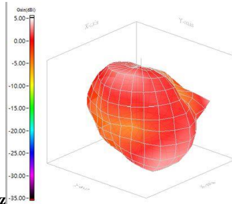
2.45GHz
