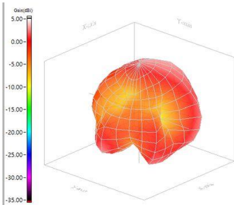
5.785GHz
