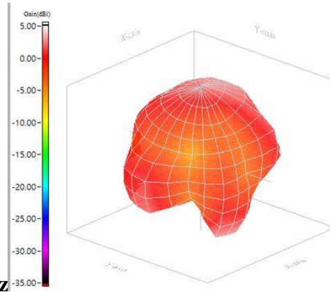
5.47GHz
