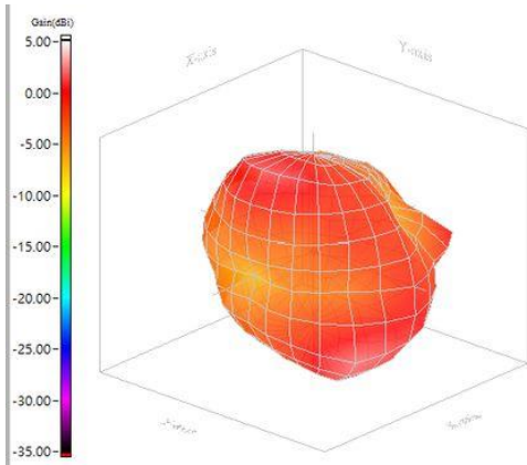
2.4GHz
