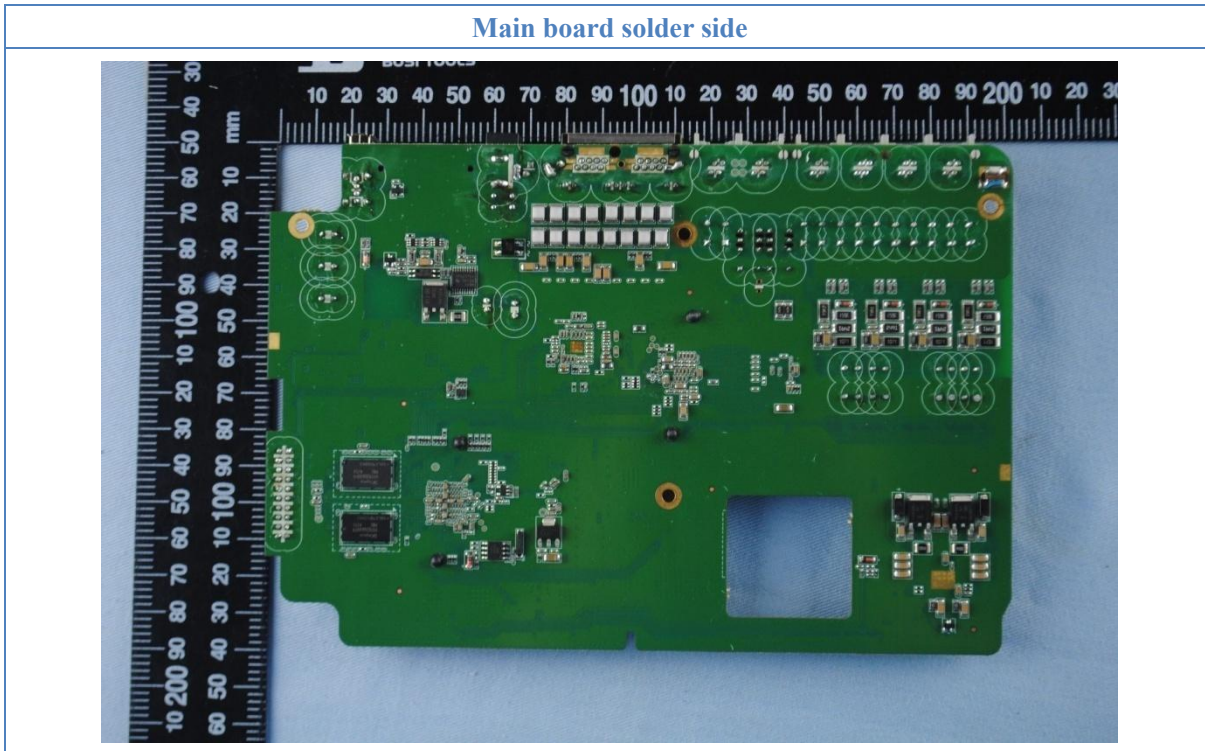
UCM6202 EUT top view
