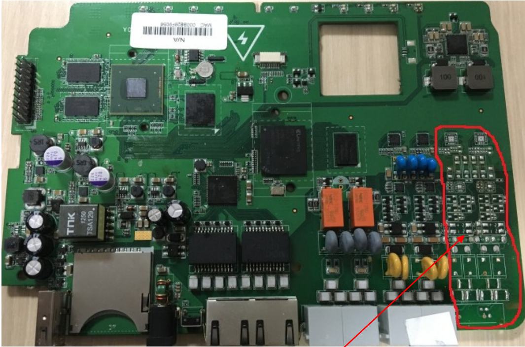
New main board top side photo
