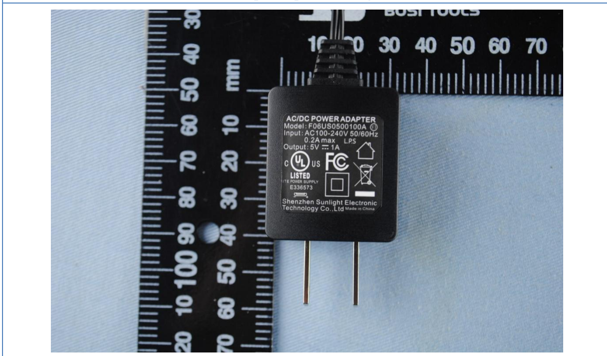
Adapter top view sunlight
