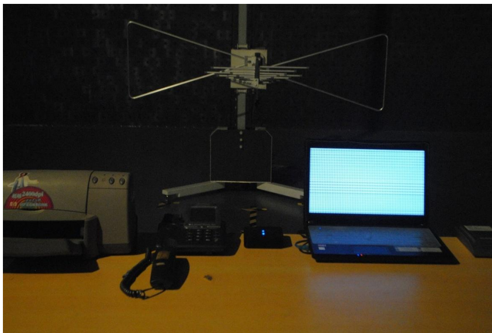
Radiated Emission test view (From 30MHz to 1GHz)
