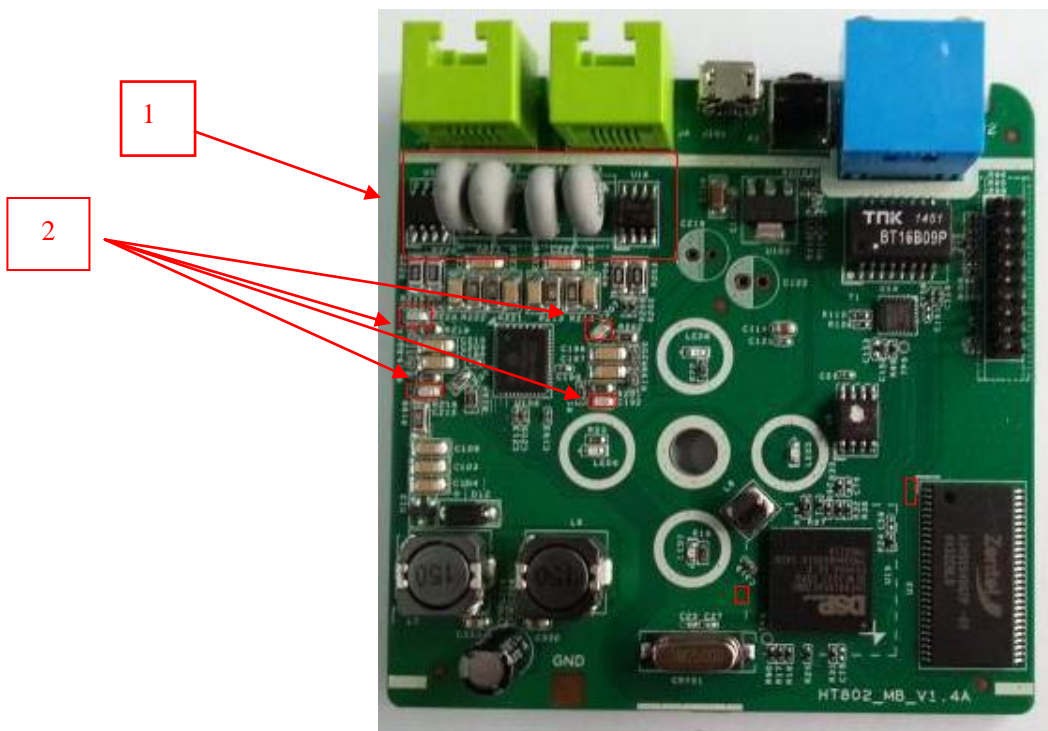
New PCB Layout view
